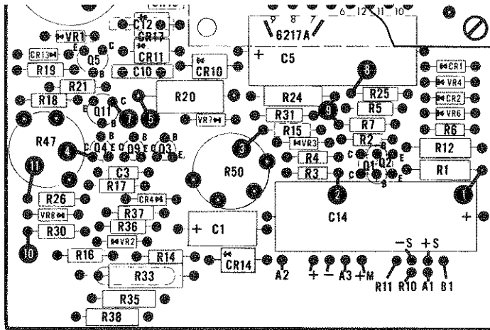
Figure A-1. Model 6217A, Component Location Diagram
