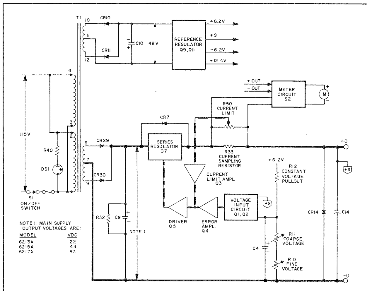
Figure 4-1. Simplified Schematic
