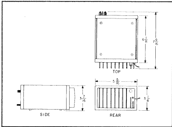
Figure 2-1. Outline Diagram
