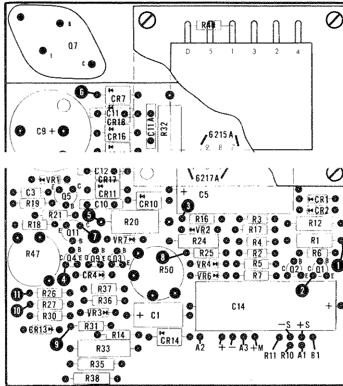
Figure A-2. Model 6217A, Component Location Diagram
