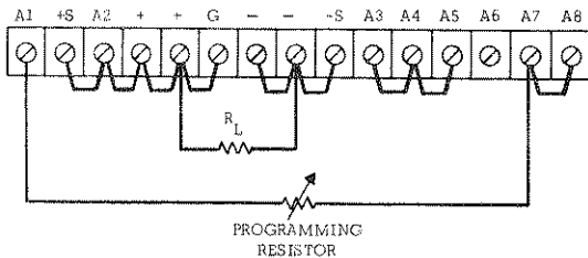
Figure 3-5. Remote Resistance Programming (Constant Current)
