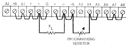
Figure 3-3. Remote Resistance Programming (Constant Voltage)
