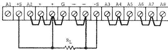
Figure 3-7. Remote Sensing
