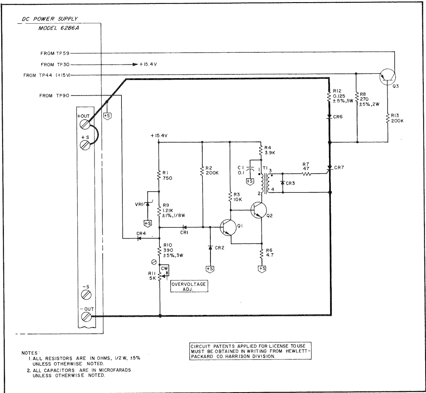
Figure A-1. Model 6286A Overvoltage Protection Crowbar
