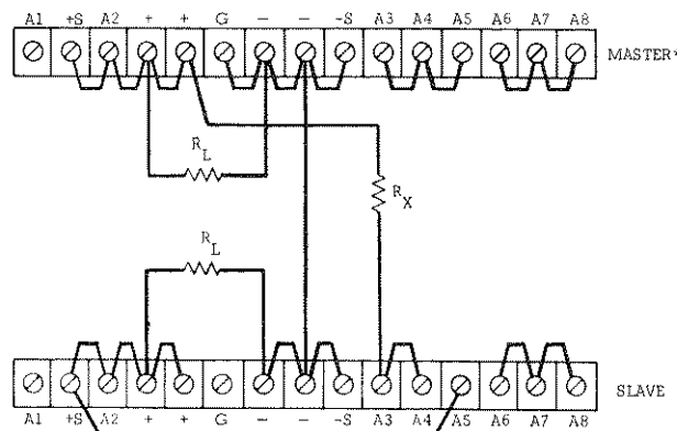
Figure 3-12. Auto-Tracking, Two Units
