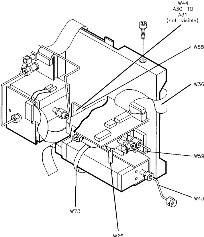
Figure 9-3. Cables (5 of 19)
