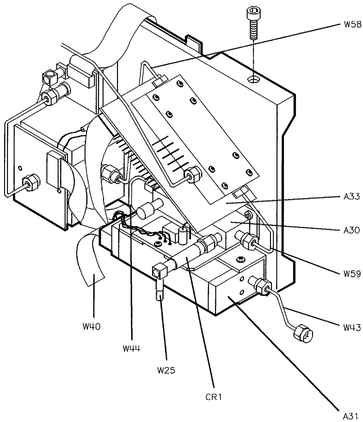
Figure 9-3. Cables (13 of 19)
