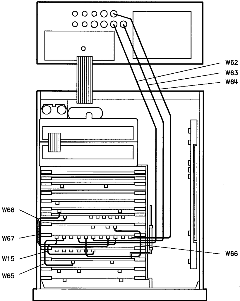
Figure 9-3. Cables (3 of 19)
