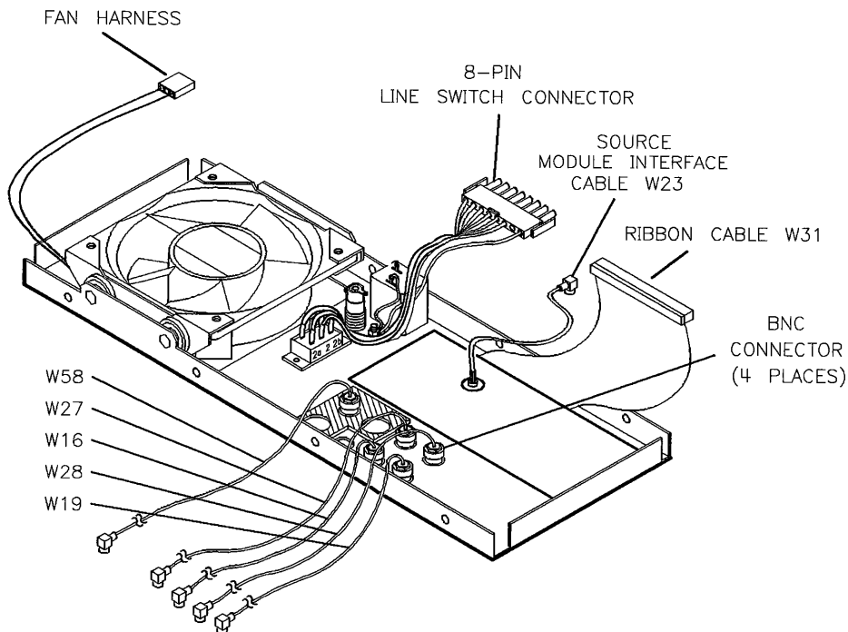
Figure 7-58. Rear Panel Cable Locations
