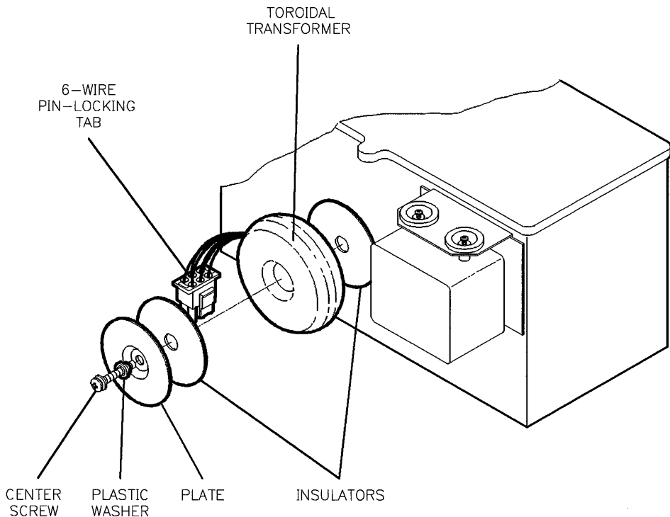
Figure 7-24. Transformer Removal
