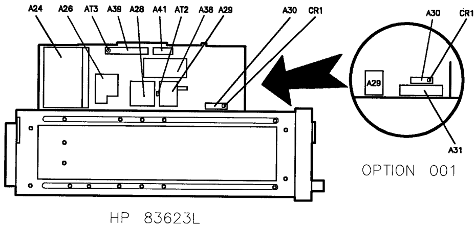
Figure 9-2. Major Assemblies (4 of 5)
