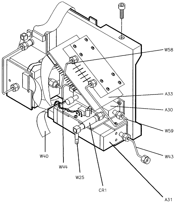
Figure 9-3. Cables (15 of 19)
