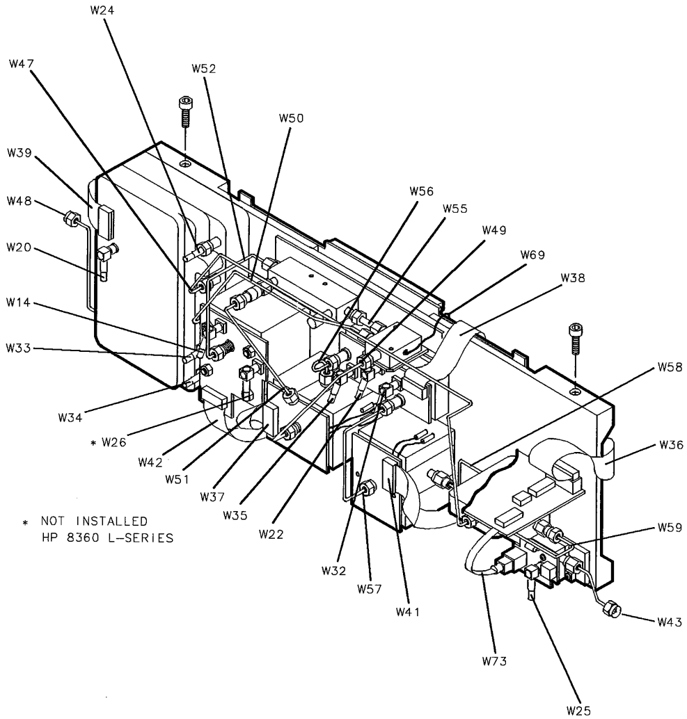
Figure 9-3. Cables (4 of 19)
