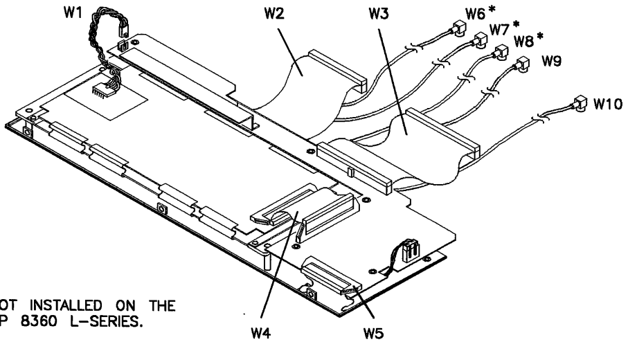
Figure 9-3. Cables (1 of 19)
