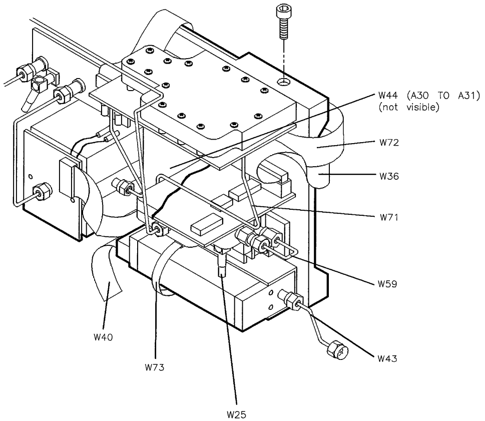
Figure 9-3. Cables (7 of 19)
