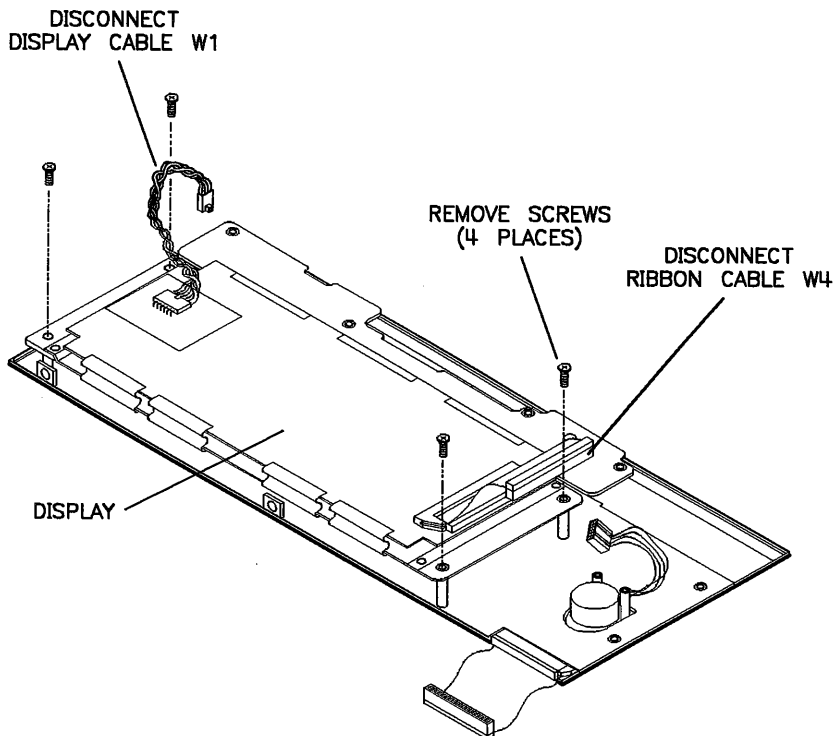
Figure 7-7. Display Removal
