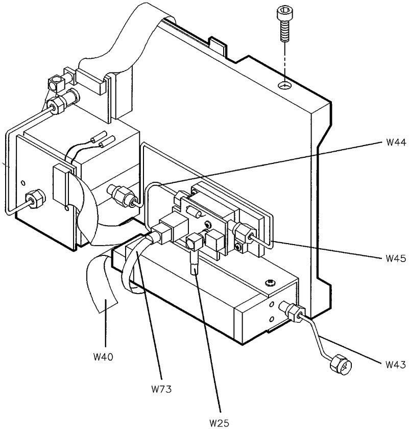
Figure 9-3. Cables (9 of 19)
