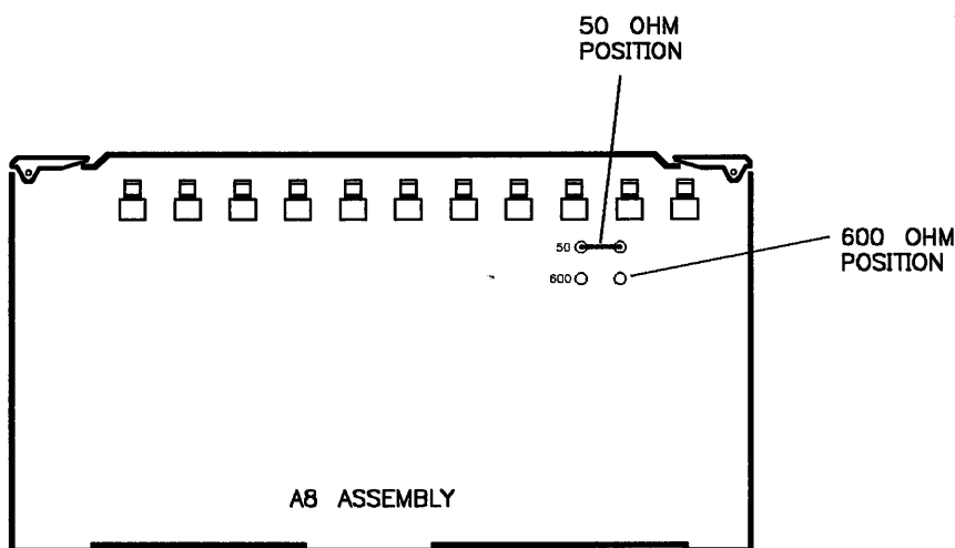
Figure 3-38. A8 Jumper Locations
