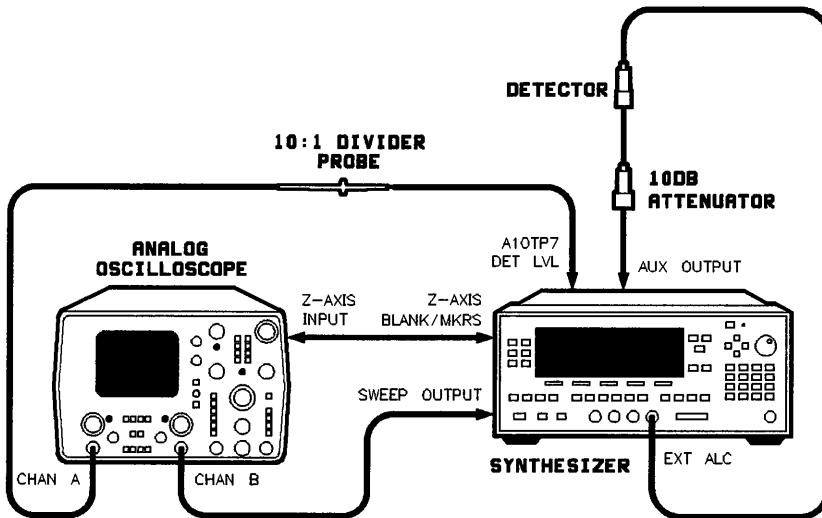
Figure 3-14. Amplifier/Multiplier Adjustments Setup
