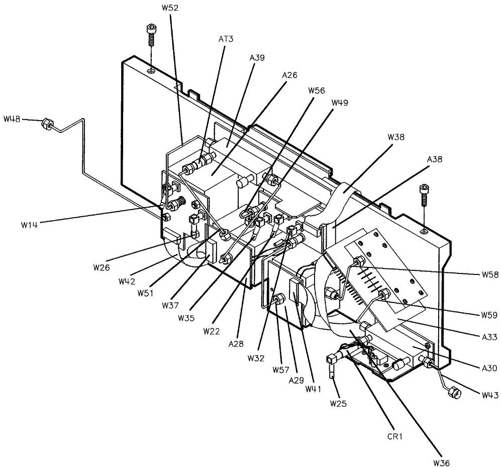
Figure 9-3. Cables (14 of 19)
