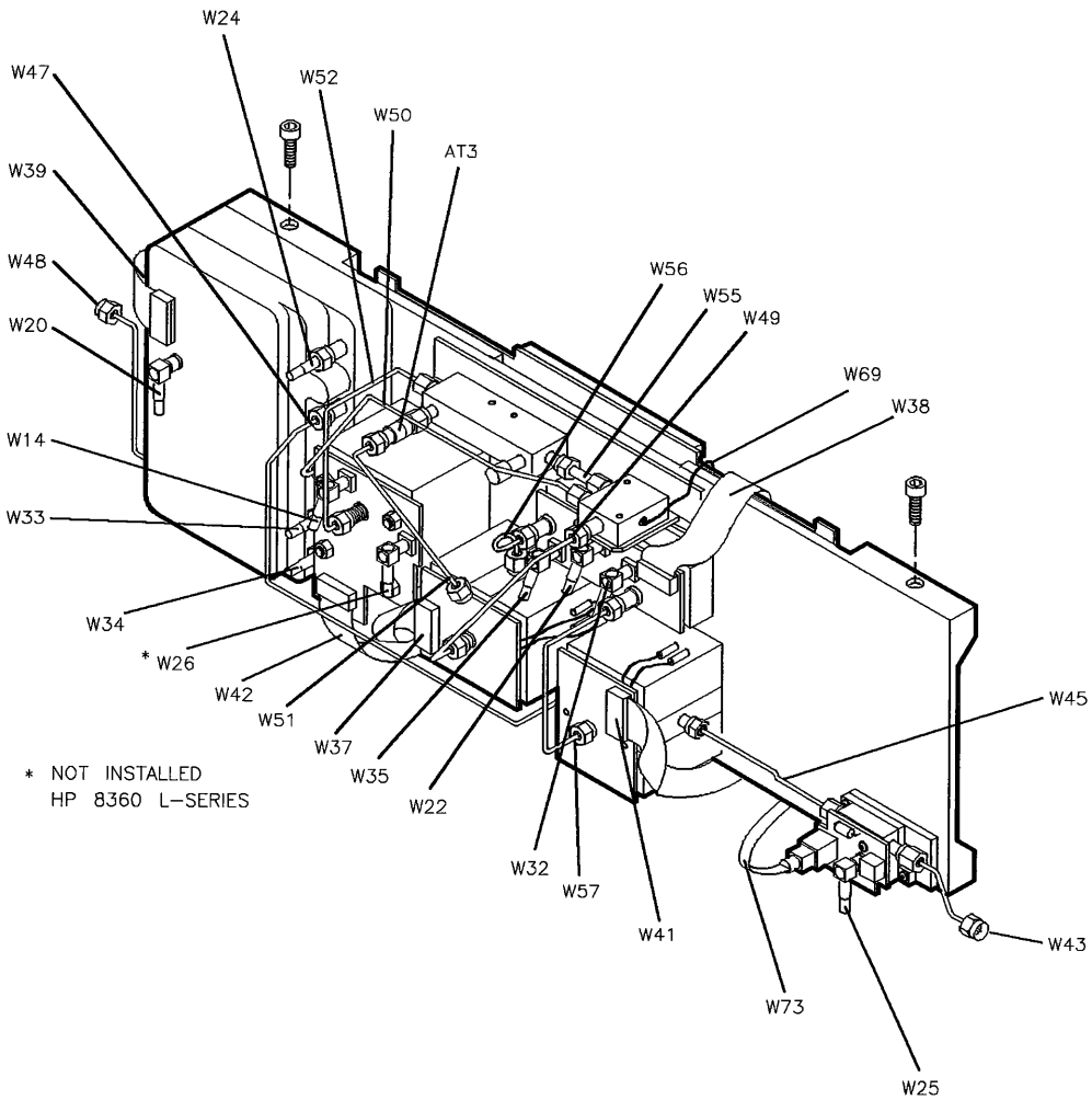
Figure 9-3. Cables (8 of 19)
