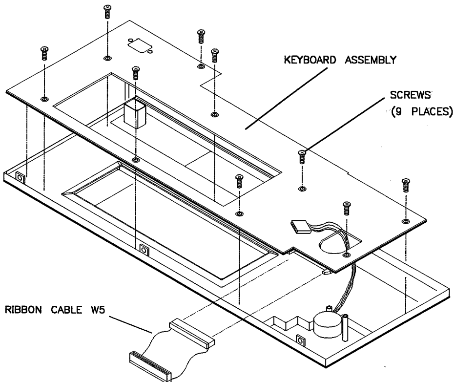
Figure 7-12. Keyboard Assembly Removal
