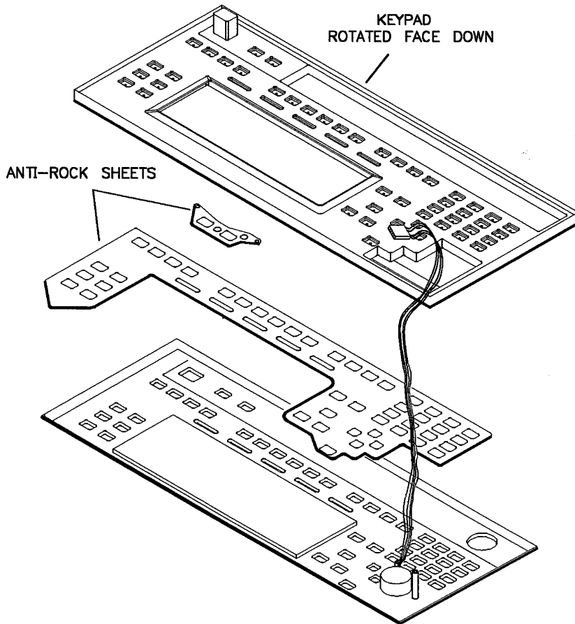
Figure 7-15. Keyboard Reassembly
