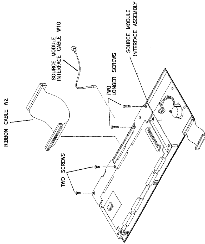
Figure 7-8. Source Module Interface Removal
