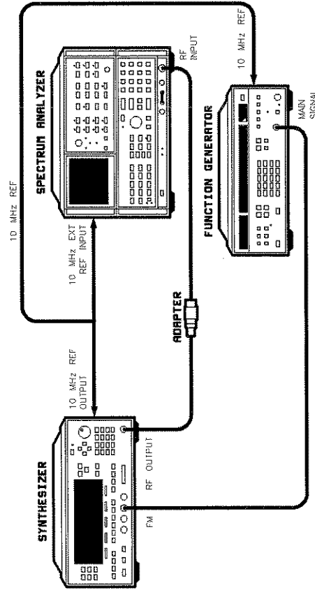
Figure 2-28. FM Accuracy Test Setup
