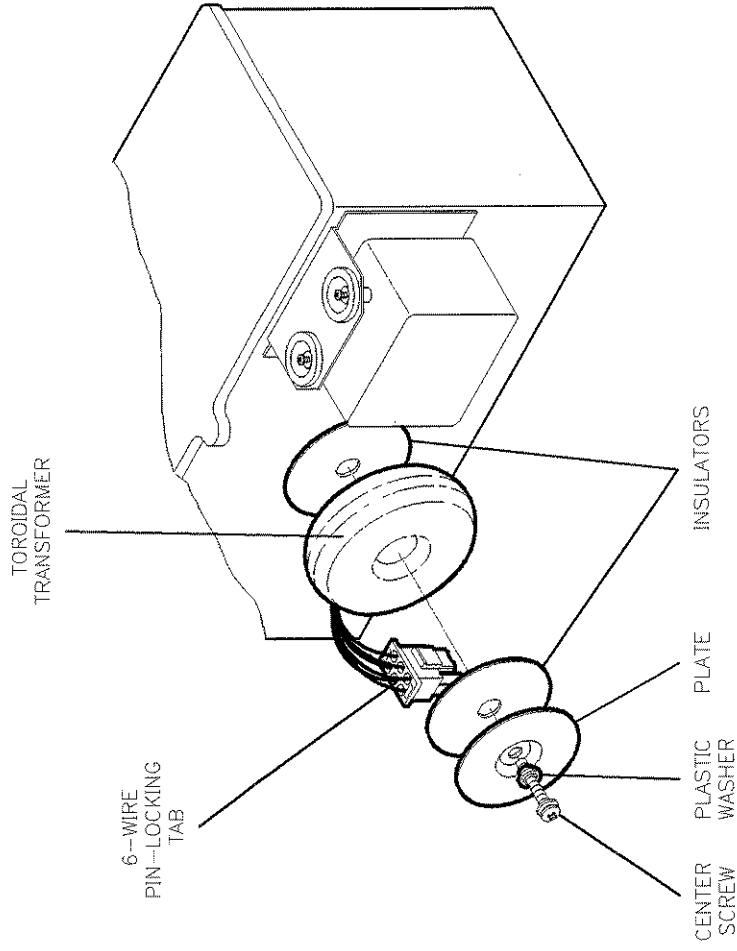
Figure 7-24. Transformer Removal
