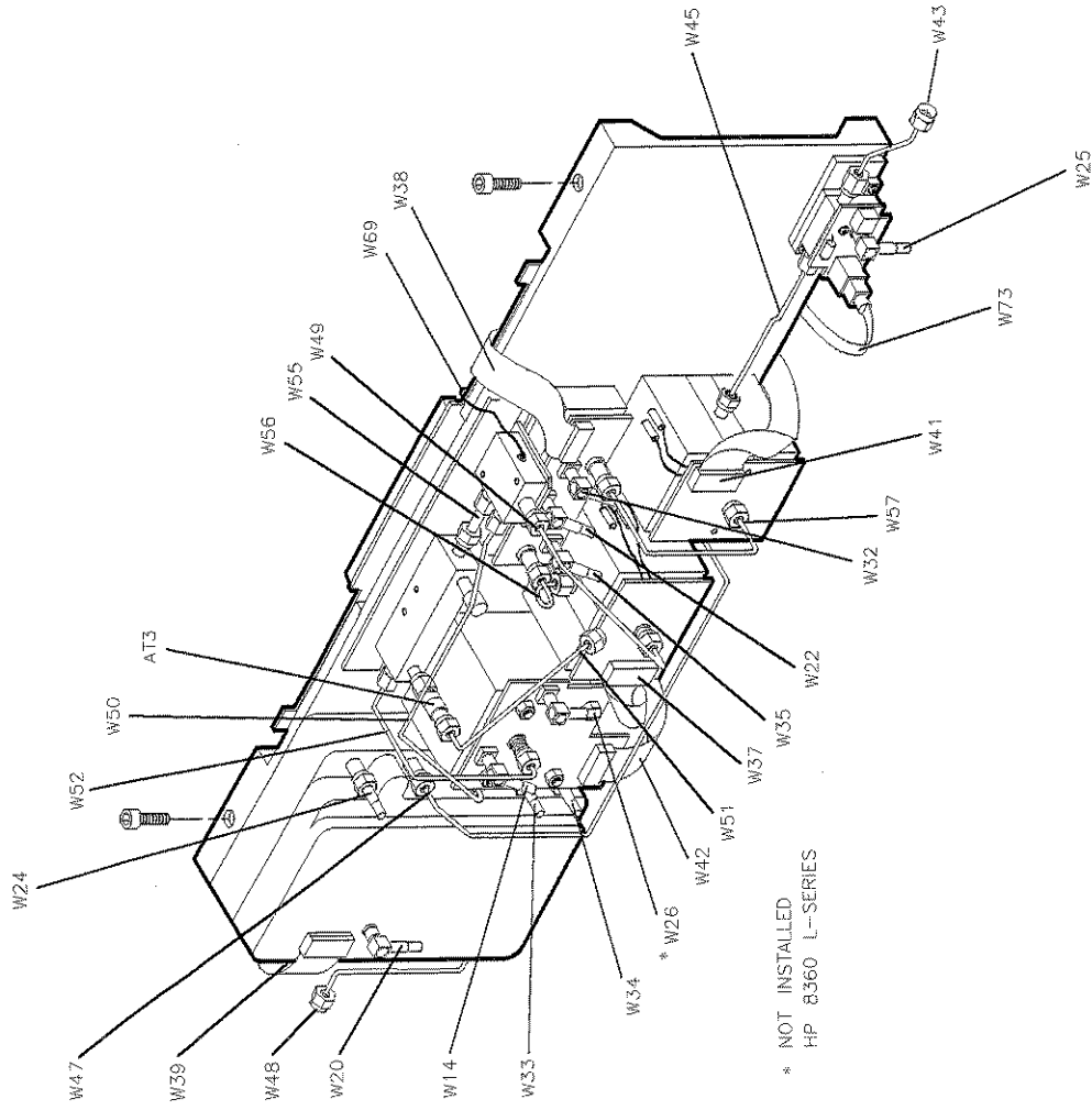
Figure 9-3. Cables (8 of 19)
