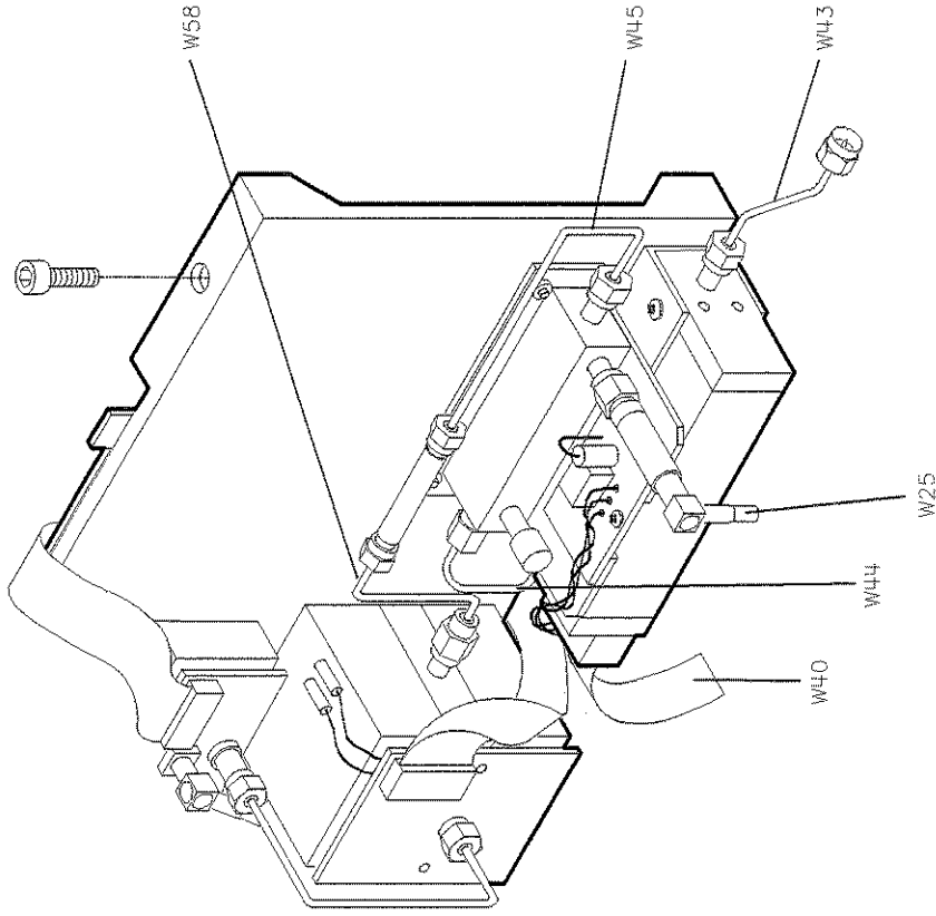
RF Deck Cable Locations - HP 83623L Option 001
