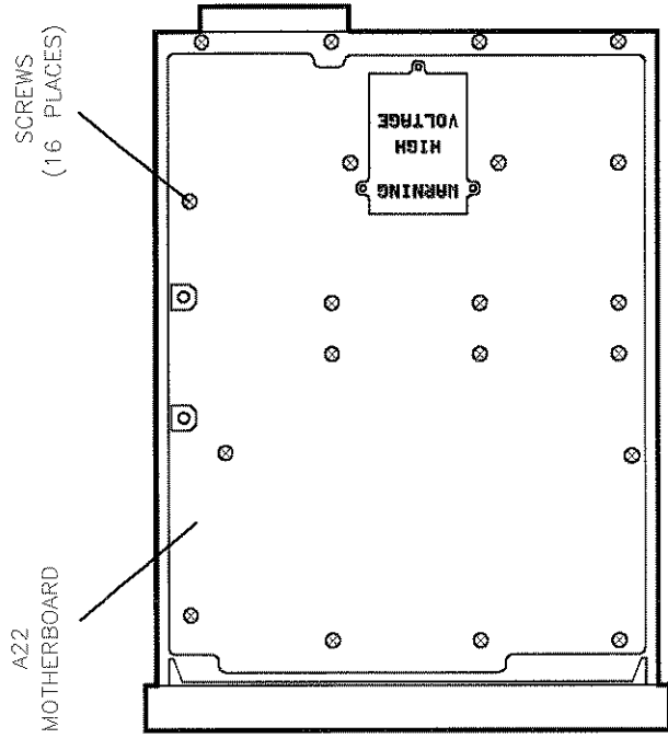
Figure 7-62. Motherboard Screws
