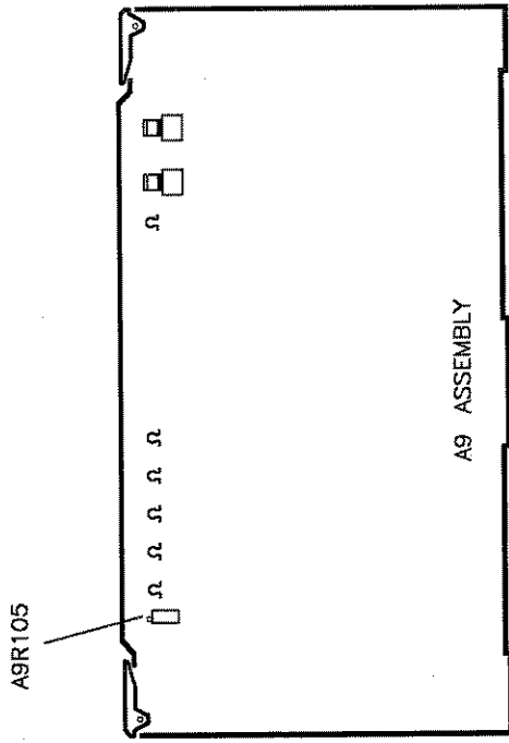
Figure 3-22. A9R105 Location
