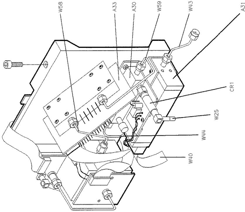
Figure 9-3. Cables (15 of 19)
