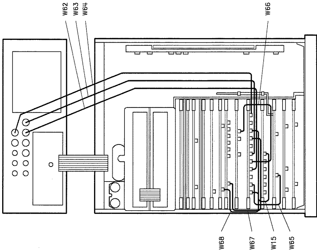
Figure 9-3. Cables (3 of 19)
