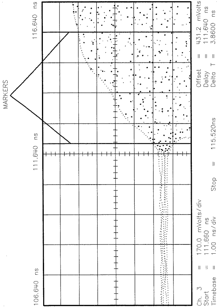
Figure 2-17. Widened Pulse Envelope
