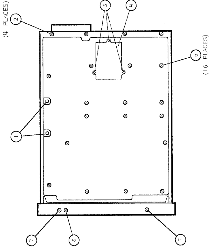
Figure 9-9. Bottom View, Attaching Hardware
