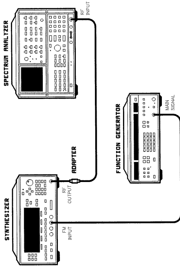
Figure 3-32. FM Gain Adjustment Setup
