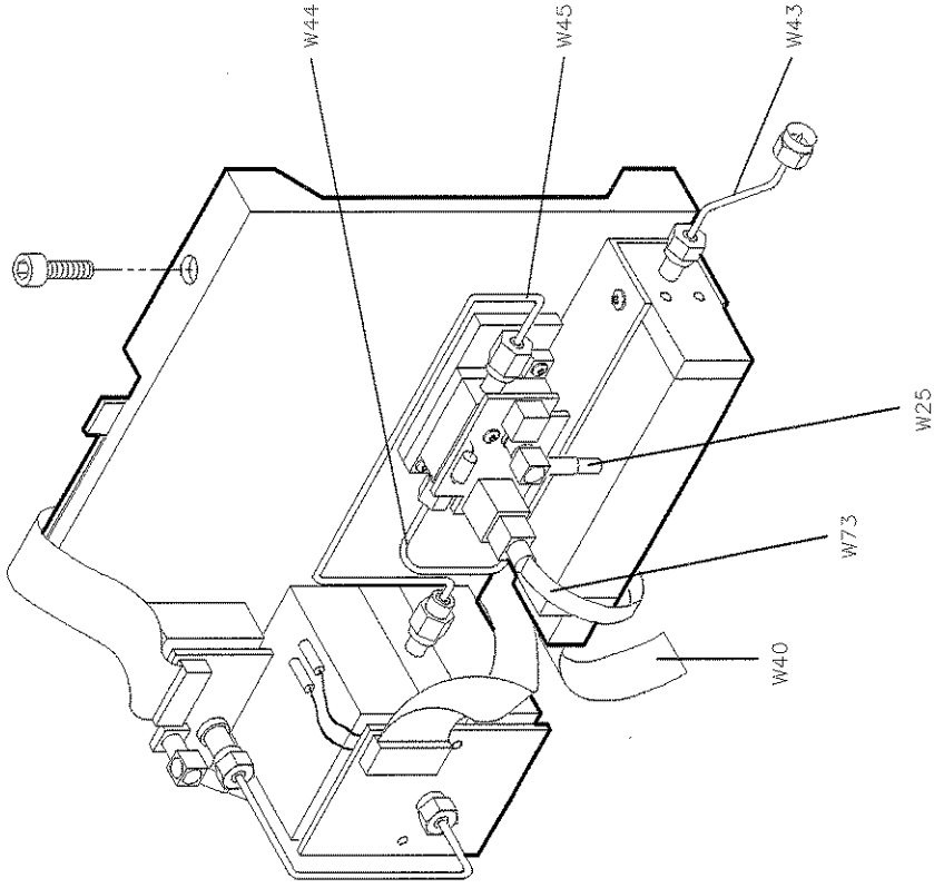
Figure 9-3. Cables (9 of 19)
