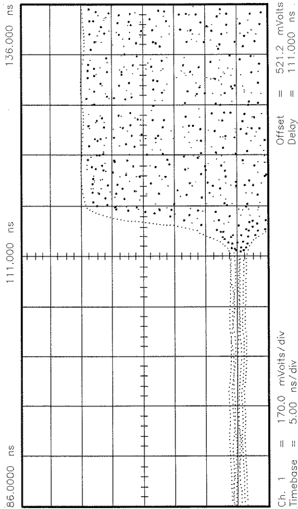
Figure 2-16. Pulse Envelope Displayed Over 5 Divisions
