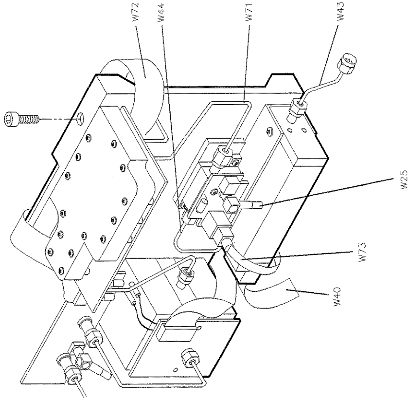
Figure 9-3. Cables (11 of 19)
