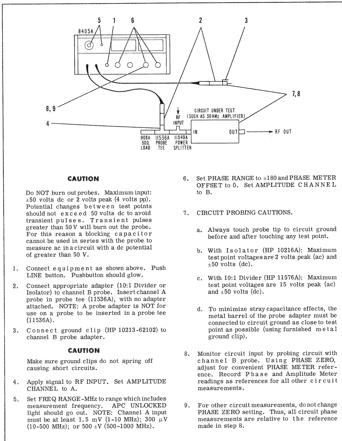
Figure 3-4. In-Circuit Measurements
