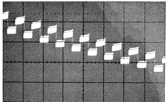
Typical Sampling Waveform When A11R23 Improperly Adjusted.
