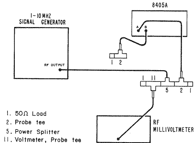
Figure 2K. Setup for RF Gain Adjustment
