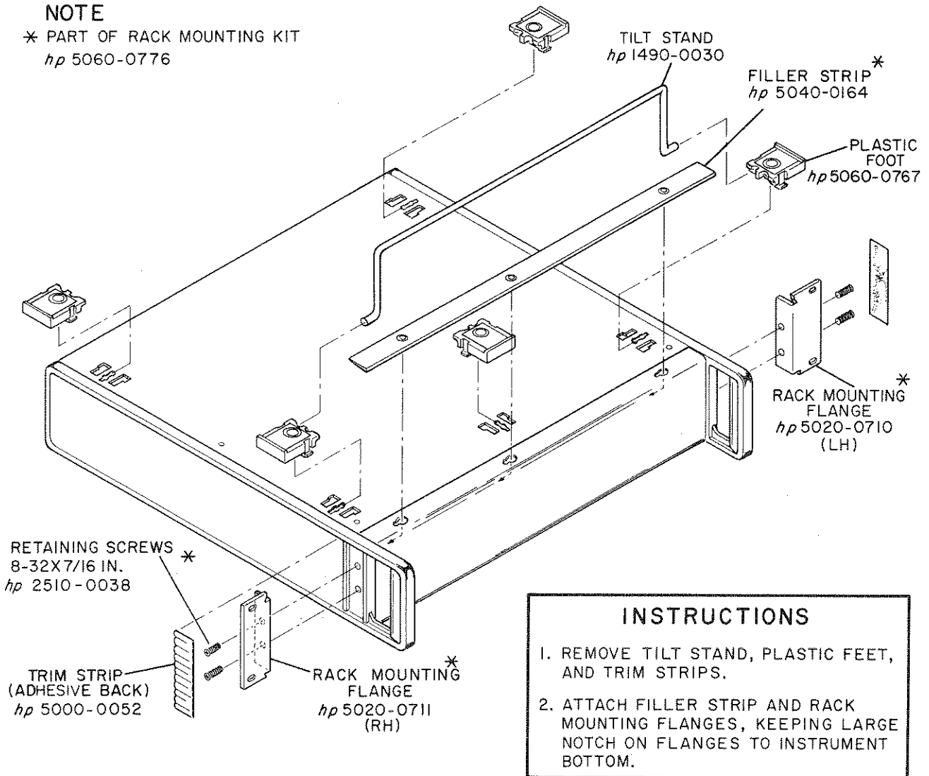
Figure 2-1. Preparation for Rack Mounting
