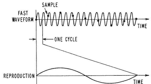
Figure 4-3. Fast Waveform Reproduced on Slower Time Base by Sampling
