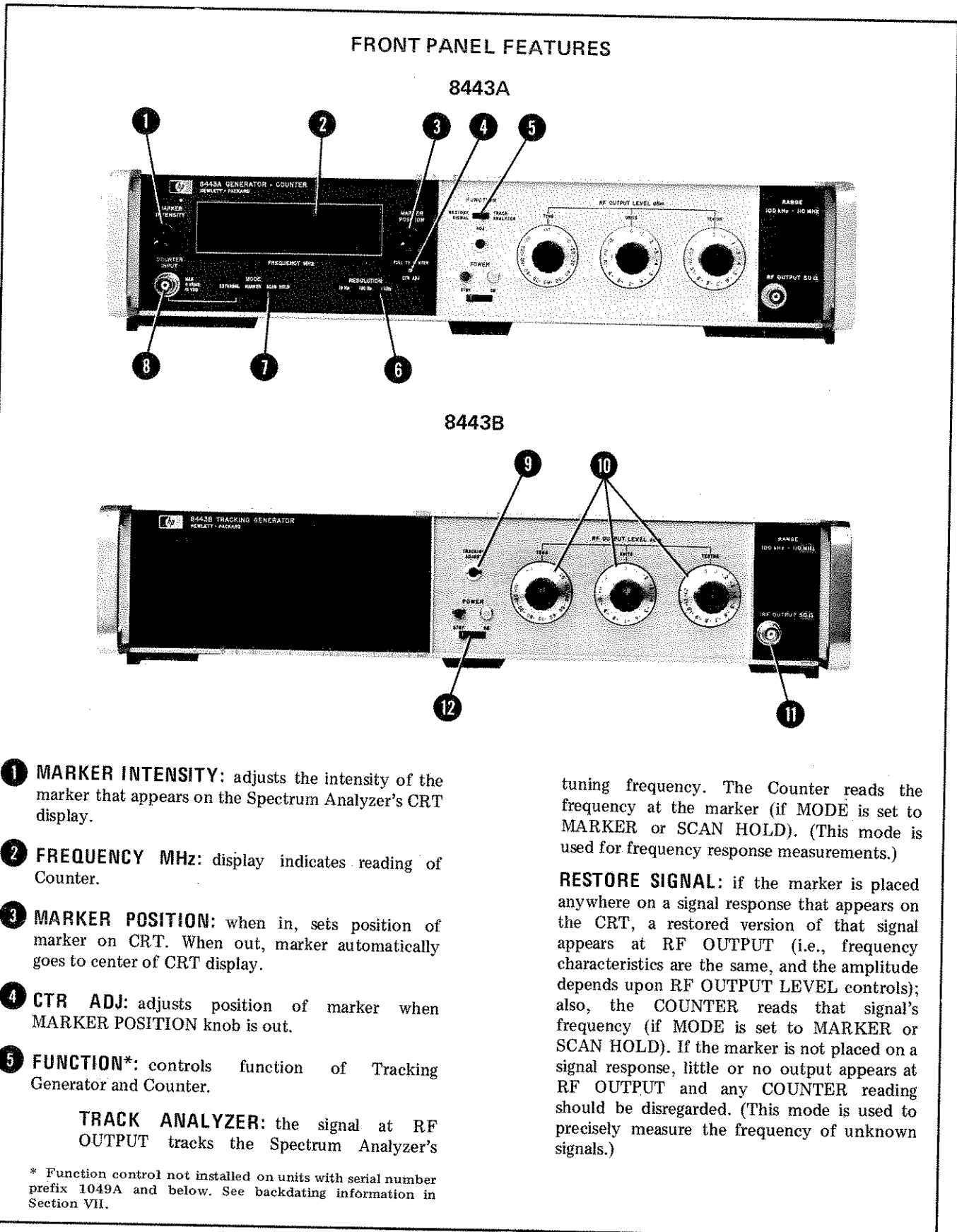
Figure 3-1. Front Panel Controls, Indicators, and Connectors (1 of 2)
