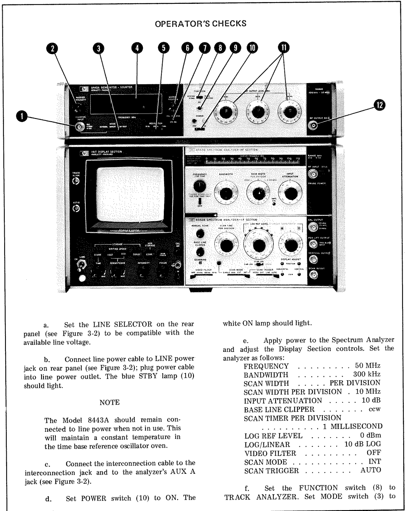
Figure 3-3. Operator's Checks (1 of 2)
