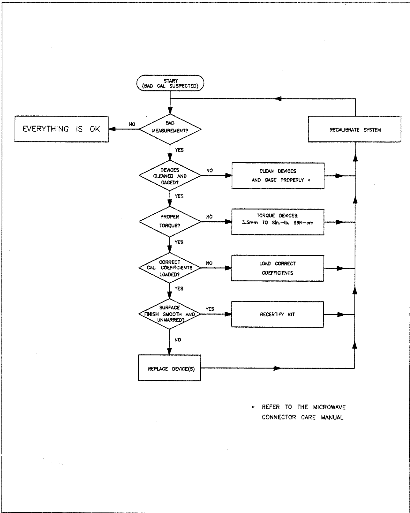
Figure 5-1. Troubleshooting Flowchart
