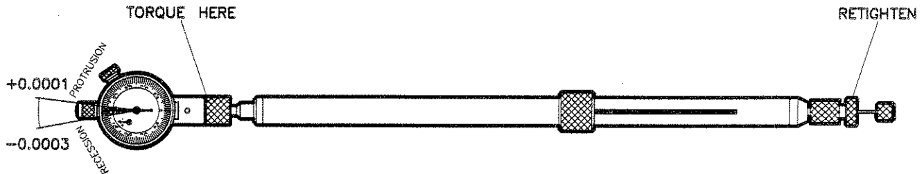
Figure 4-2. Gaging the Sliding Load Termination
