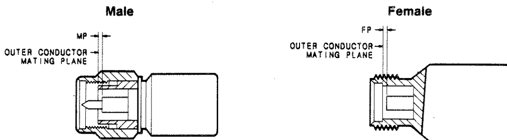
Figure 2-1. 3.5 mm Terminations
