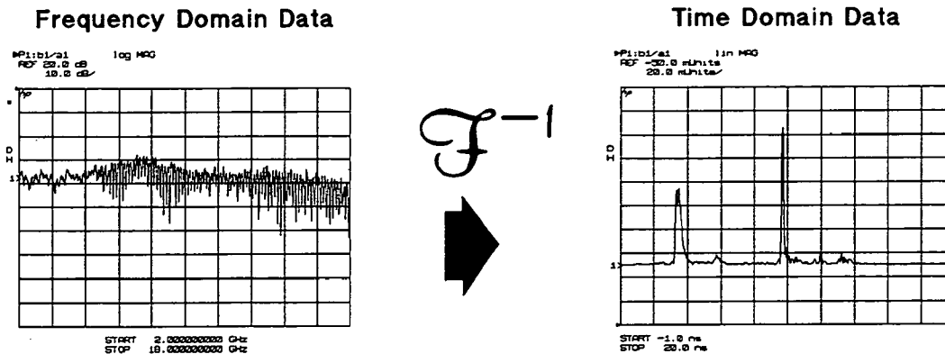
Figure 1-4. Time Domain
