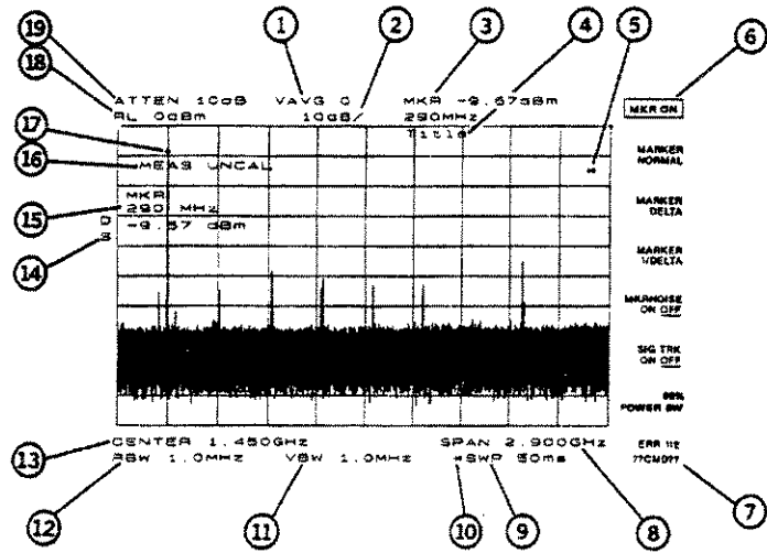
Figure 1-2. Display Annotation
