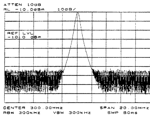
Figure 1-7. Frequency, Span, and Amplitude Set for Calibration
