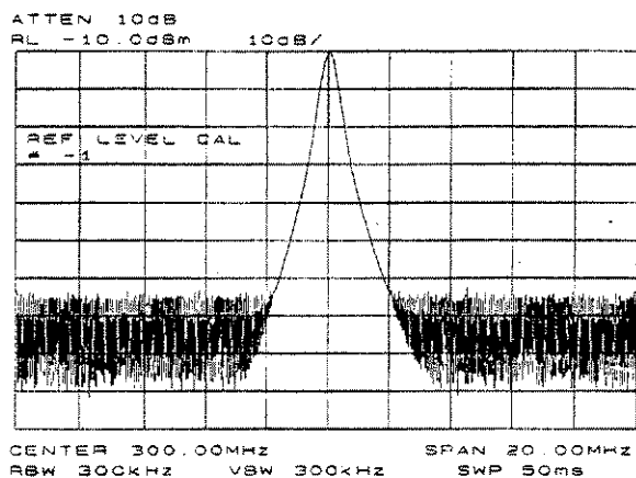
Figure 1-8. Signal Peak Calibrated to the Reference Level
