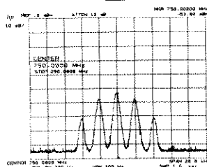
Third Harmonic
