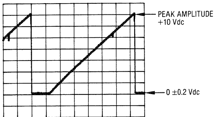
Figure 5-45. Sweep Out Waveform
