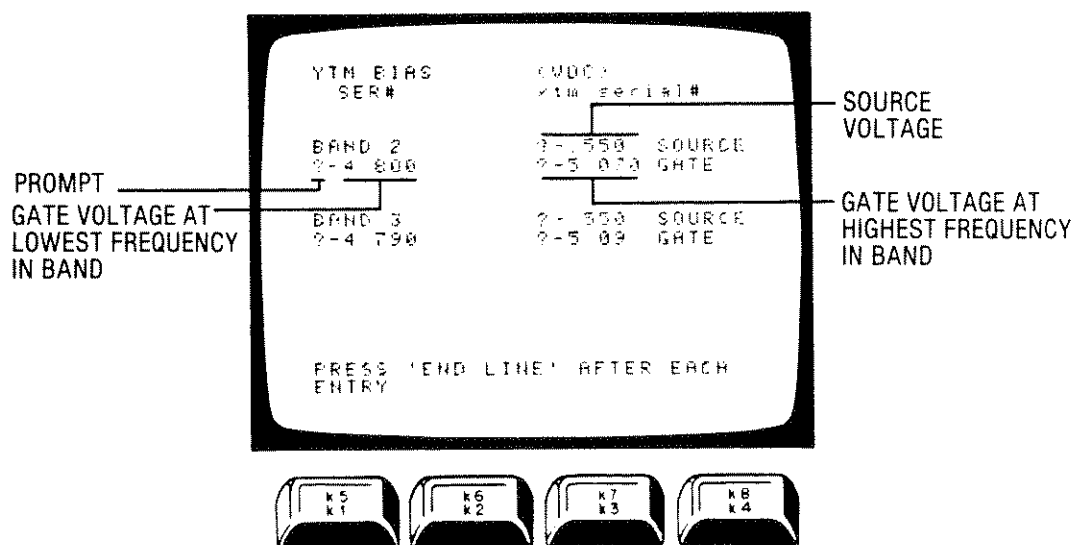
Figure 5-18. Format for Entering SRD Bias Voltages
