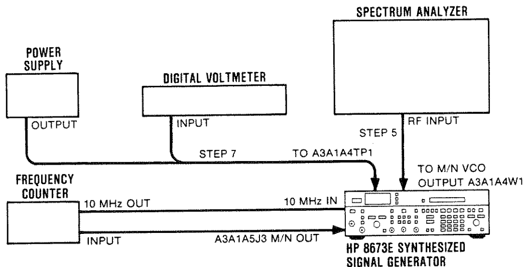
Figure 5-6. M/N Loop Adjustment Test Setup
