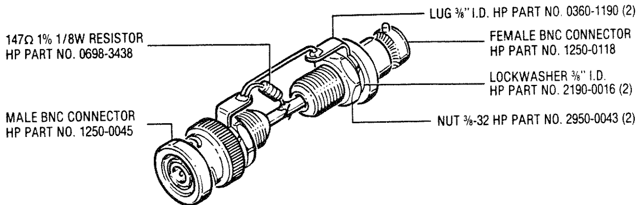
Figure 5-34. Pulse Shunt Adapter
