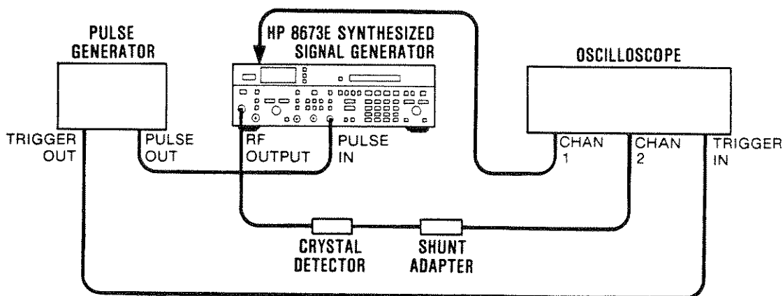
Figure 5-35. ALC Sample Pulse Adjustment Test Setup
