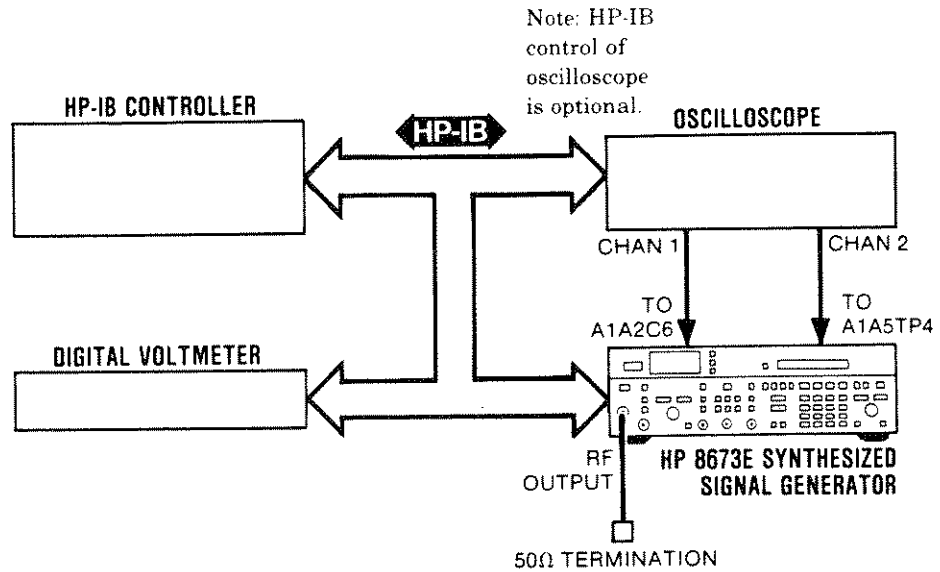
Figure 5-22. YTM Tune Adjustment Test Setup
