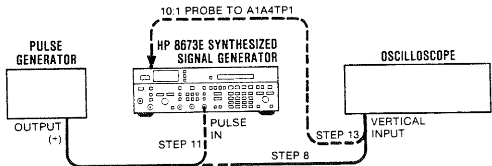
Figure 5-32. Series Pulse Width Adjustment Test Setup
