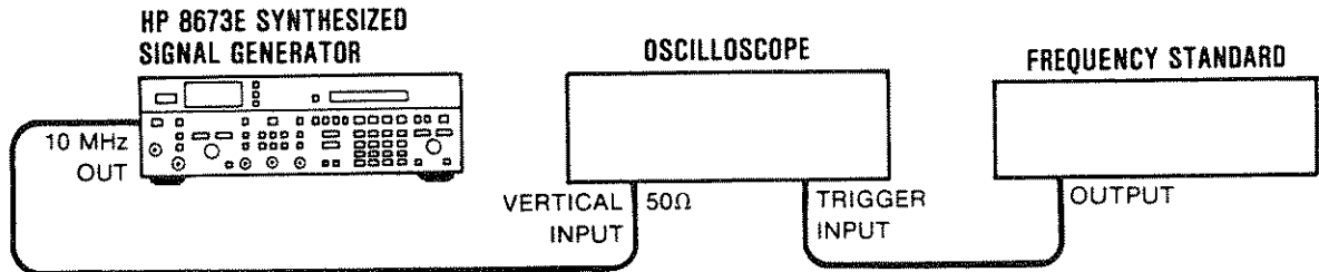
Figure 5-4. 10 MHz Reference Oscillator Adjustment Test Setup
