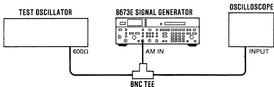
Figure 3-8. AM Functional Check Setup
