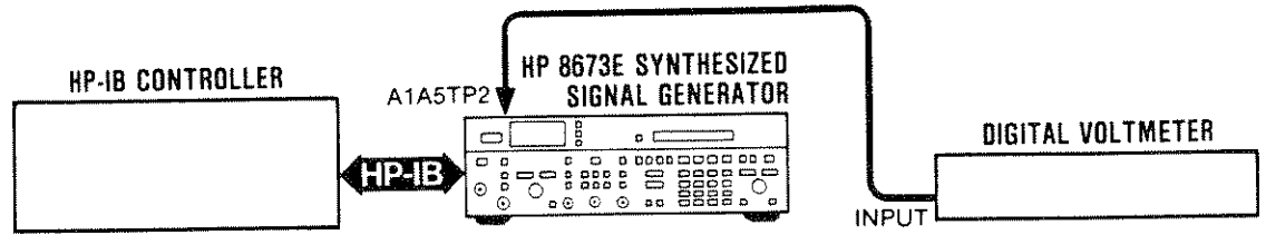
Figure 5-31. PAC DAC Adjustment Test Setup
