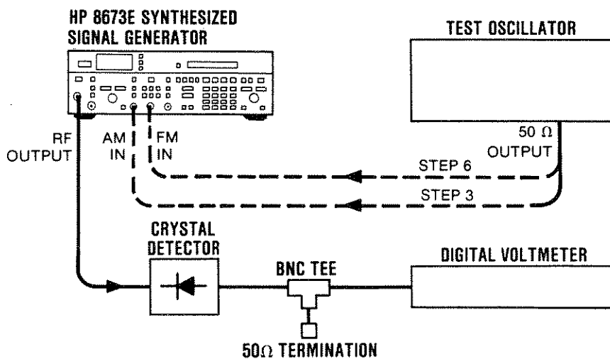
Figure 4-10. Incidental AM Test Setup
