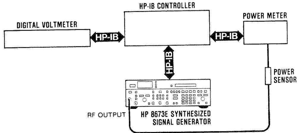
Figure 5-28. Flatness and ALC Adjustment Test Setup
