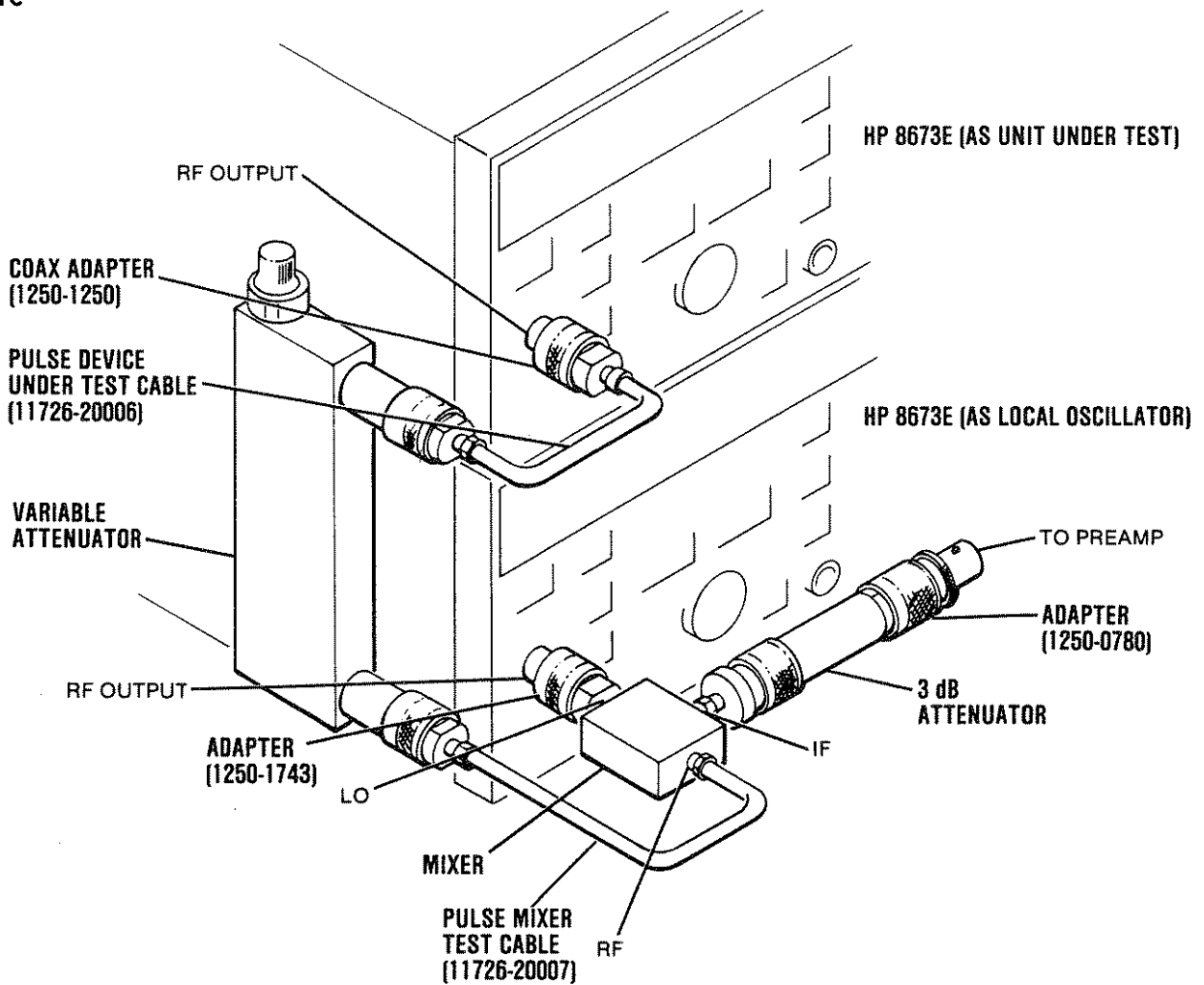
Figure 4-12. Equipment Interconnection for Pulse Test
