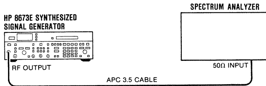
Figure 4-14. On-Off Ratio Test Setup
