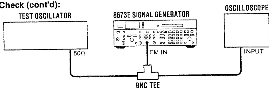
Figure 3-9. FM Functional Check Setup
