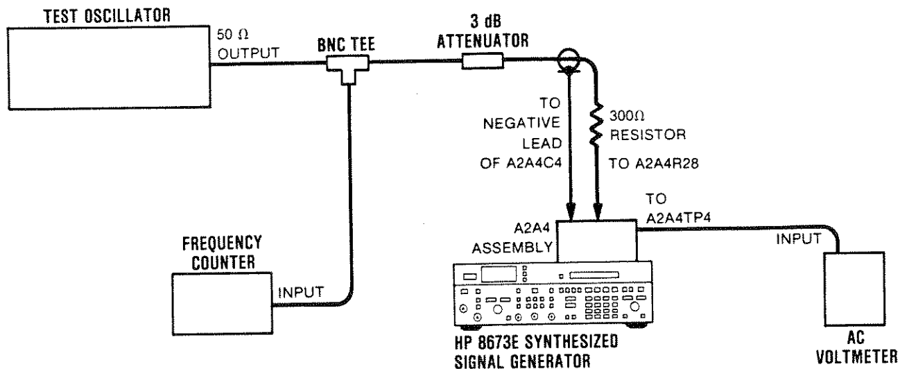
Figure 5-8. LFS Loop Notch Filter Adjustment Test Setup
