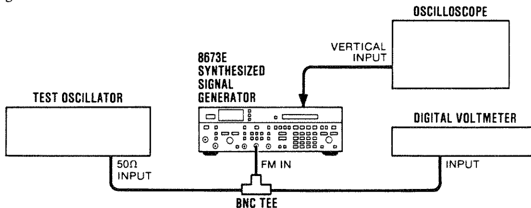
Figure 5-16. FM Driver Adjustment Test Setup
