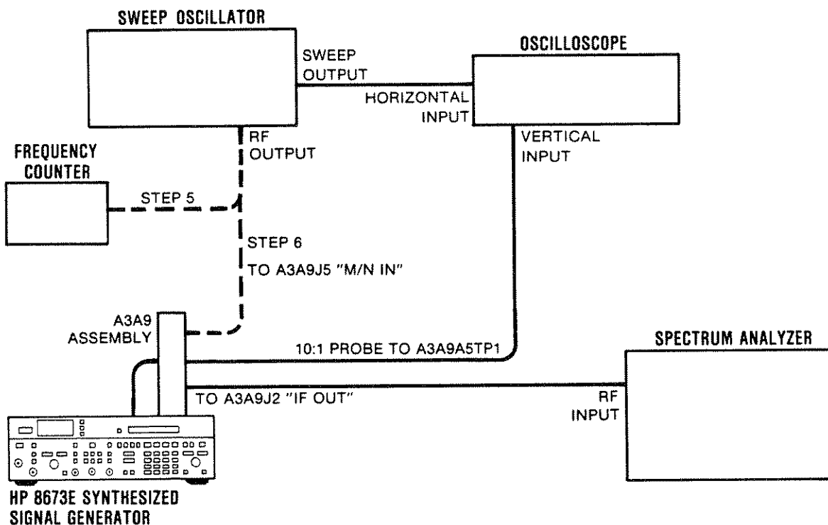
Figure 5-9. YTO Loop Sampler Adjustment Test Setup
