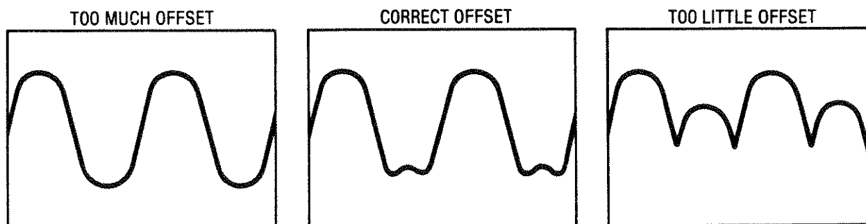
Figure 5-12. YTO Loop Offset Adjustment Waveforms
