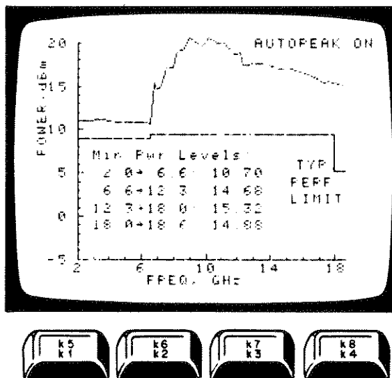
Figure 5-25. Maximum Power Plot
