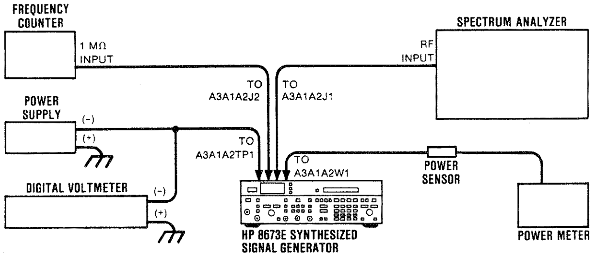
Figure 5-5. Reference Loop (VCXO) Adjustment Test Setup
