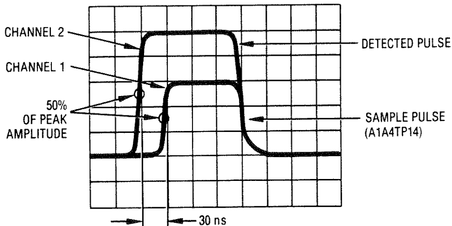
Figure 5-36. ALC Sample Pulse Waveform
