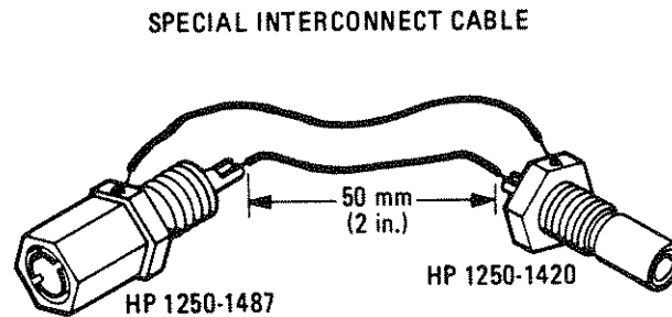
Figure 5-14. Special Interconnect Cable
