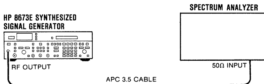
Figure 4-5. Non-Harmonically Related Spurious (CW and AM Modes) Test Setup
