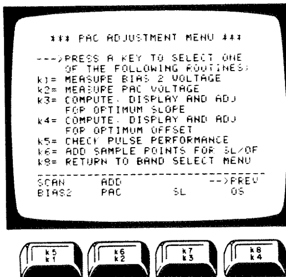
Figure 5-39. PAC Adjustment Menu
