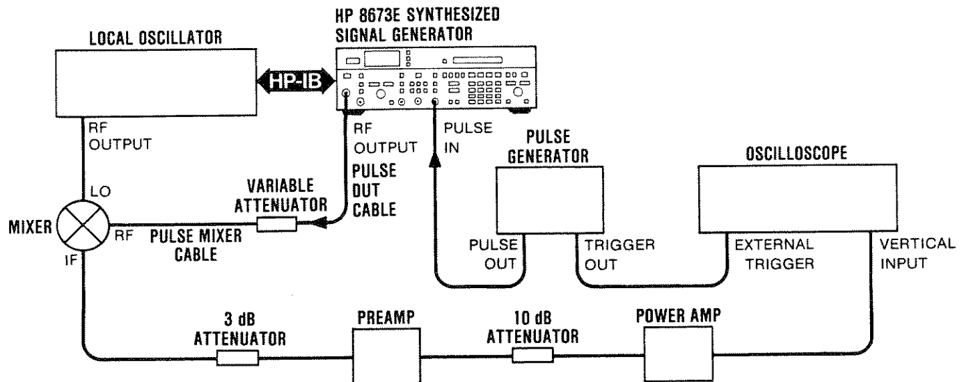
Figure 4-11. Pulse Overshoot and Ringing Test Setup
