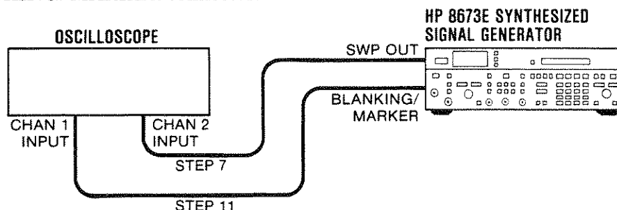
Figure 5-44. Sweep Out and Blanking/Marker Adjustments Test Setup
