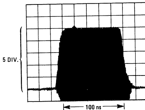
Figure 4-13. Overshoot and Ringing Measurement Display
