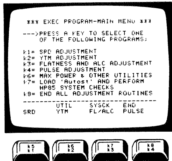
Figure 5-2. Main Menu
