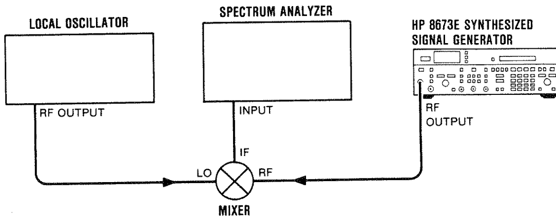
Figure 4-6. Single-Sideband Phase Noise Test Setup
