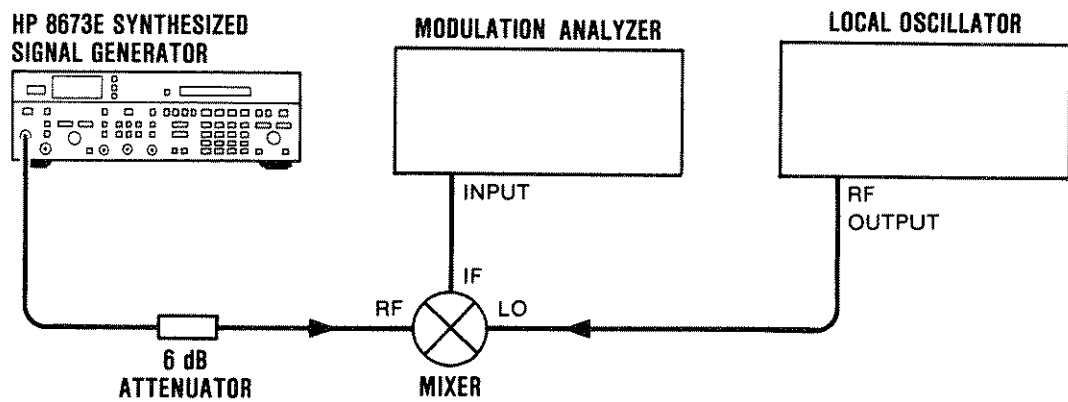
Figure 4-7. Residual AM Test Setup
