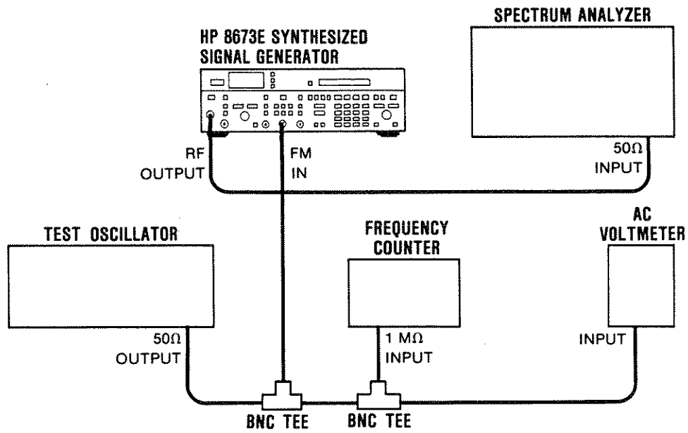
Figure 4-9. FM Frequency Response Test Setup
