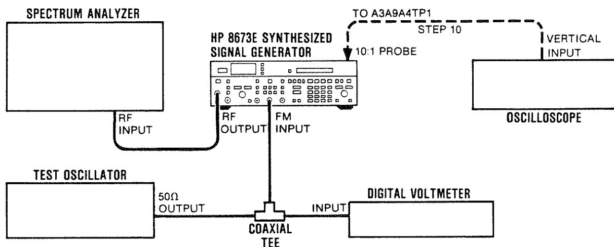
Figure 5-11. YTO Loop Offset and FM Overmodulation Adjustment Test Setup
