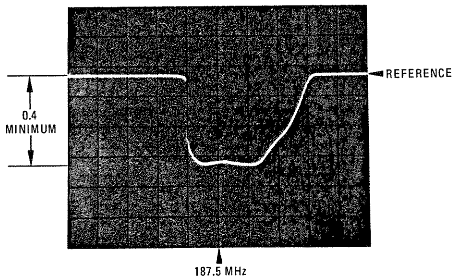
Figure 5-10. Sampler Frequency Response
