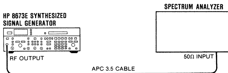
Figure 4-4. Harmonics, Subharmonics, and Multiples Test Setup
