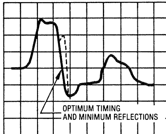
Figure 5-33. Series Pulse Width Waveform
