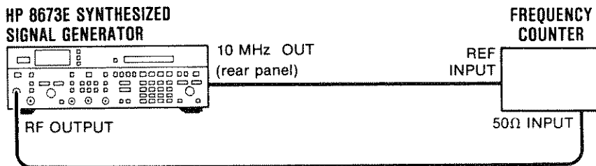
Figure 4-1. Frequency Range and Resolution Test Setup
