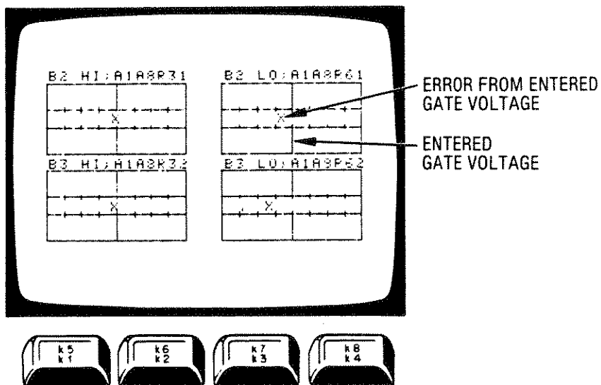
Figure 5-19. Gate Voltage Adjustment
