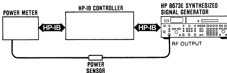
Figure 5-23. Power Clamp Adjustment Test Setup
