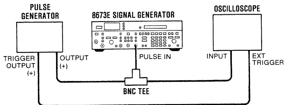
Figure 3-10. Pulse Modulation Functional Check Setup
