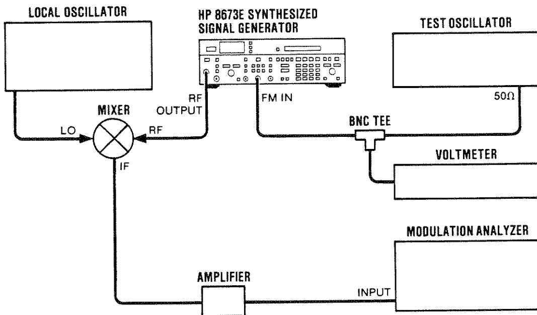
Figure 5-17. FM Accuracy and Overmodulation Adjustment Test Setup
