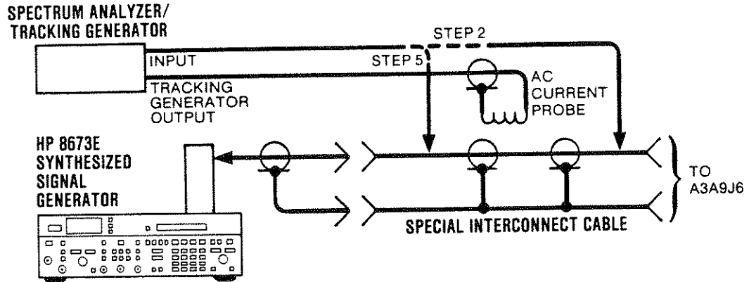
Figure 5-13. YTO Loop Phase Detector Adjustment Test Setup
