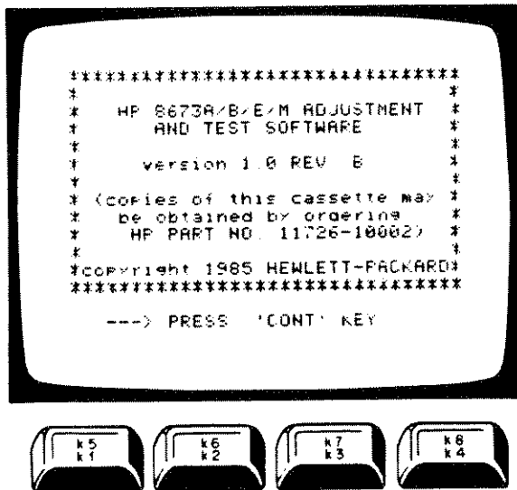
Figure 5-1. Title Screen
