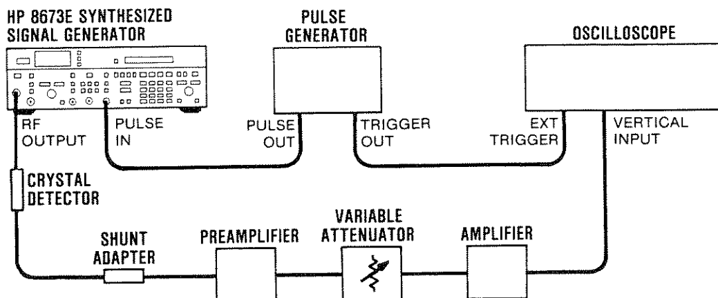
Figure 5-43. Pulse Amplitude Control Adjustment Test Setup
