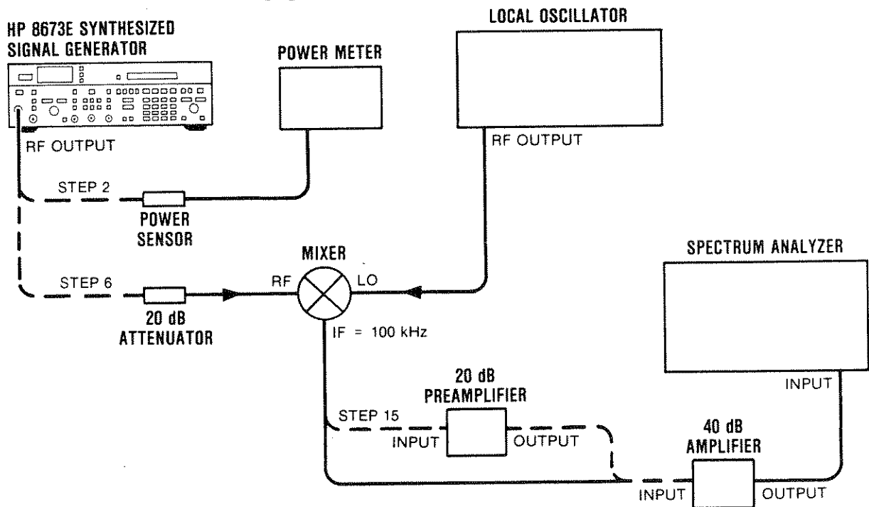
Figure 4-3. Low Level Accuracy Test Setup
