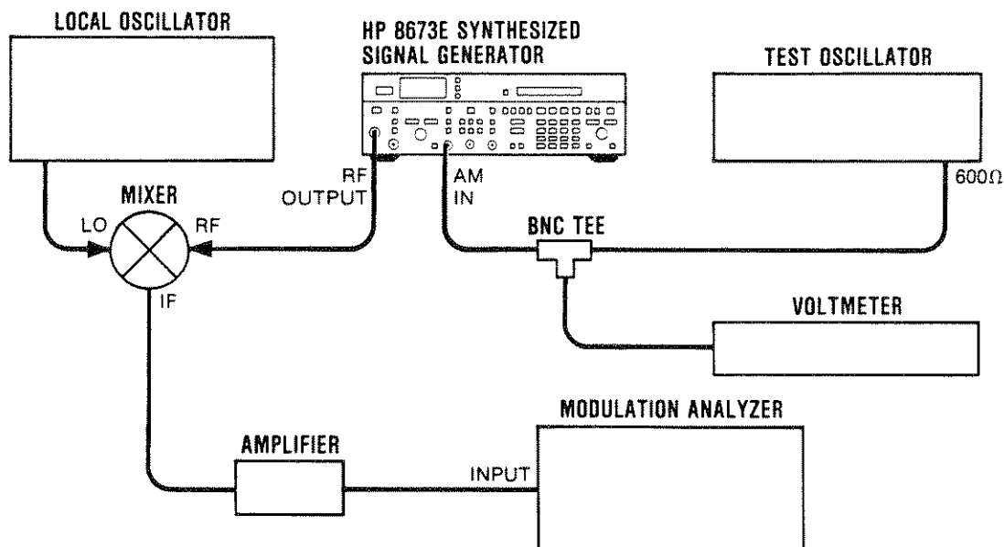
Figure 5-30. AM Accuracy and Meter Adjustment Test Setup
