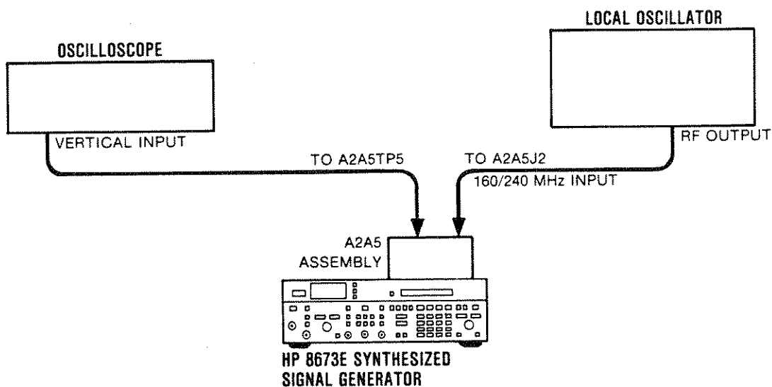
Figure 5-7. 20/30 MHz (LFS) Loop Divider Bias Adjustment Test Setup
