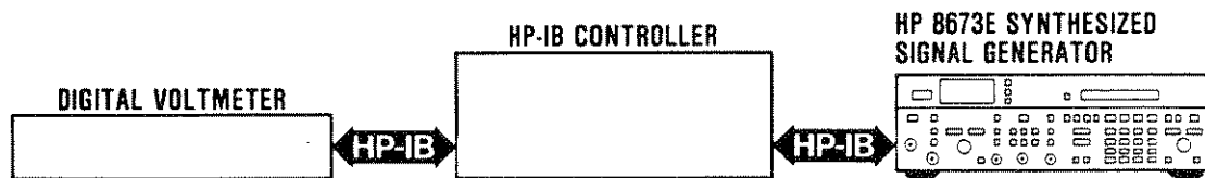
Figure 5-20. SRD Bias Adjustment Test Setup
