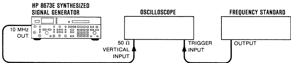
Figure 4-15. Internal Time Base Aging Rate Test Setup
