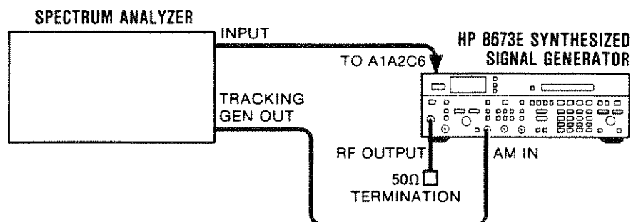
Figure 5-29. AM Bandwidth Adjustment Test Setup
