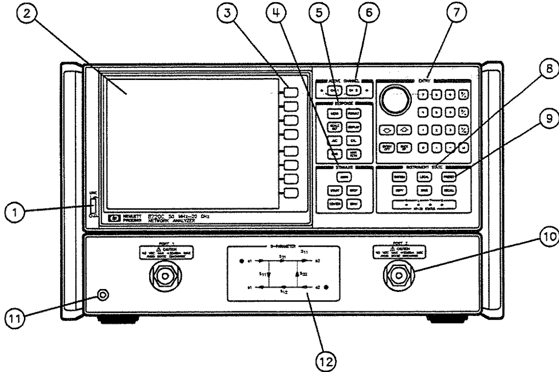
Figure 3-1. Front Panel
