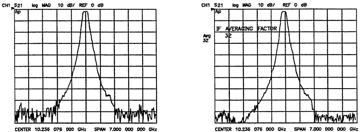
Figure 5-31. Effect of Averaging on a Trace
