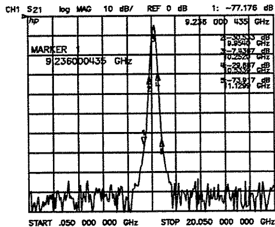
Figure 7-1. Markers on Trace
