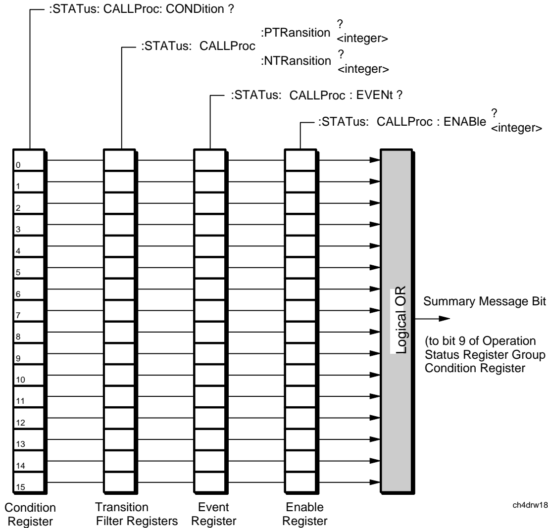
Figure 13 Call Processing Status Register Group
