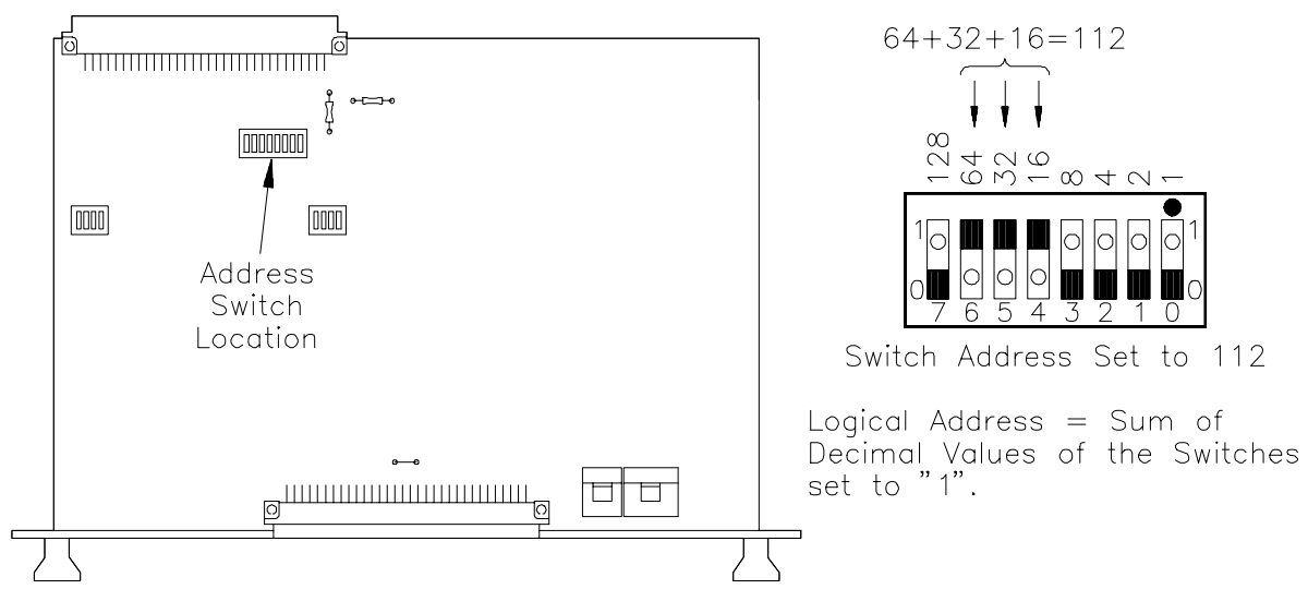
Figure 2-4. Setting the Logical Address Switch
