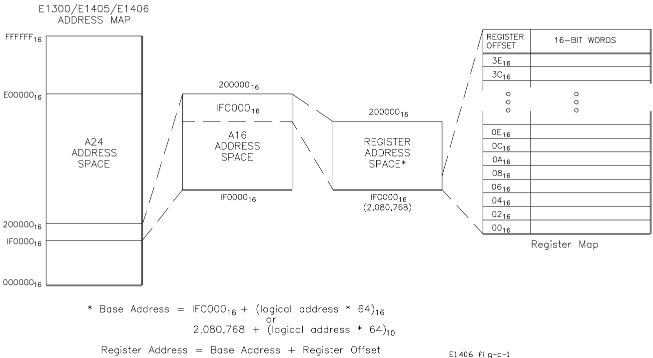
Figure C-1. HP E1406A Command Module A16 Address Space
