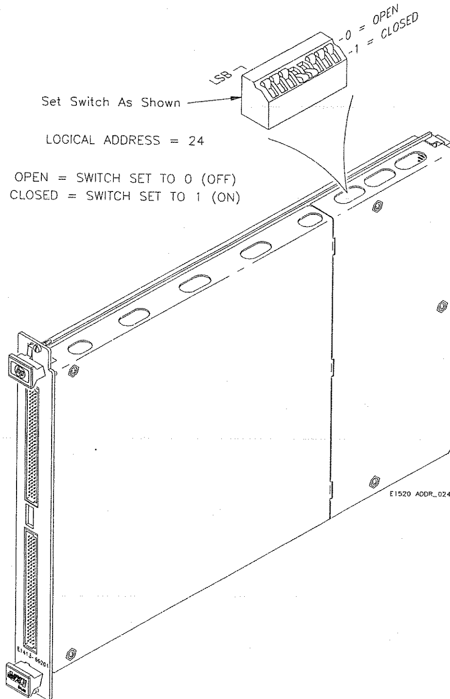
Figure 1-1 Setting Logical Address Switch
