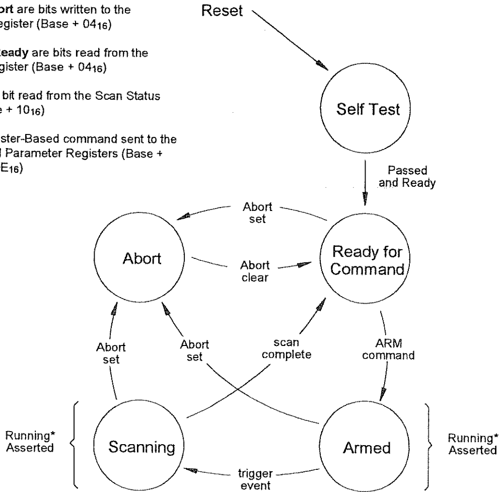
Figure D-7 Control Processor State Diagram
