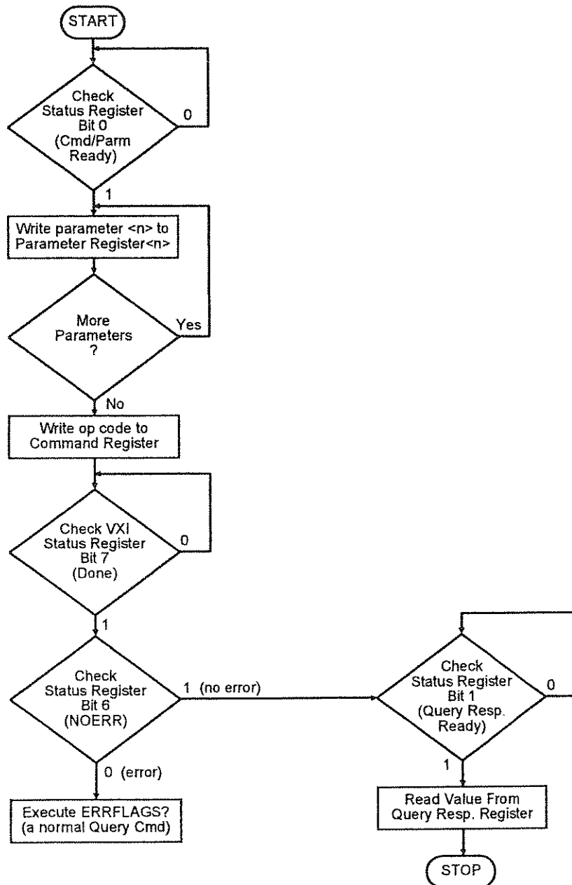
Figure D-6. Executing Queries
