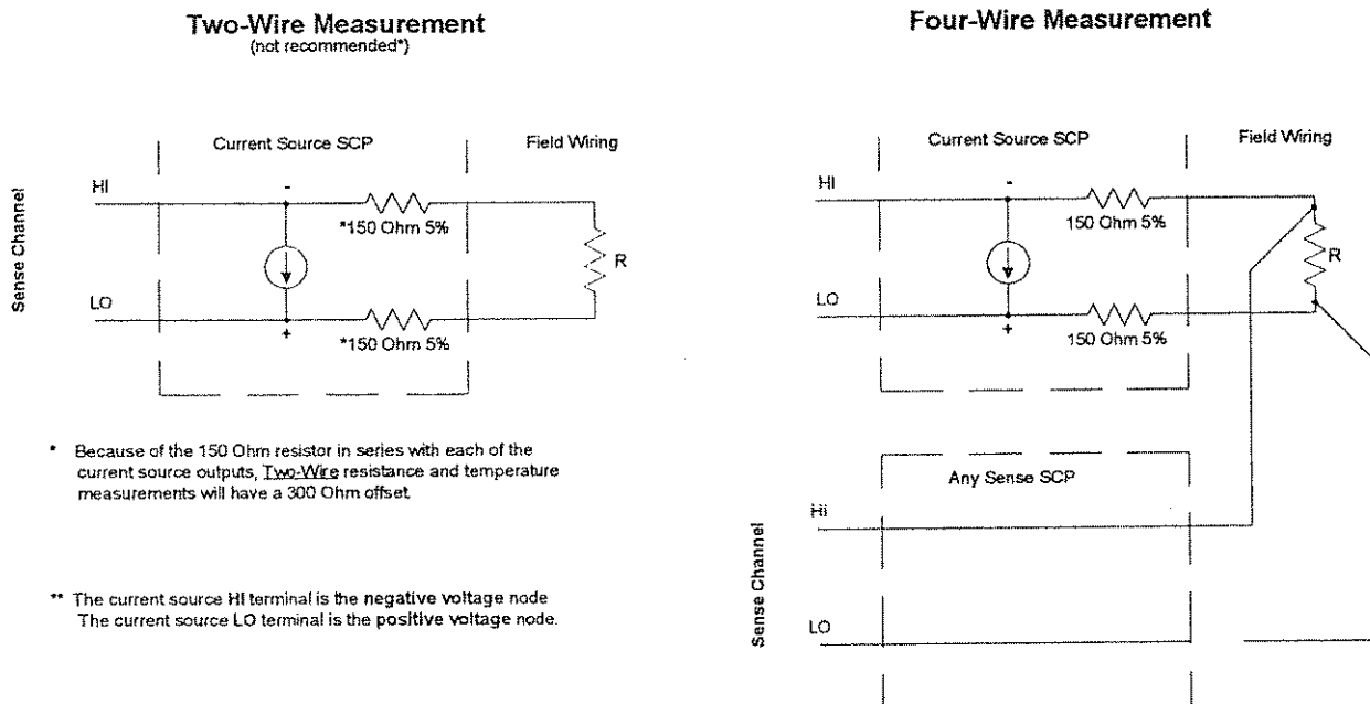
Figure 3-1 Resistance Measurement Sensing
