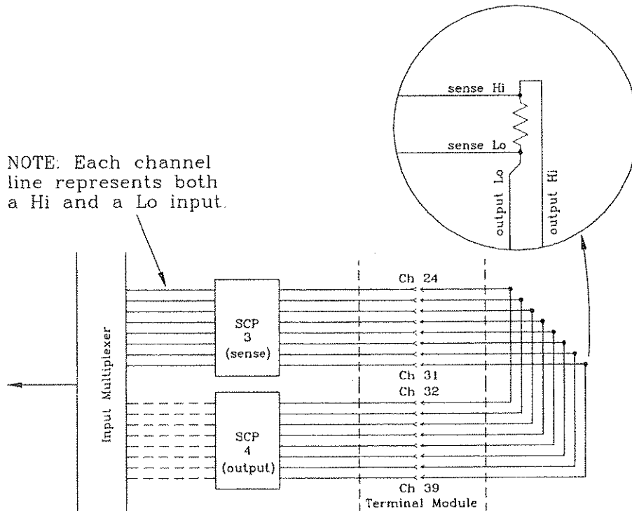
Figure 2-2 Pairing Output and Sense SCP Channels
