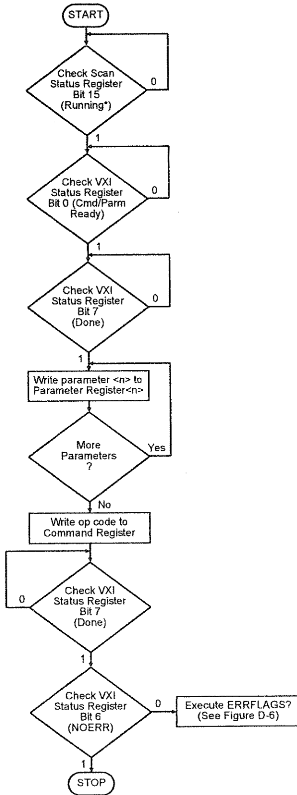
Figure D-5. Executing Commands
