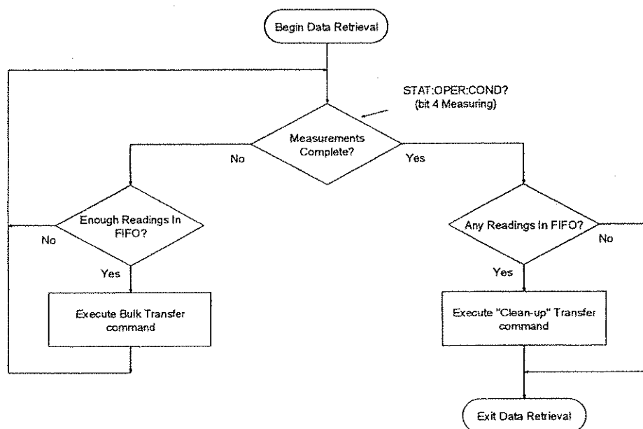
Figure 4-1 General Form of FIFO Data Retrieval
