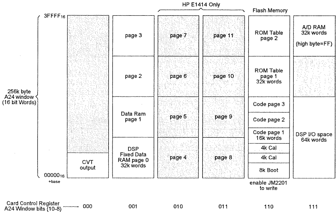
Figure D-2 A24 Memory Mapping
