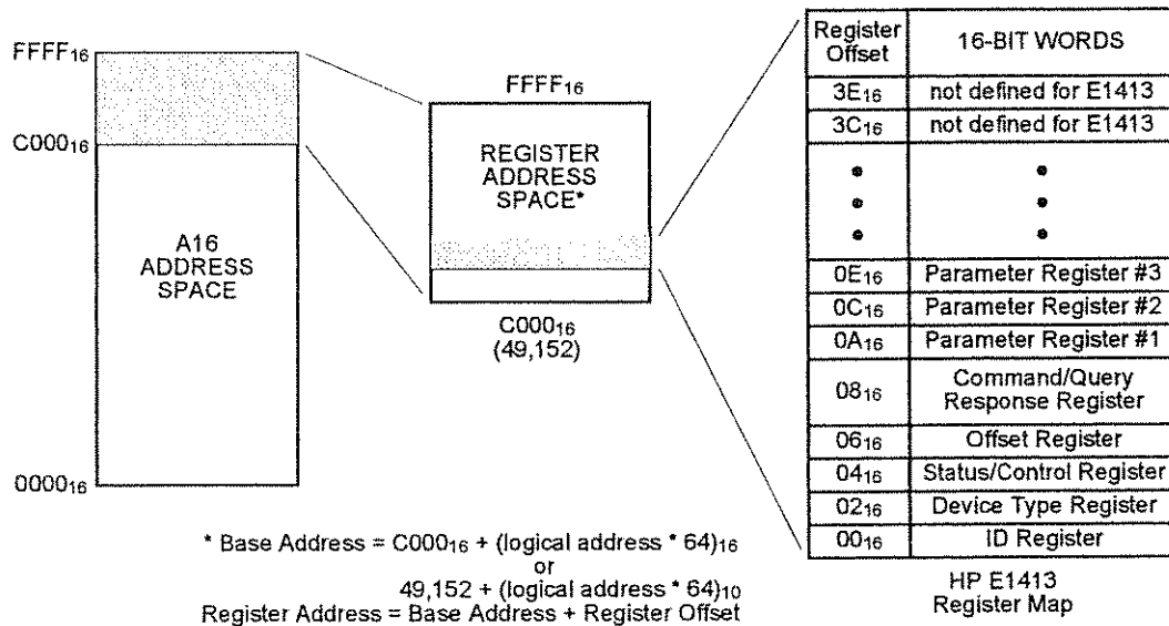
Figure D-1. E1413 Registers within A16 Address Space.
