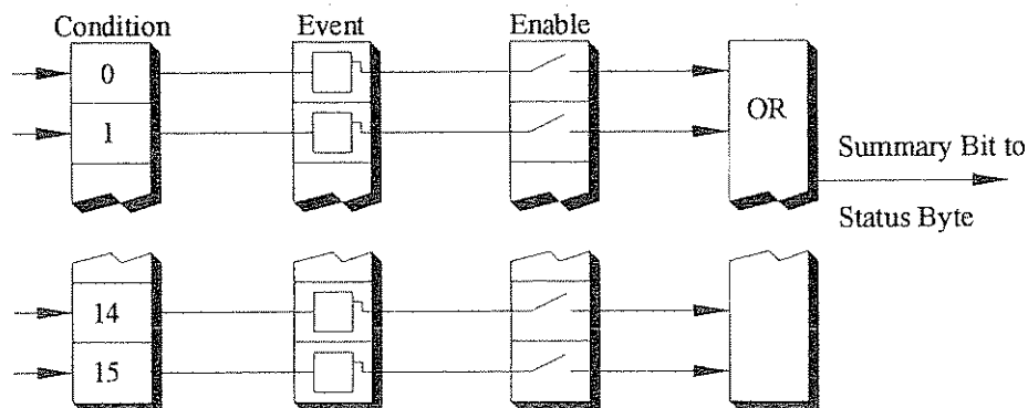
Figure 5-4 General Status Register Organization
