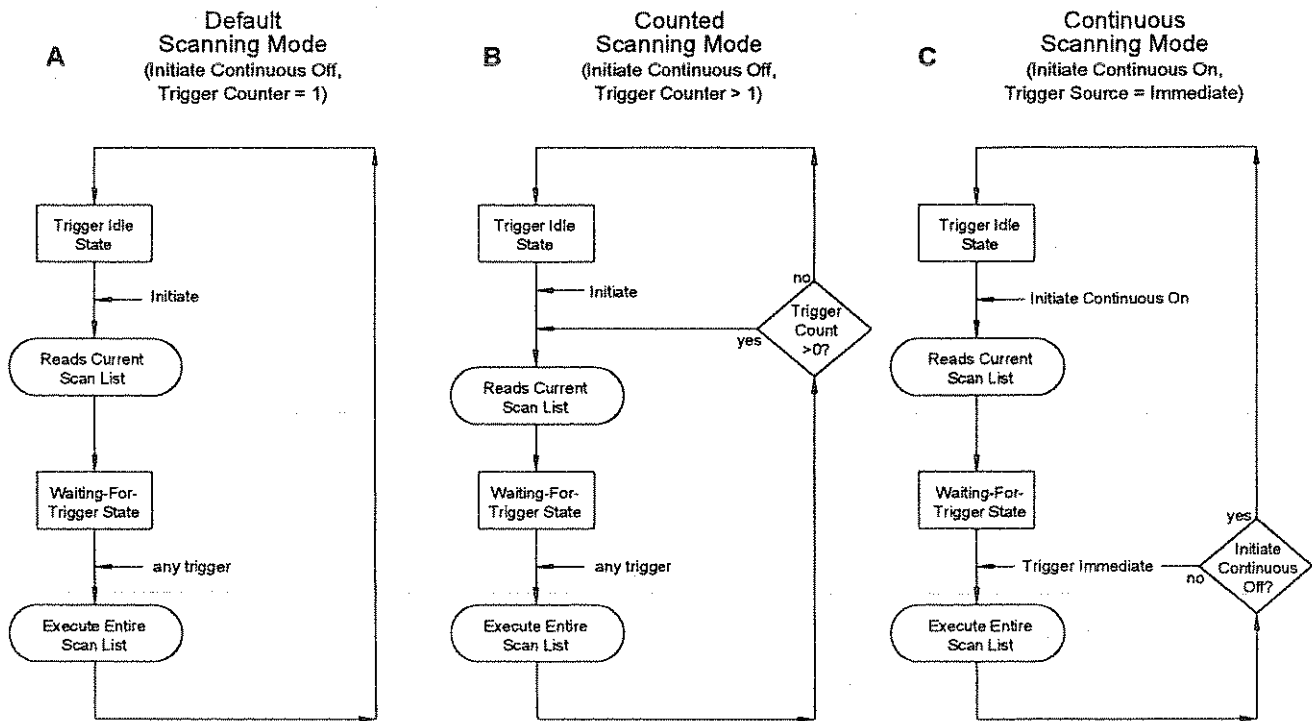
Figure 4-4 Scanning Modes
