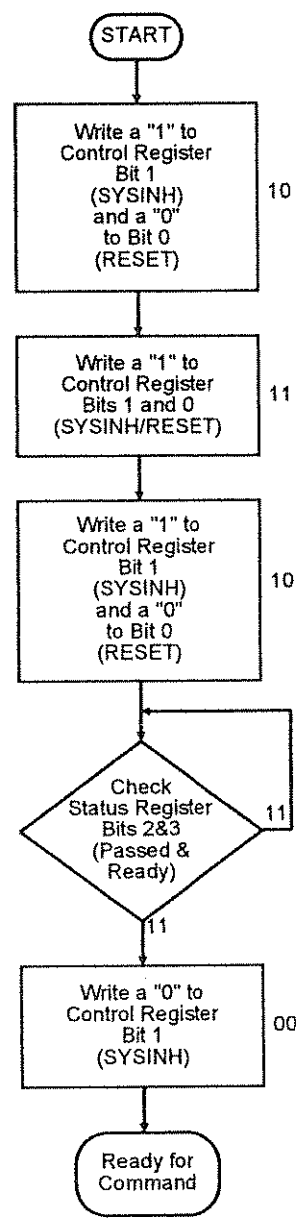
Figure D-3. Resetting the E1413A
