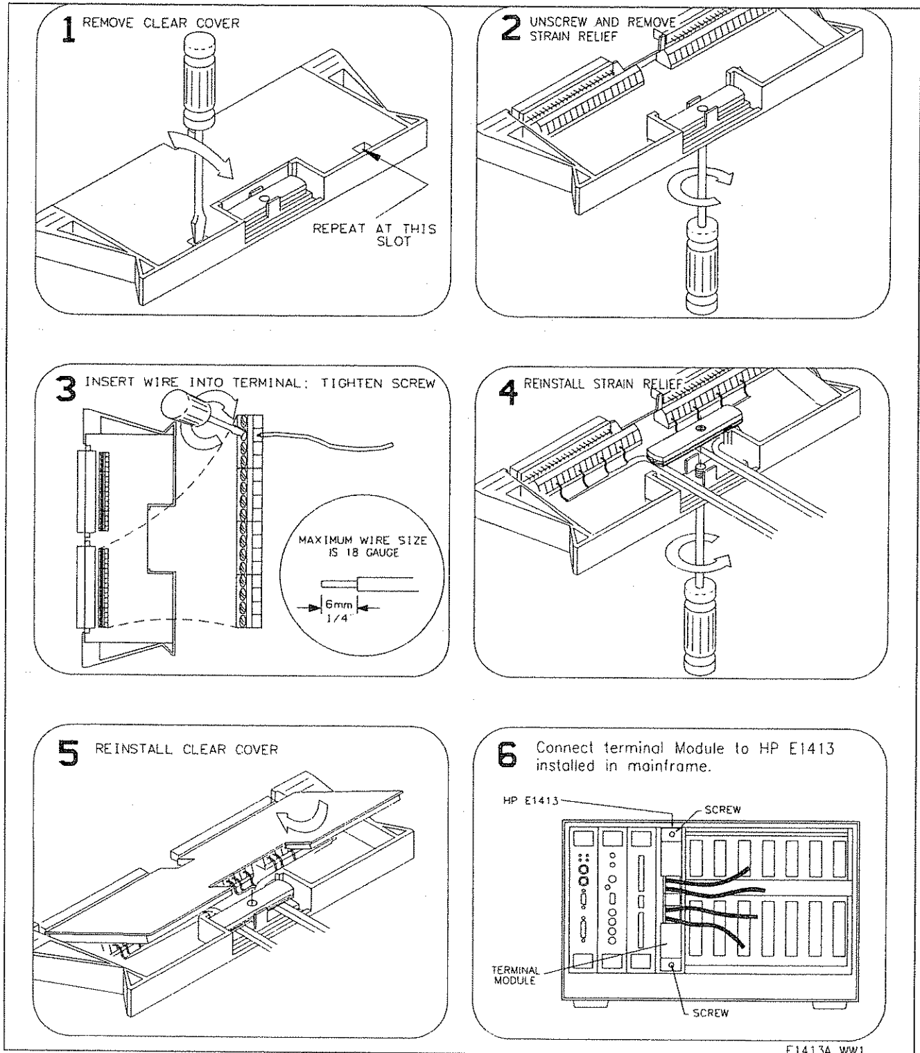
Figure 2-7 Opening And Wiring the Terminal Module
