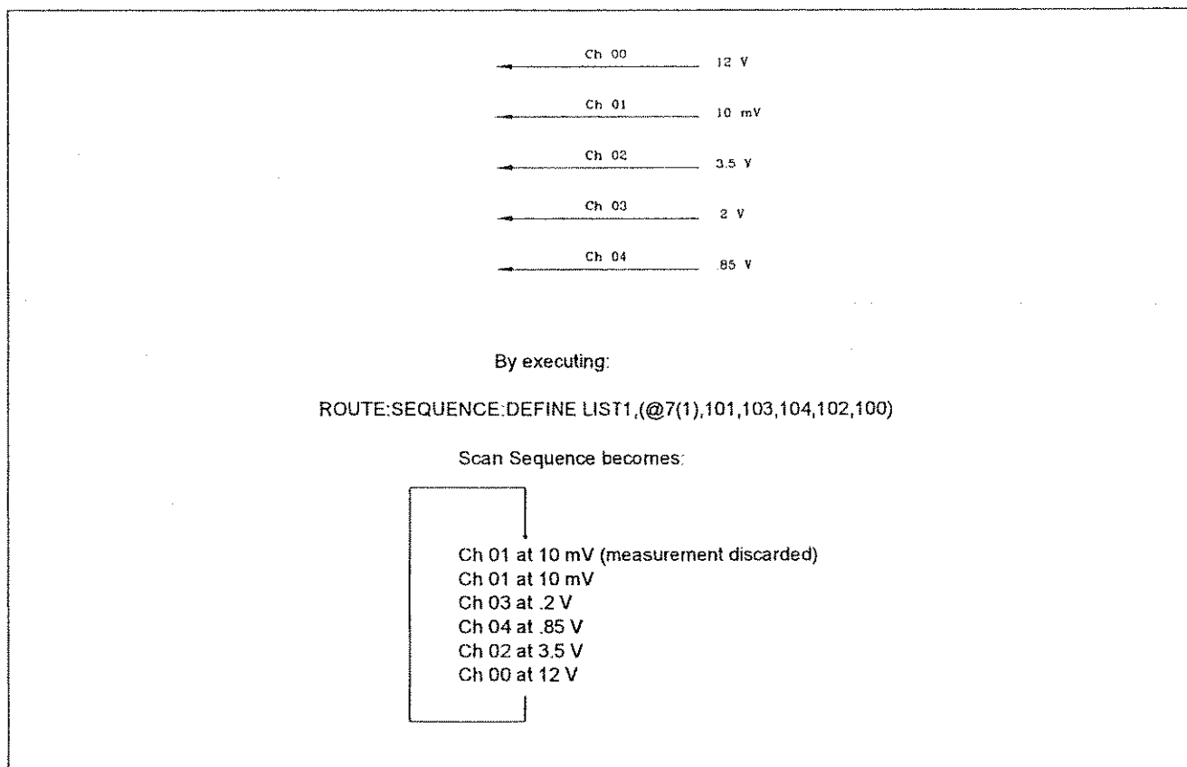
Figure 4-6 Recommended Scanning Sequence
