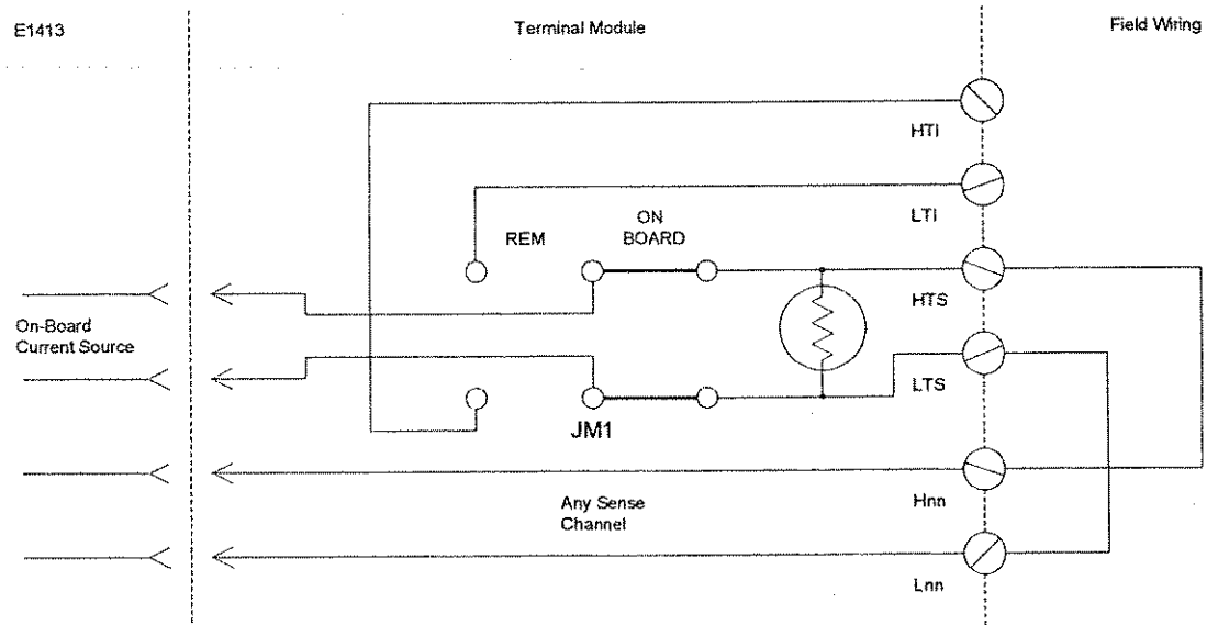
Figure 2-4 On-Board Thermistor Connections
