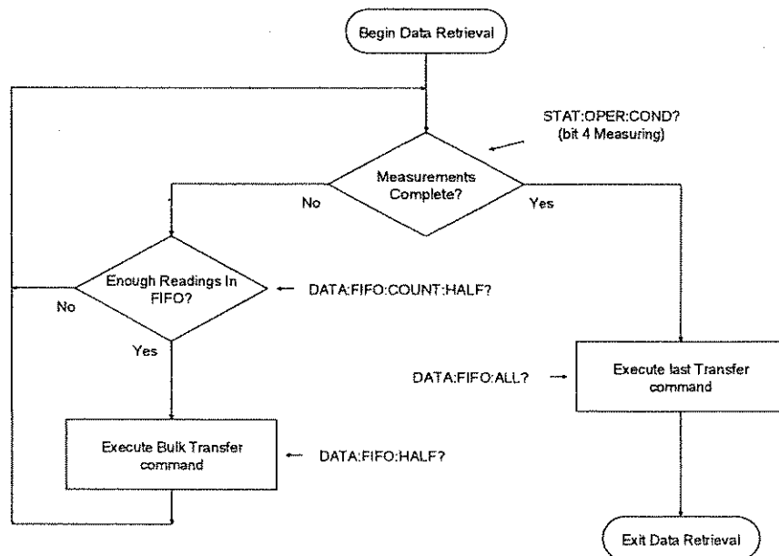
Figure 4-3 Fastest Reading Transfer
