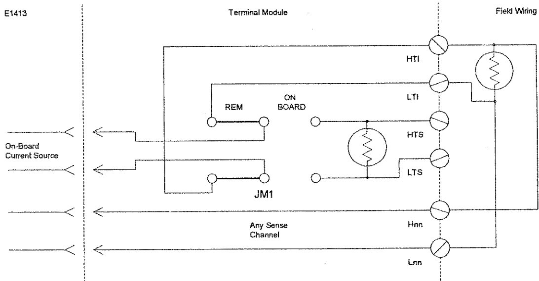
Figure 2-3 Remote Thermistor or RTD Connections
