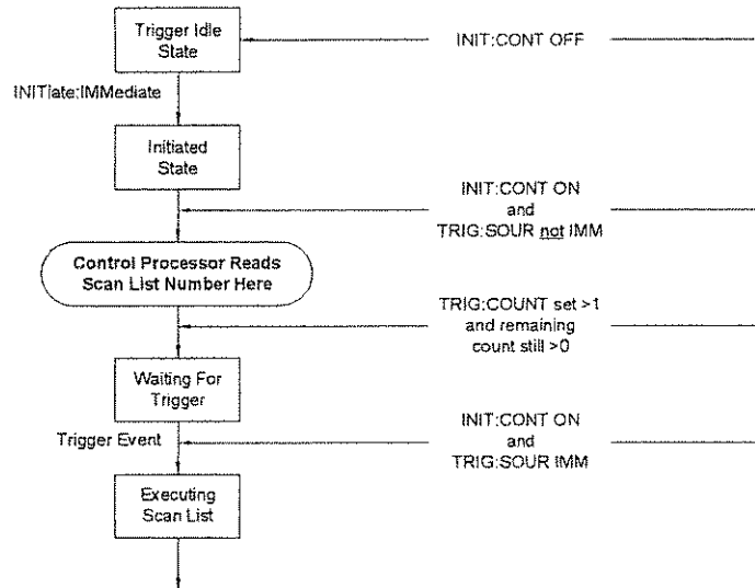
Figure 5-3 Event Sequence for ROUTE:SCAN
