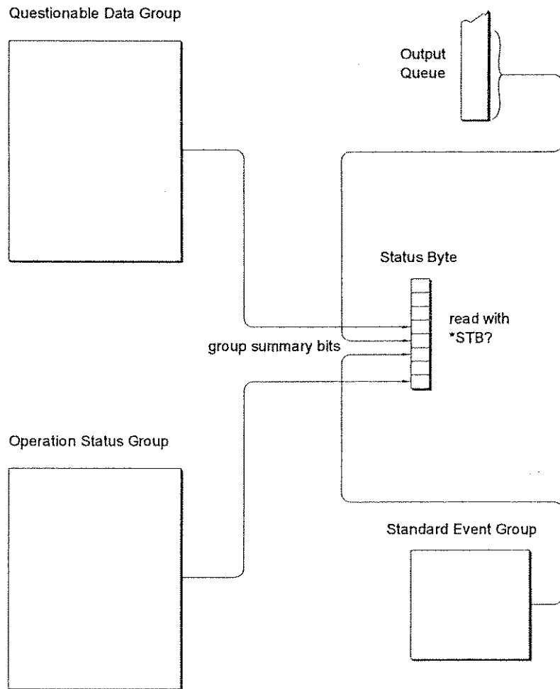
Figure 4-5 Simplified Status System Diagram
