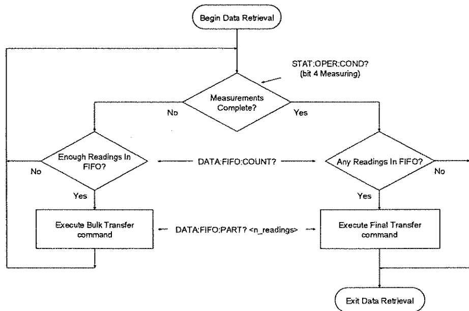
Figure 4-2 Controlling Reading Count
