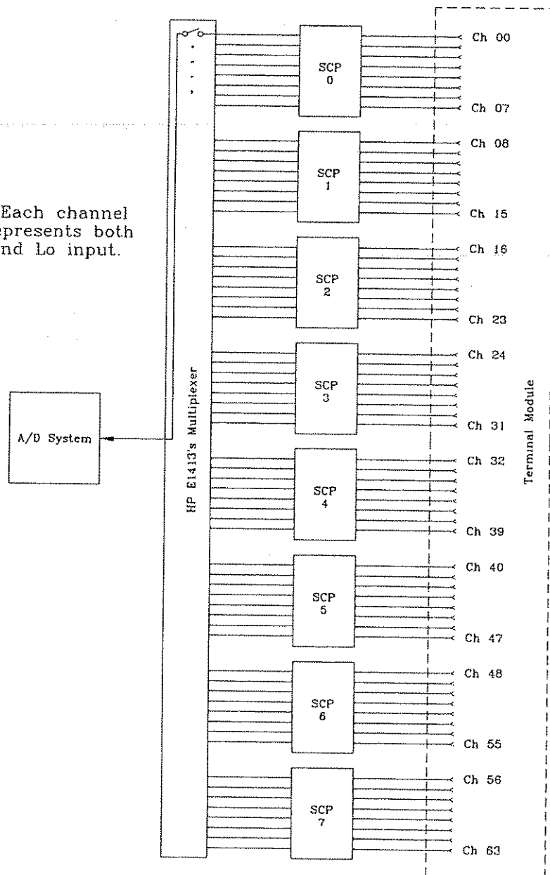
Figure 2-1 Channel Numbers at SCP Positions
