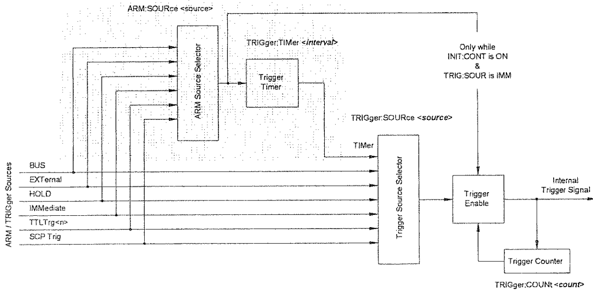
Figure 5-5 Logical Trigger Model
