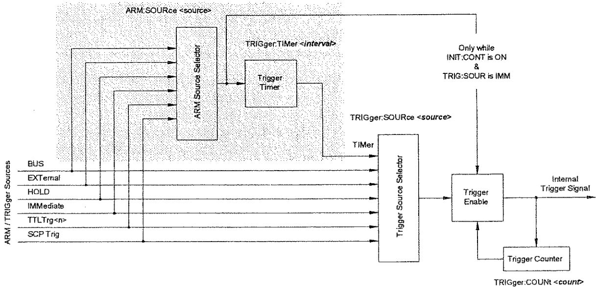
Figure 3-3 Logical Arm and Trigger Model
