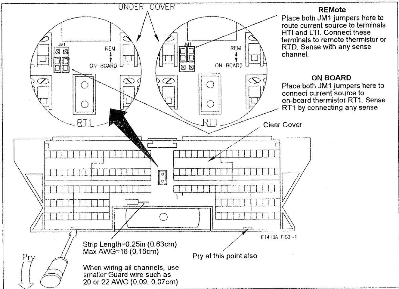
Figure 2-6 The Terminal Module
