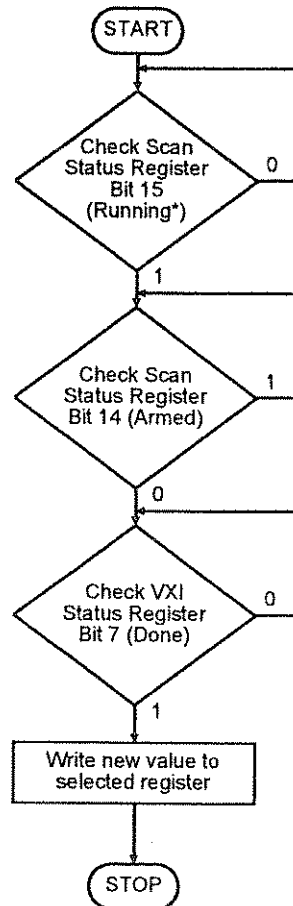
Figure D-4. General Register Access
