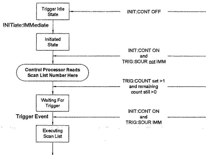
Figure 3-2 Event Sequence for ROUTe:SCAN
