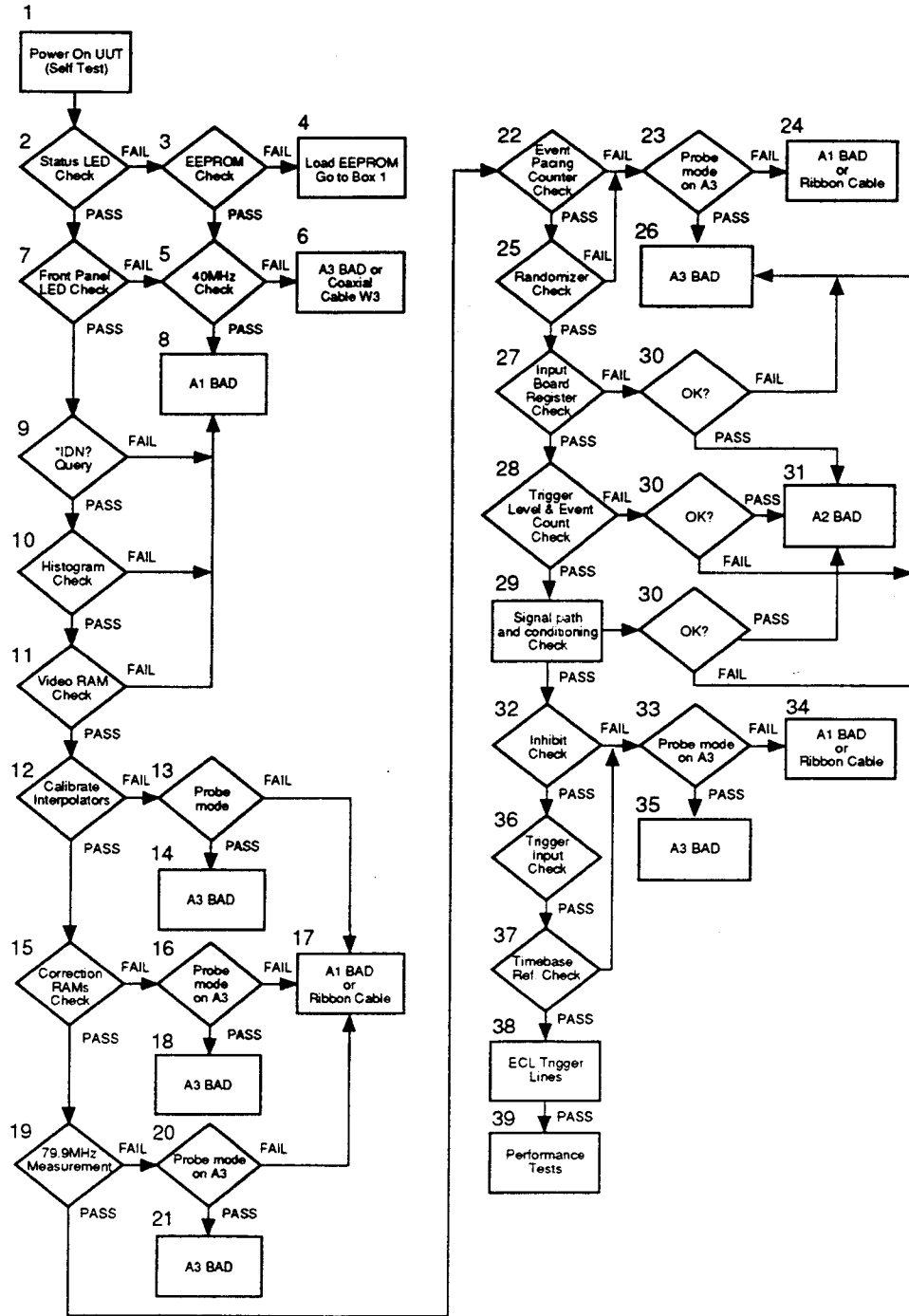
Figure 16-1. E1740A Troubleshooting Flowchart
