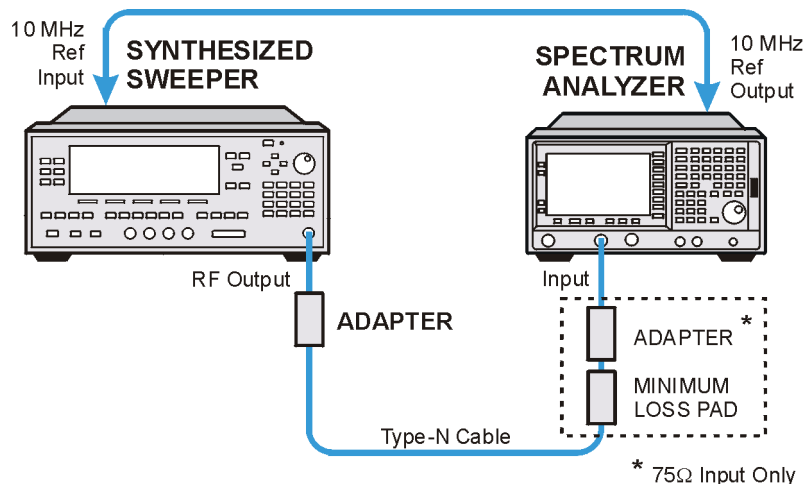
Figure 4-2 Equipment Setup
