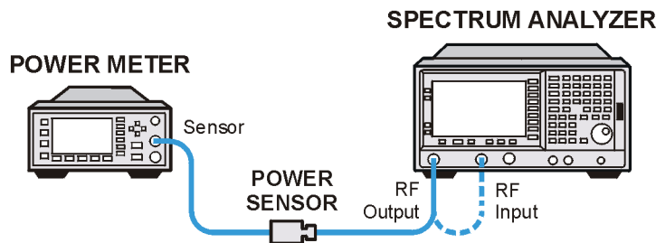
Figure 4-8 Equipment Setup
