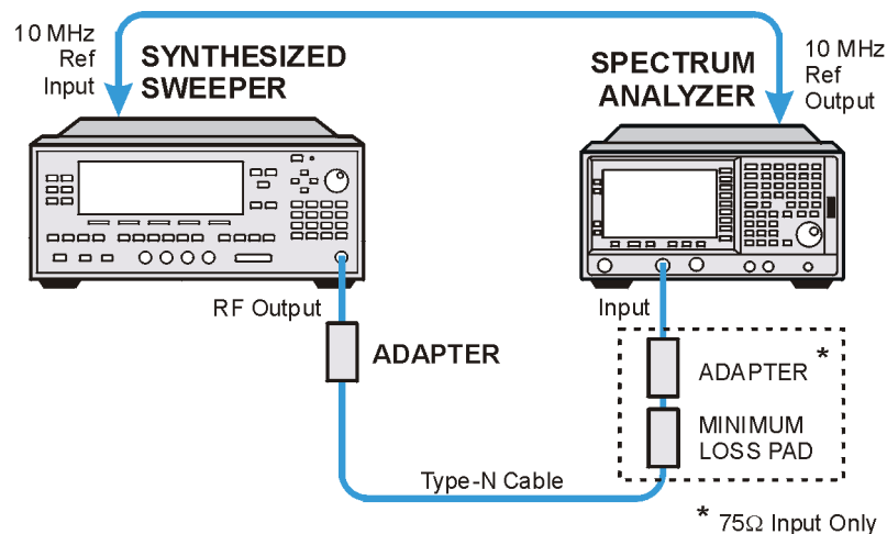
Figure 4-4 Equipment Setup
