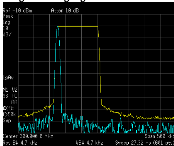
Viewing a Drifting Signal With Max Hold and Clear Write
