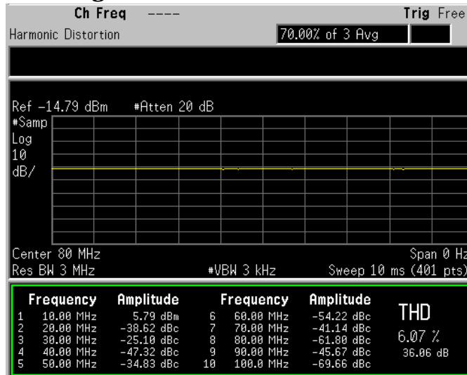
Figure 6-6 Measuring the Harmonic Distortion
