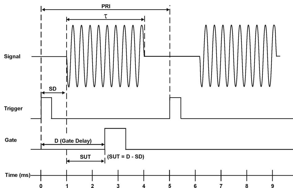
Figure 15-15 Time-domain Parameters
