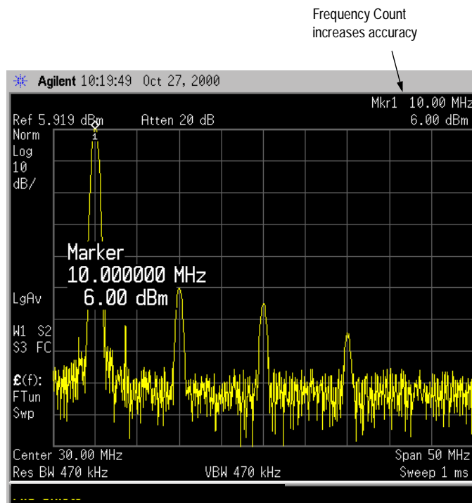
Figure 3-5 Increasing Marker Frequency Accuracy
