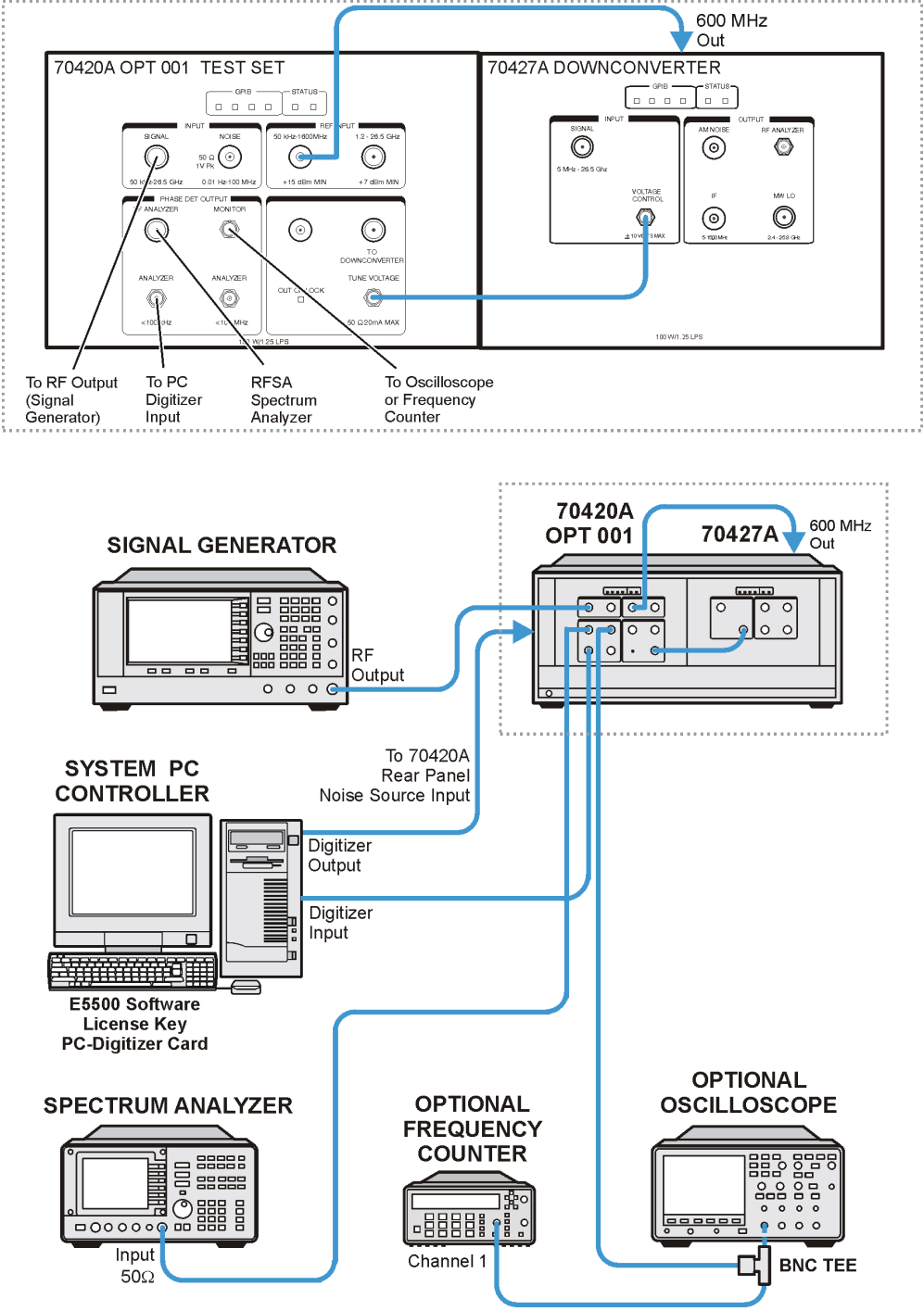
Figure 3-27 Setup with a Carrier Frequency of 600 MHz from the 70427A Reference Source
