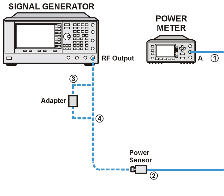
Figure 4-6 Setup for AM Audio Path Offset Calibration
