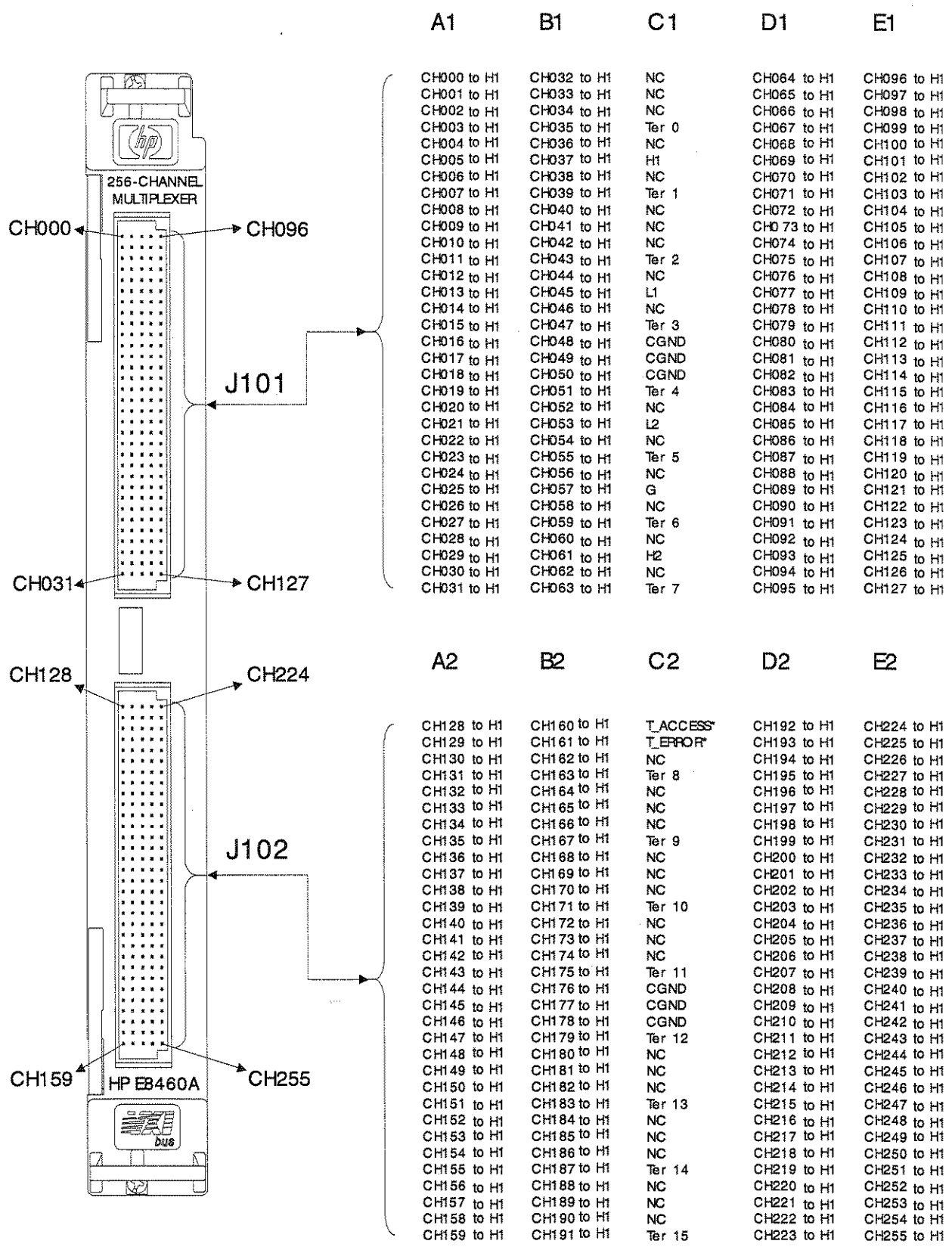
Figure 1-6. HP E8460A Multiplexer Front Panel Pin-out 1-Wire Mode, (Default)
