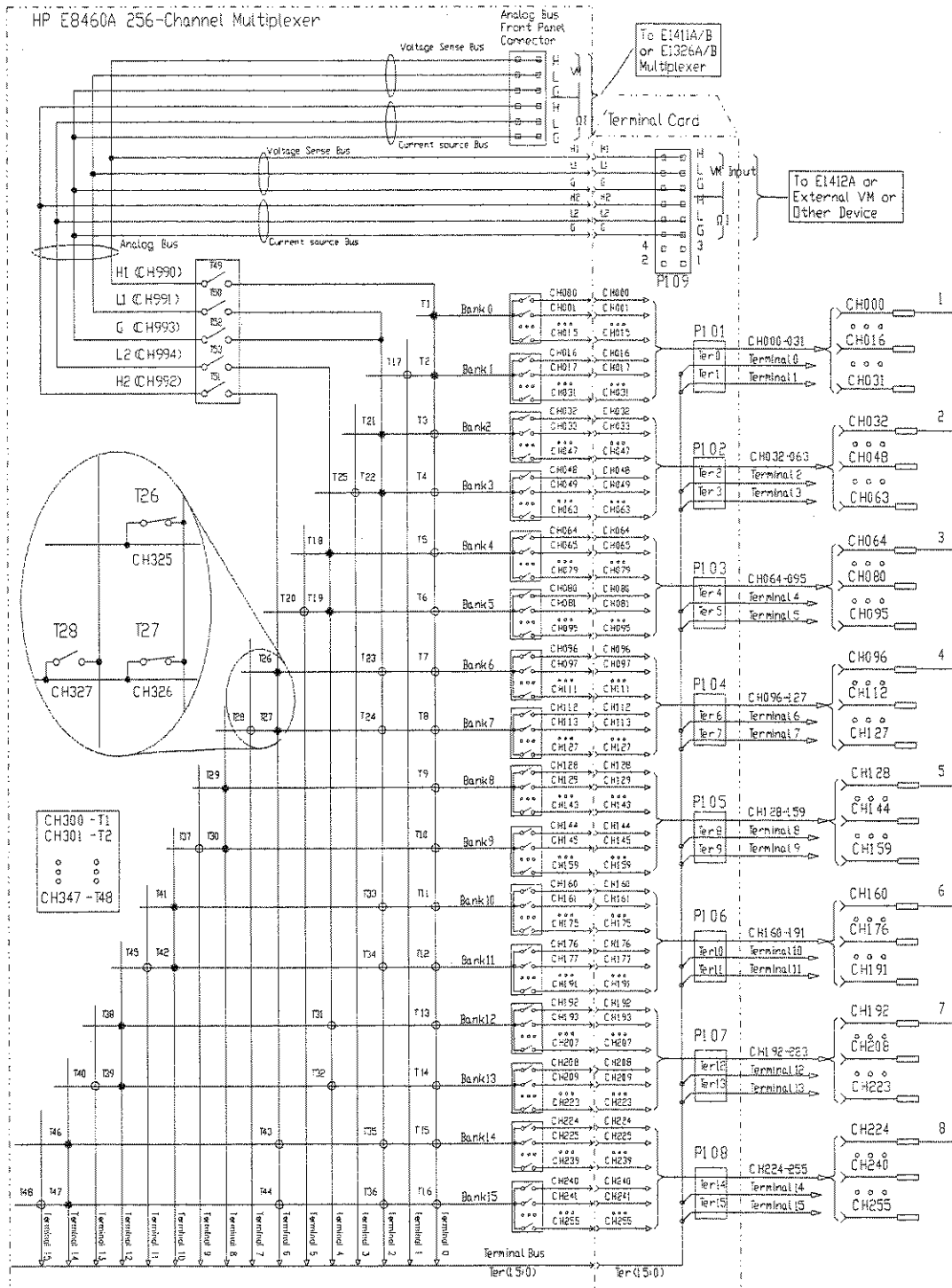
Figure 2-5. Eight 32 x 1 Multiplexer
