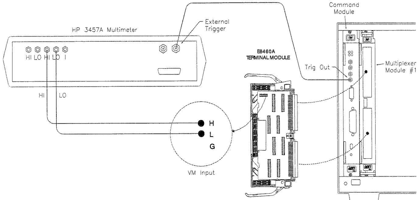
Figure 2-9. Scanning with an External Device
