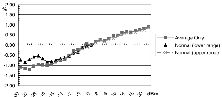
Figure 5 Typical Power Linearity at 25^{\circ}\text{C} for E9323A and E9327A 5 MHz bandwidth sensors after zero and calibration, with associated measurement uncertainty
