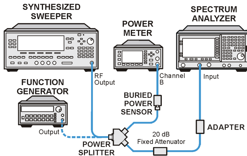
Figure 2-41 Frequency Response Test Setup, Preamp On
