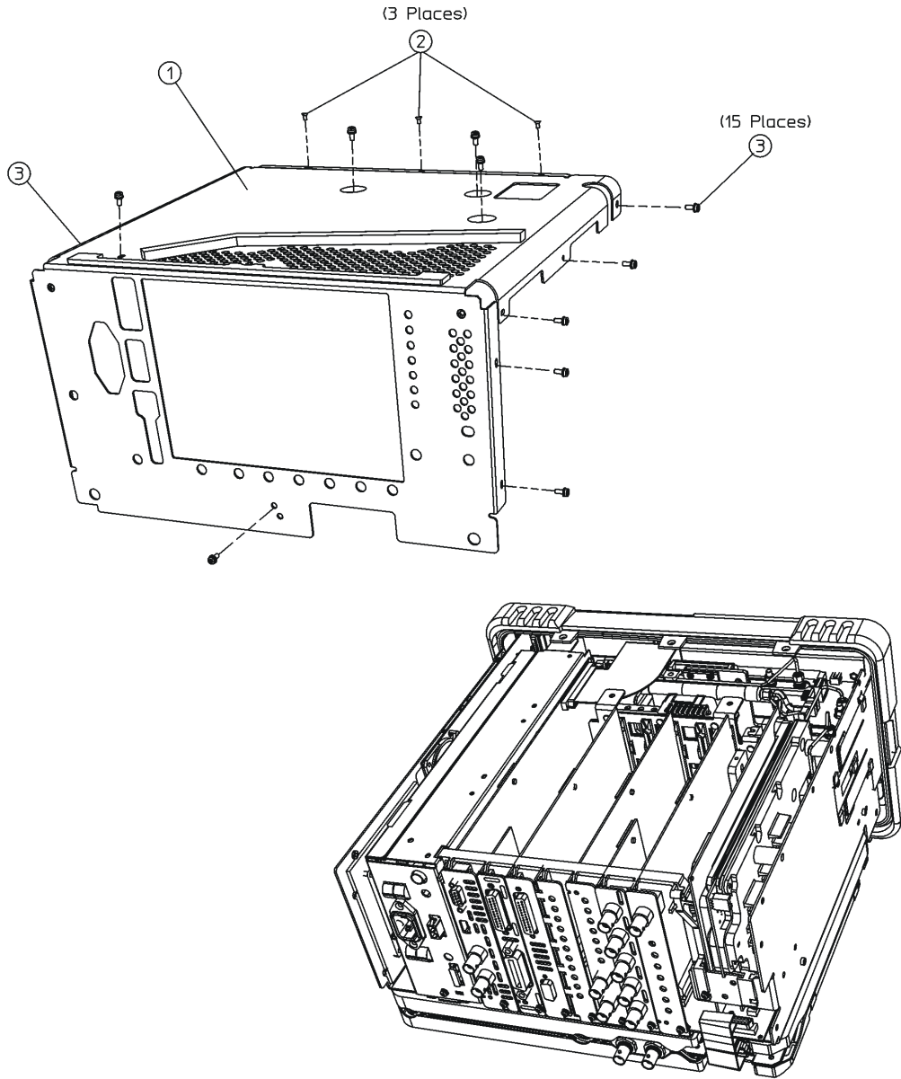
Figure 2. Remove Chassis Cover
