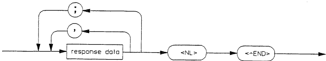
Figure 4-4. Simplified Response Message Syntax
