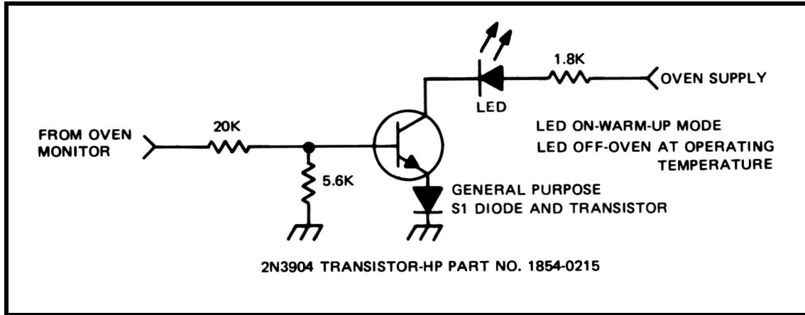
Figure 2-2. Oven Monitor LED Circuit
