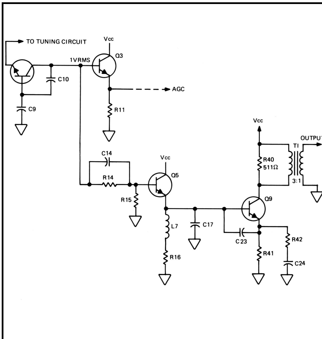
Figure 8-8. Output Amplifiers
