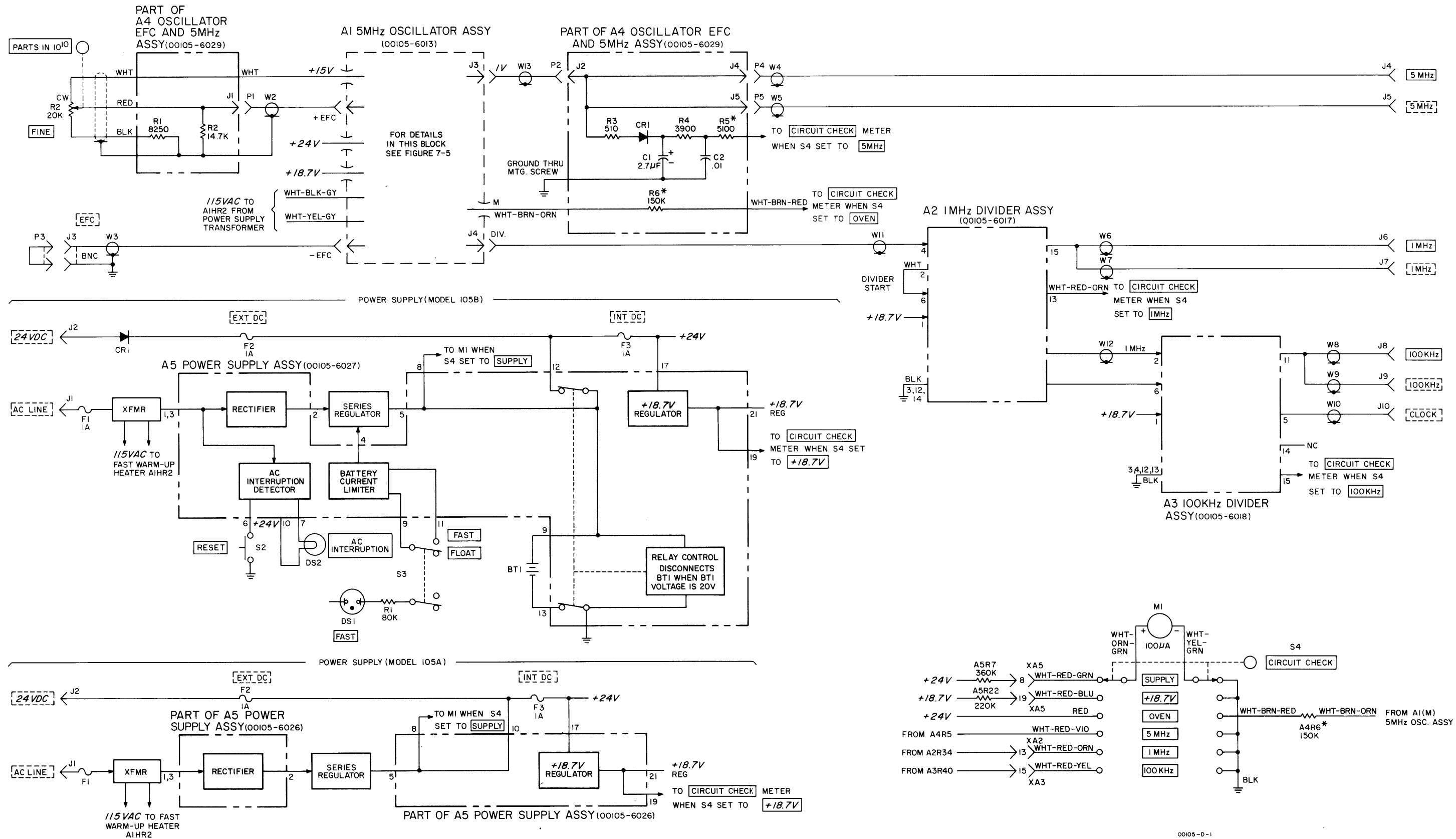
Figure 7-2. Block Diagram
