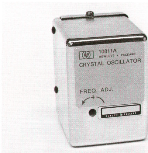
Fig. 1. The new 10811A/B 10-MHz Crystal Oscillator is a component oscillator for instruments and systems. A new quartz crystal cut and a new circuit design give it many improved features including lower phase noise and lower power consumption than previous designs. Two models, A and B, provide a choice of electrical connection methods.
