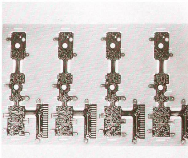
Fig. 2. Flex circuits come five to a panel and are loaded, soldered, and tested before being separated.
