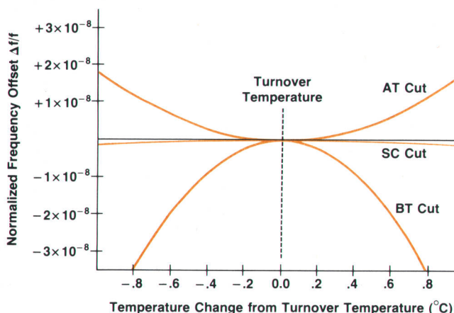
Fig. 1. Comparing the SC-cut crystal's temperature performance with that of two other common cuts, AT and BT.
