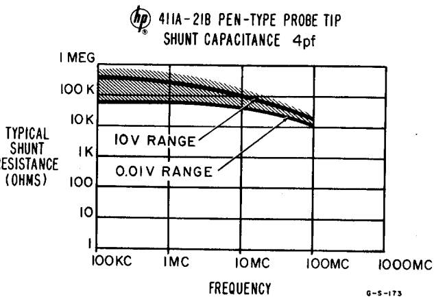
Figure 3-5. Input Impedance of Pen-Type Probe Tip
