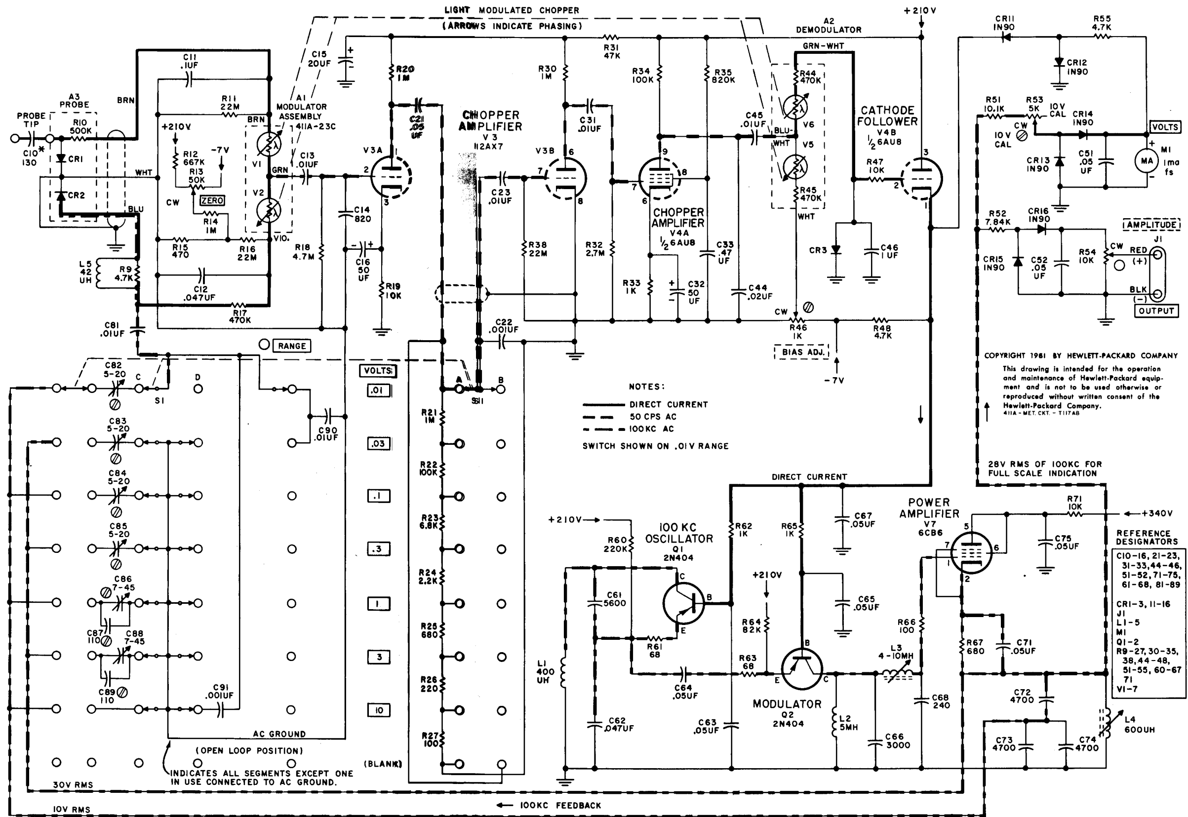
Figure 5-7. Voltmeter 5-11/5-12
