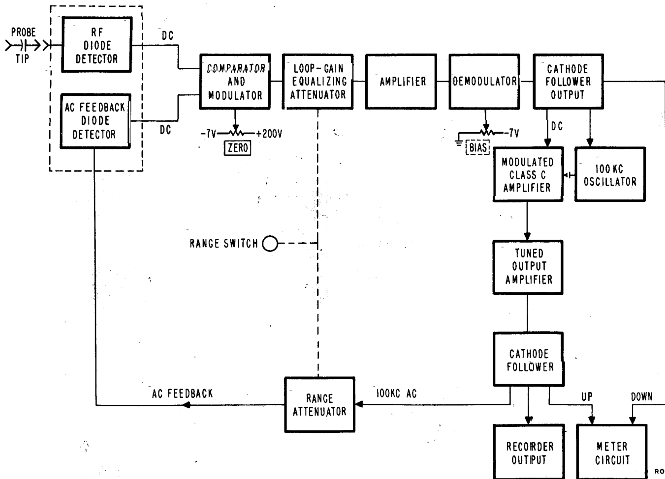
Figure 4-1. Block Diagram
