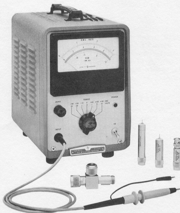
Figure 1-1. Model 411A RF Millivoltmeter
