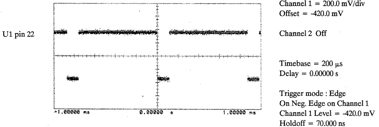
Figure 6C-18. Test Loop 21 Troubleshooting Waveform on the Horizontal Assembly
