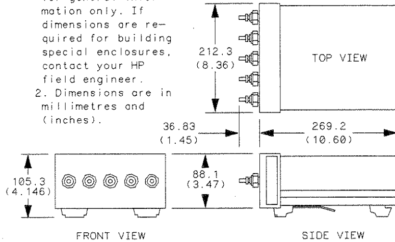
Figure 1-1. HP 54121A Dimensions
