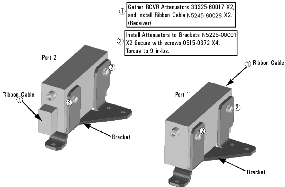
Figure 1 Port 1 and Port 2 Receiver Attenuator and Bracket Assembly
