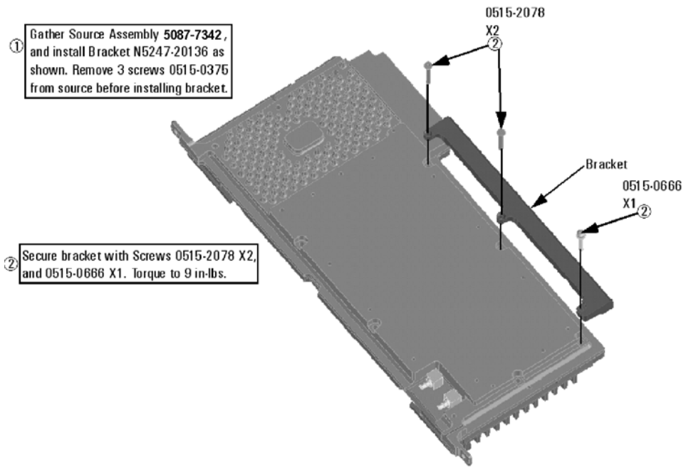
Figure 16 A10 Source 2 Assembly Bracket Installation
