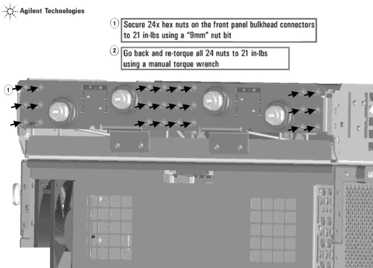
Figure 23 Bulkhead Connections, Front Panel
