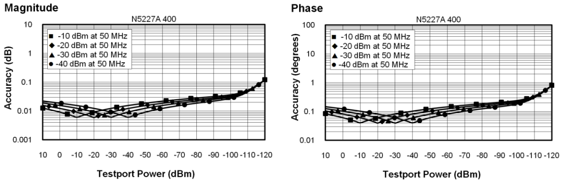
N5227A Dynamic Accuracy, 50 MHz - Specification
