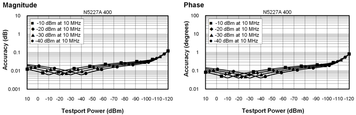
N5227A Dynamic Accuracy, 10 MHz - Specification
