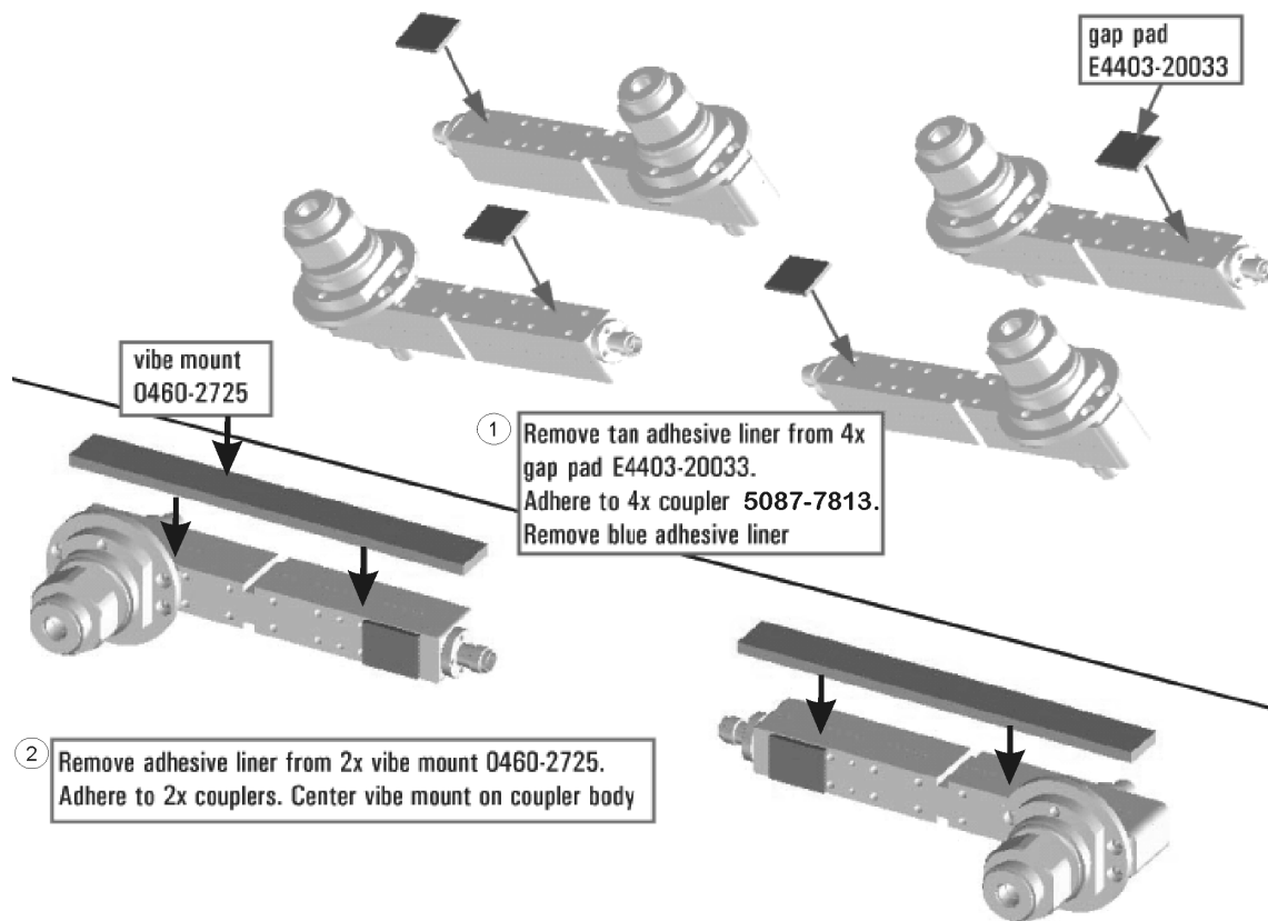
Figure 10 A29 - A32 Test Port Coupler Assembly
