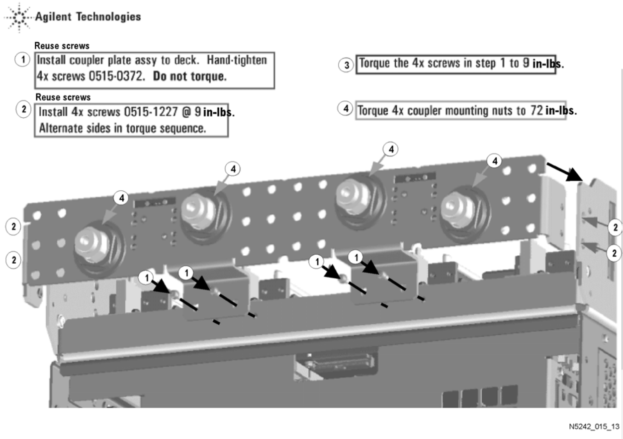
Figure 8 Coupler Plate Assembly Installation
