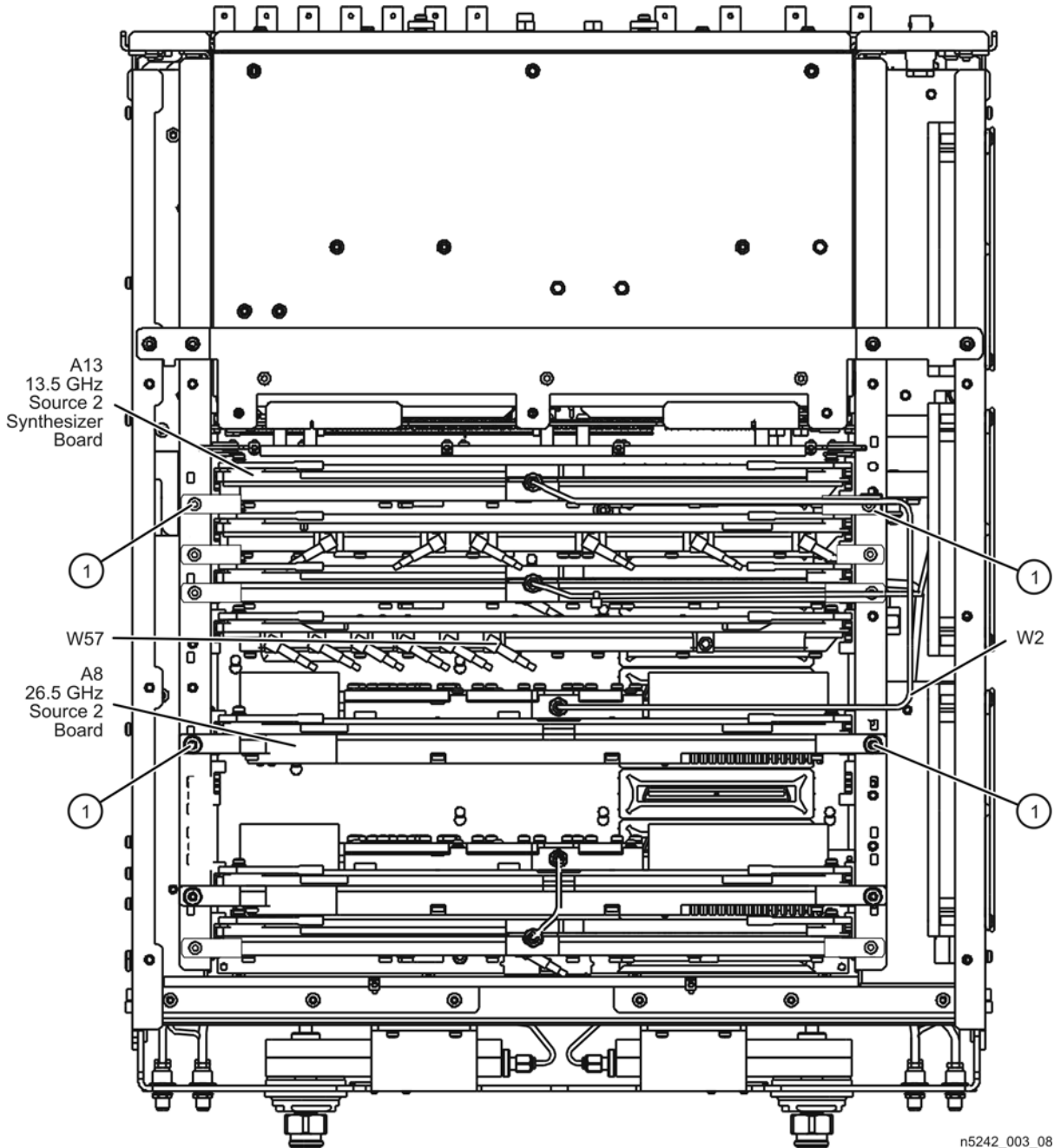
Figure 9-2 Second Source Boards Installation
