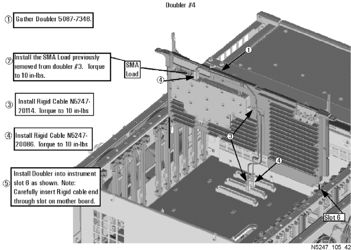
Figure 8 A13 40 GHz Doubler 4 Installation
