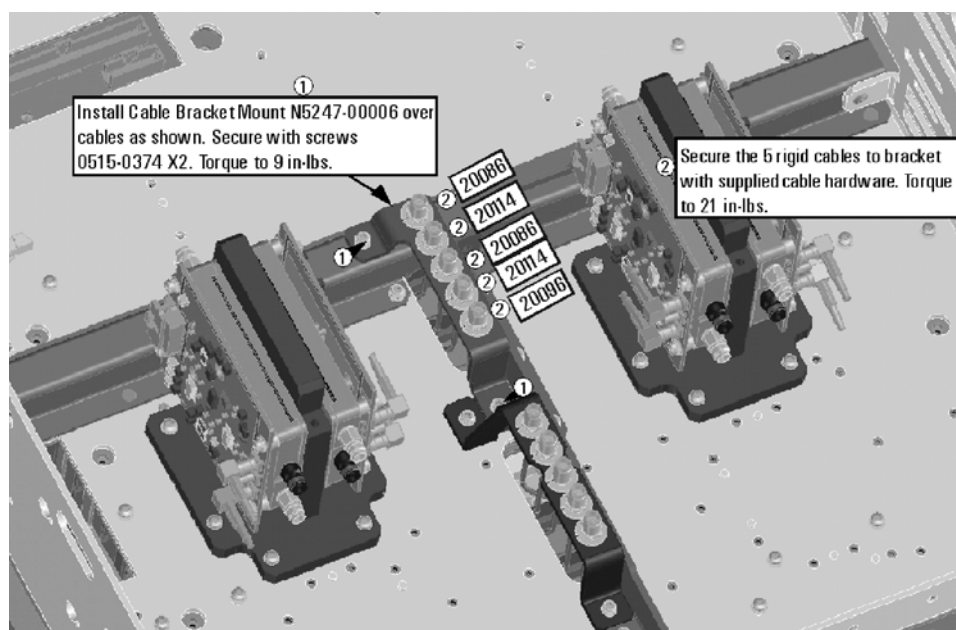
Figure 13 Cable Bracket Mount Installation
