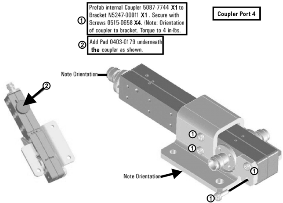
Figure 18 A31 Reference Coupler Assembly
