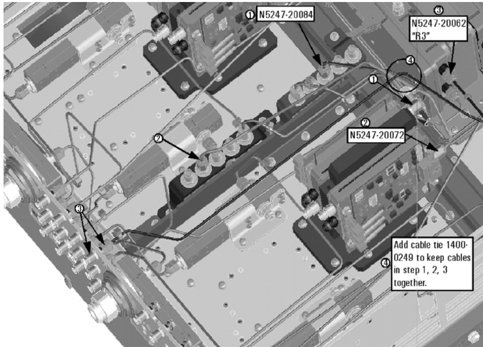
Figure 27 Location of Cable Tie to Secure W14, W18, and W54 Together
