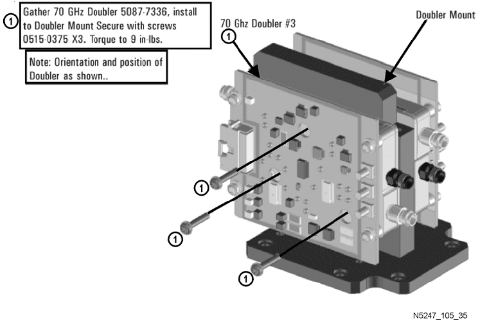
Figure 2 Installing A61 Doubler 3 on the Doubler Mount
