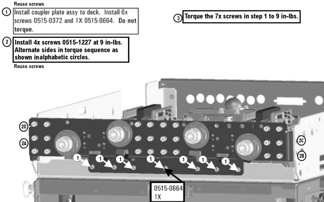
Figure 22 Coupler Plate Assembly Installation
