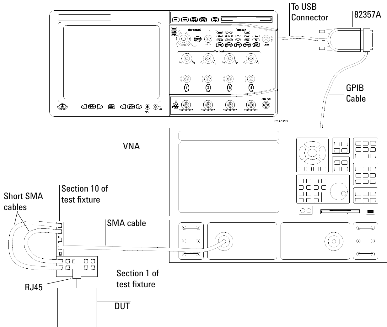
Figure 41 Probing for 10 Base-T Transmitter Return Loss
