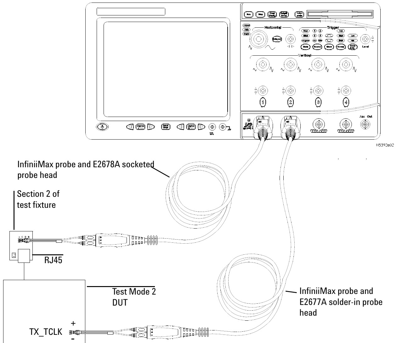
Figure 17 Probing for 1000 Base-T MASTER JTxOut
