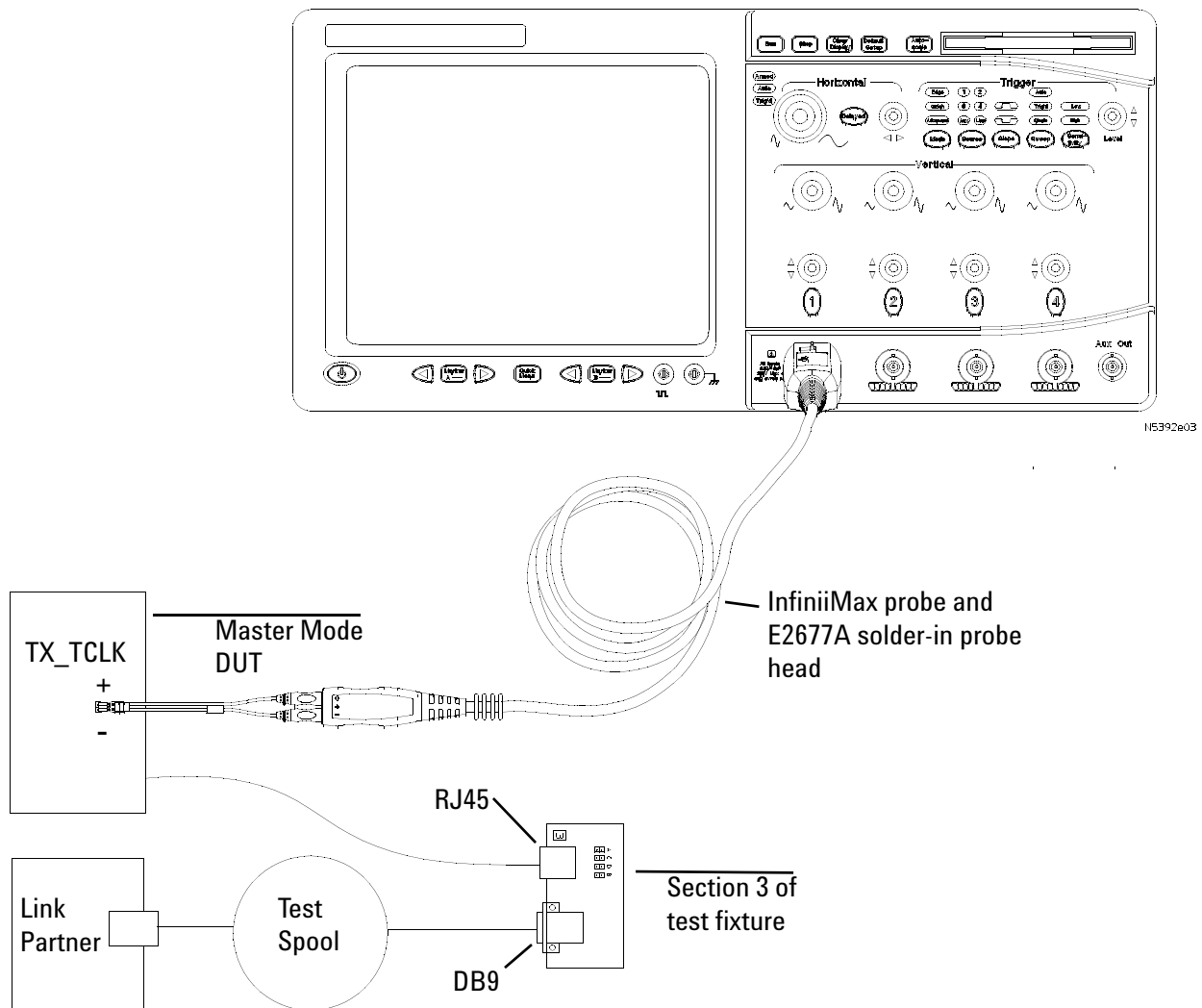
Figure 18 Probing for 1000 Base-T MASTER TX_TCLK Jitter (Filtered and Unfiltered)
