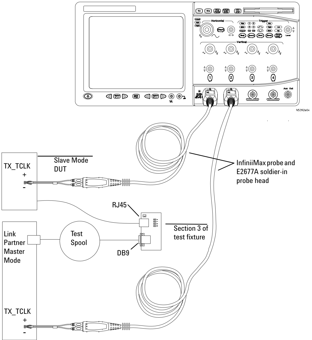
Figure 20 Probing for 1000 Base-T SLAVE TX_TCLK Jitter (Filtered and Unfiltered)
