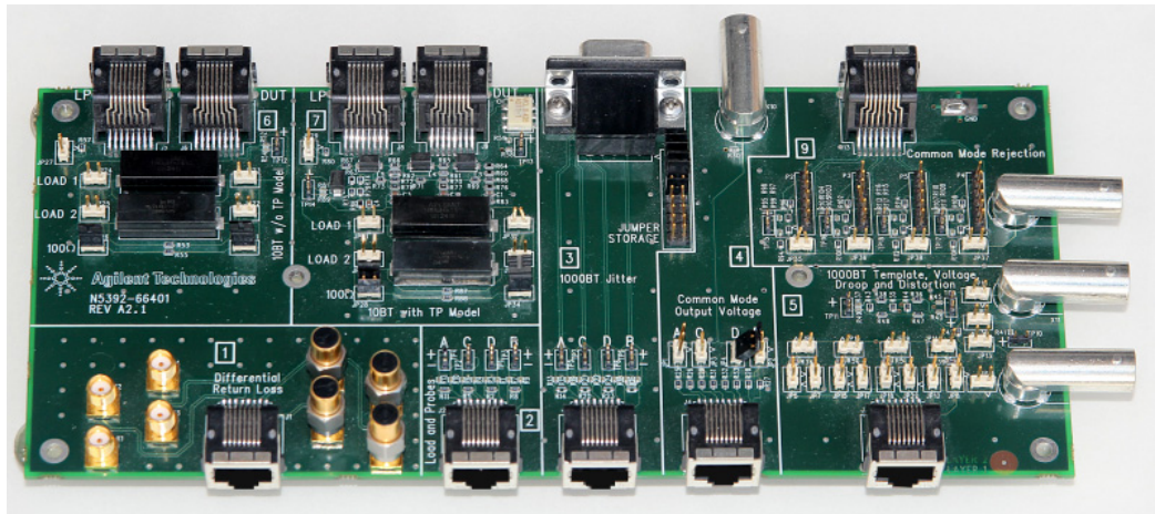
Figure 1 N5395A Ethernet Electrical Compliance Test Board - N5392-66401
