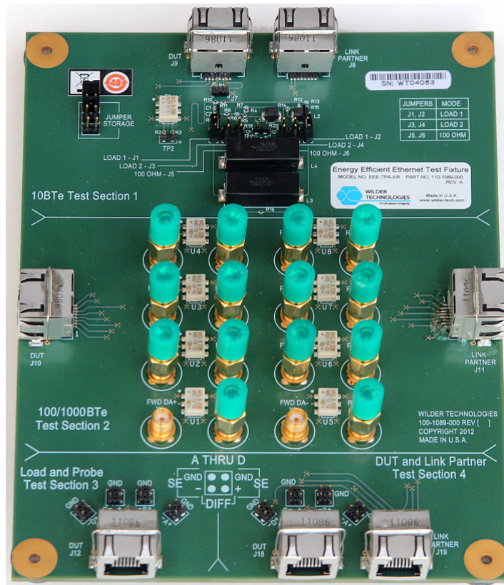
Figure 4 Wilder Technologies EEE Electrical Compliance Test Board
