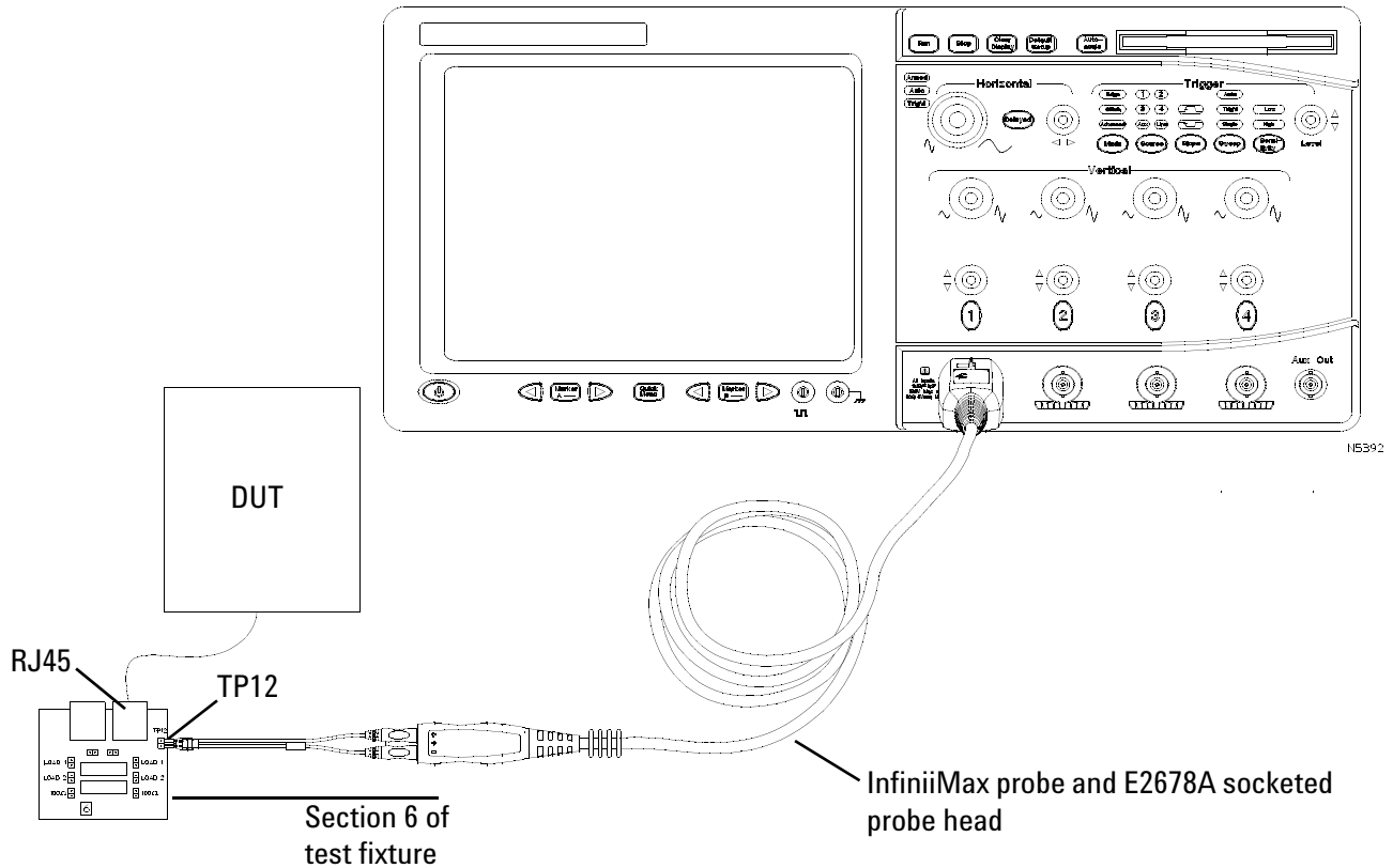
Figure 37 Probing for 10 Base-T Link Test Pulse, Without TPM
