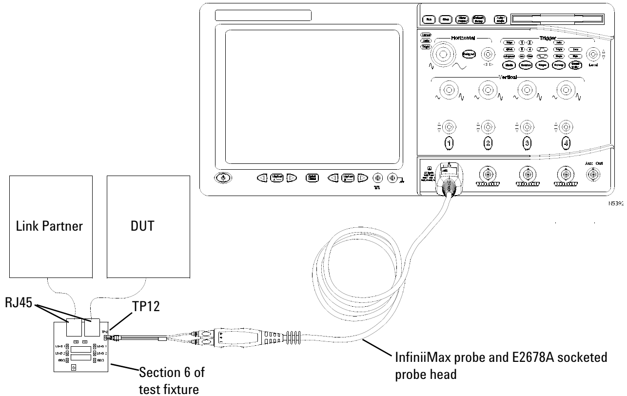
Figure 47 Probing for 10 Base-Tc Tests Without TPM, With Link Partner
