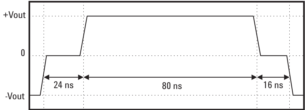
Figure 28 Rise and Falltime Reference Waveform
