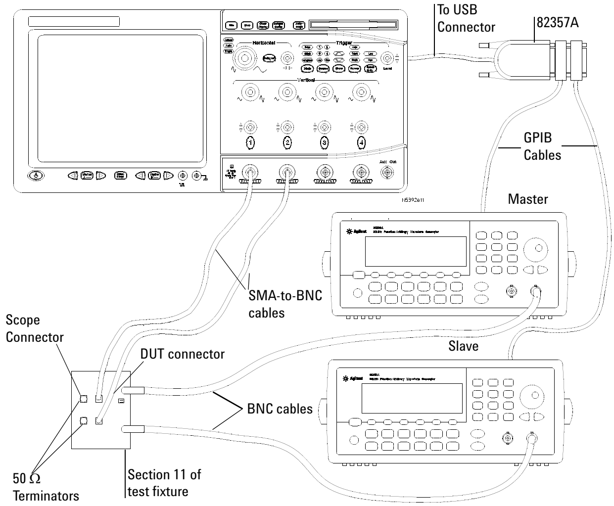
Figure 7 Calibration Setup for the 33250A Disturbing Signal Source
