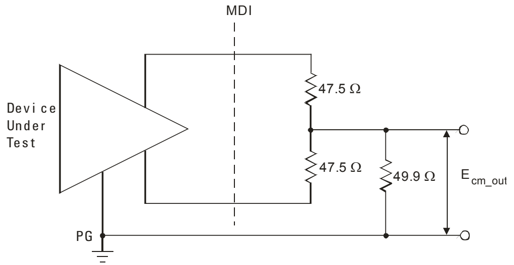
Figure 49 Common Mode Output Voltage Test Circuit
