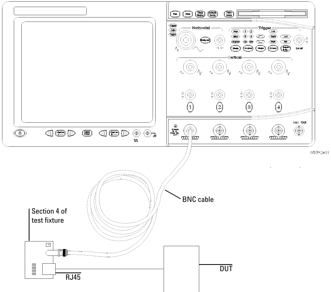
Figure 48 Probing for 10 Base-Tc Common Mode Output Voltage
