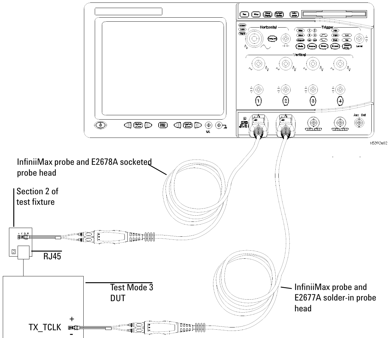
Figure 19 Probing for 1000 Base-T SLAVE JTxOut
