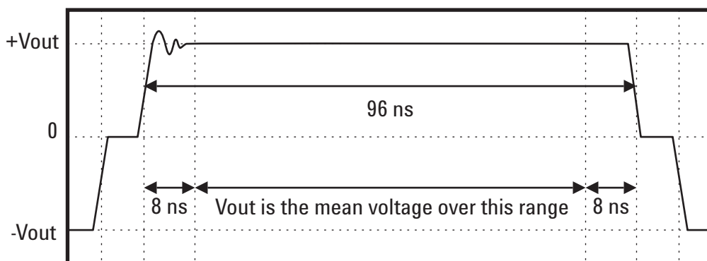
Figure 26 Mean Voltage Over the Time Range
