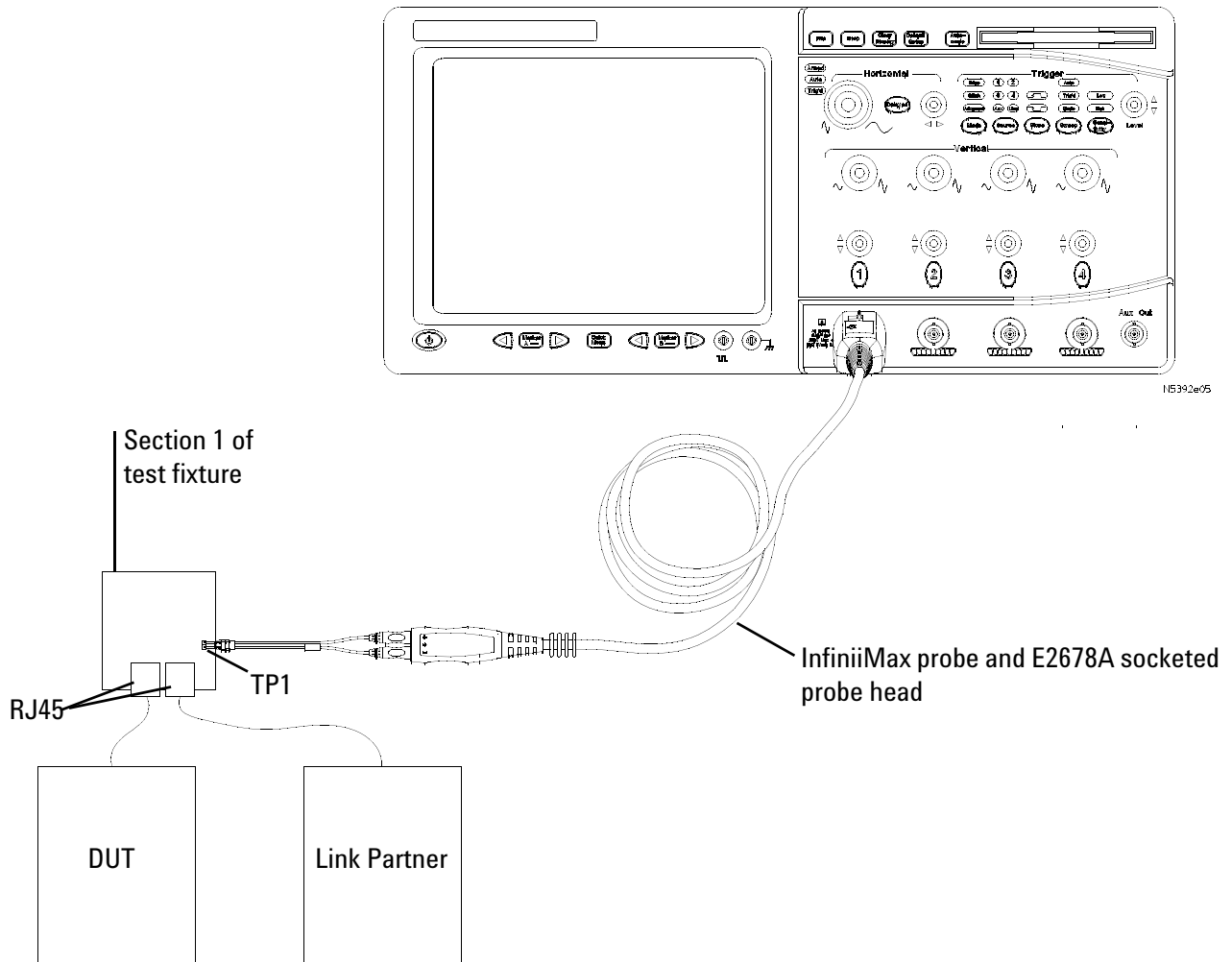
Figure 46 Probing for 10 Base-Te Tests With the TPM and Link Partner
