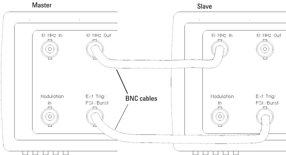
Figure 8 Rear Panel Cable Connections for the 33250A Generators
