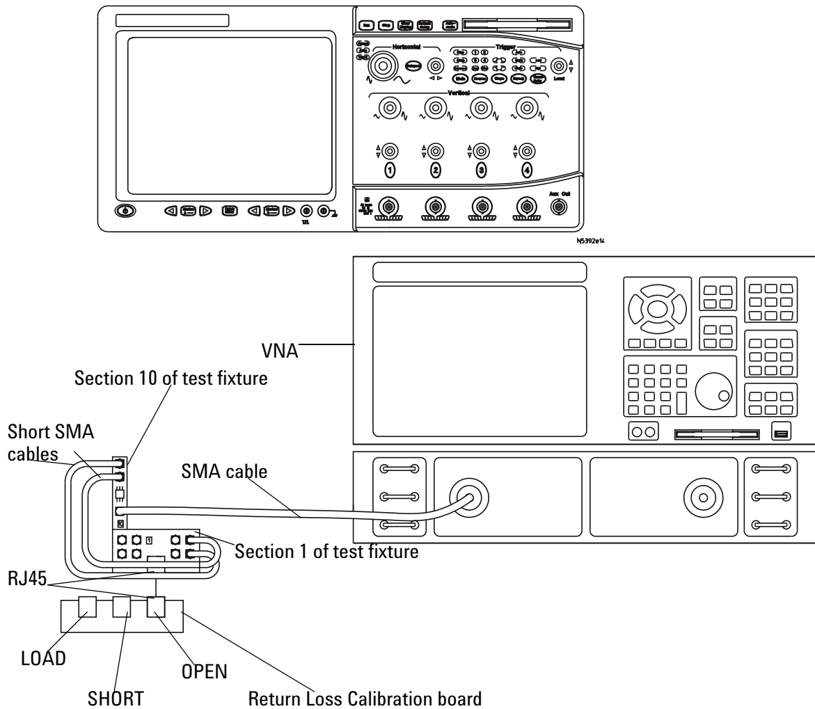
Figure 32 VNA Calibration
