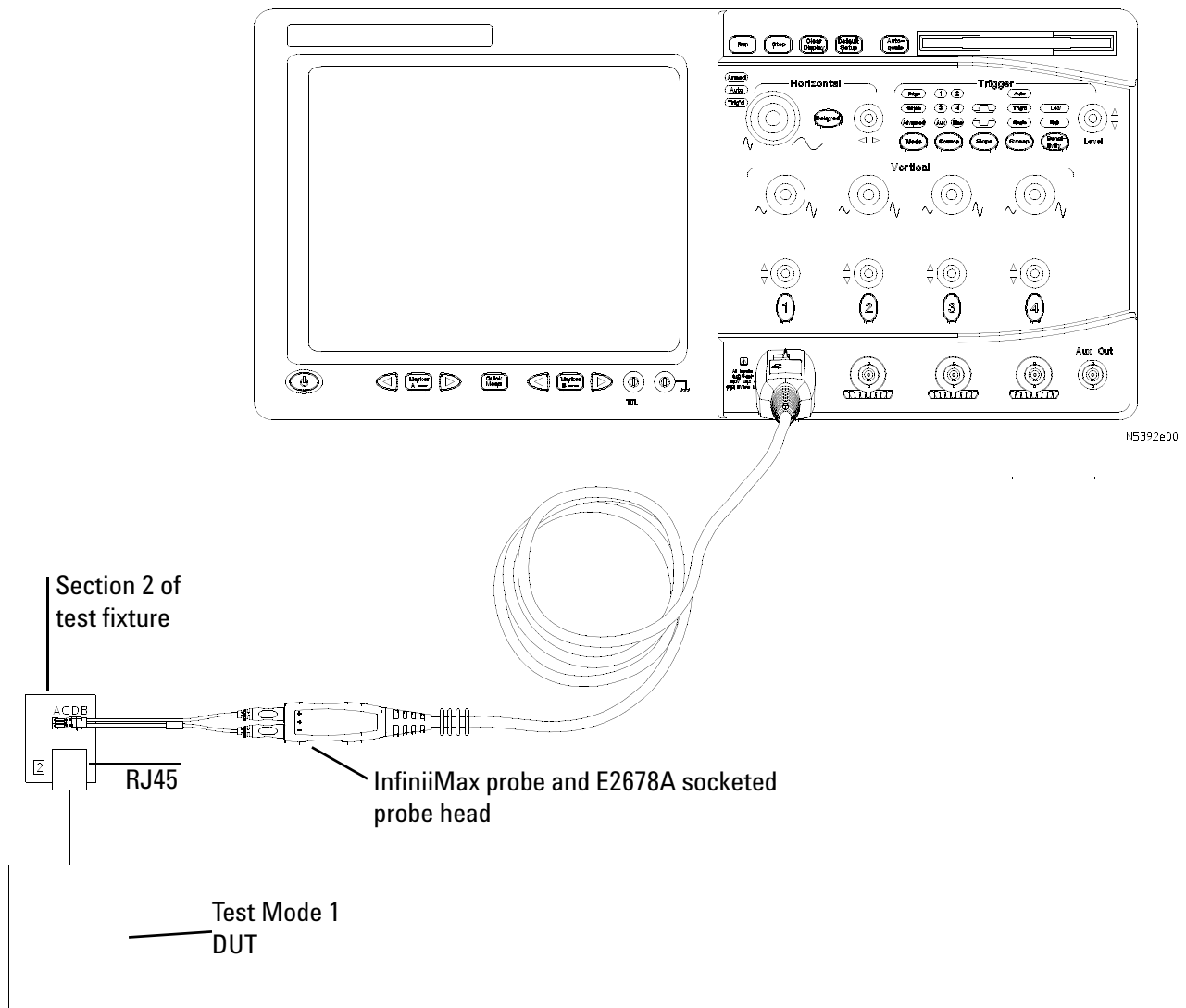
Figure 6 Probing for 1000 Base-T Test Mode 1 Tests
