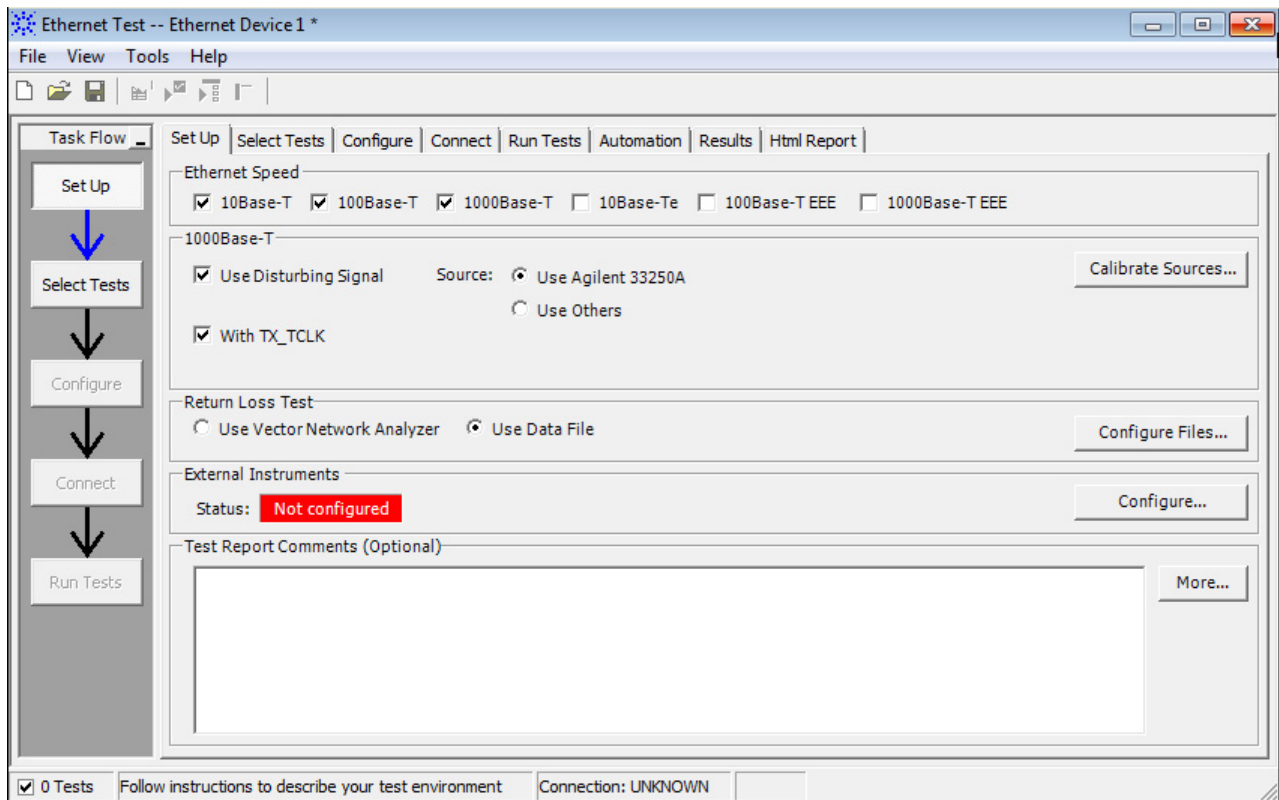
Figure 5 The Ethernet Compliance Test Application
