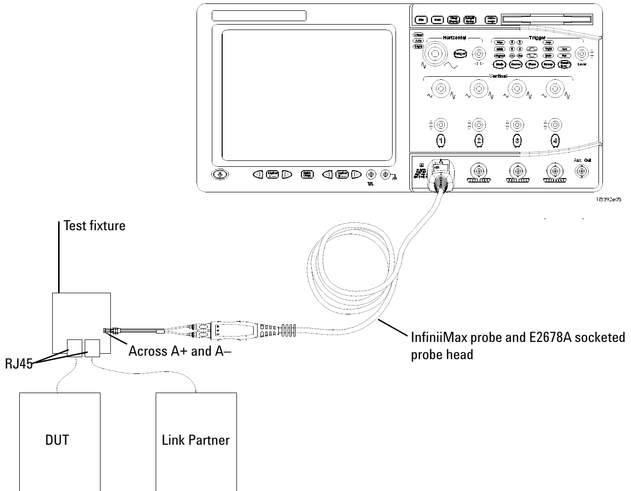
Figure 45 Probing for 100 Base-TX EEE Tests
