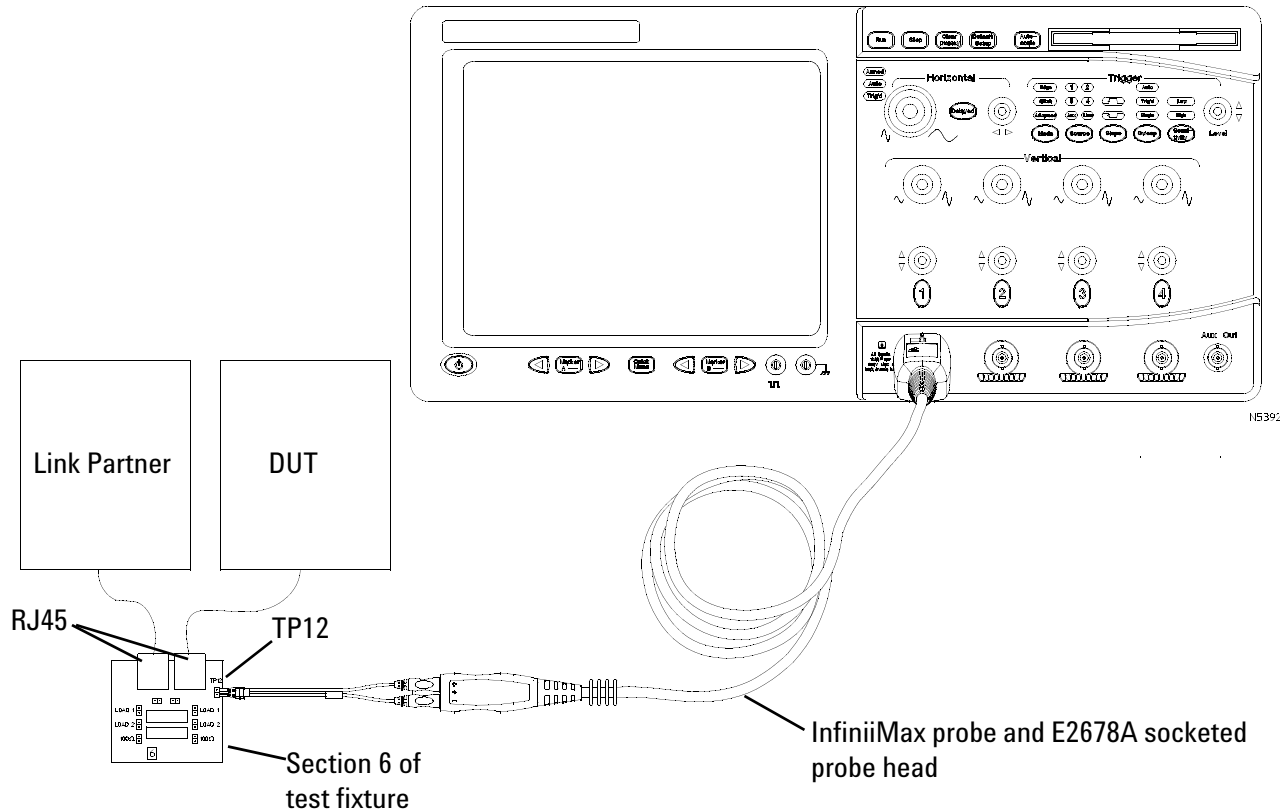
Figure 36 Probing for 10 Base-T Tests Without the TPM, With Link Partner
