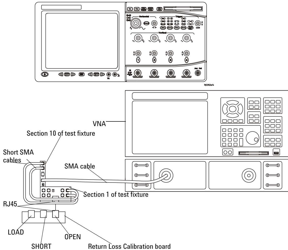
Figure 52 VNA Calibration
