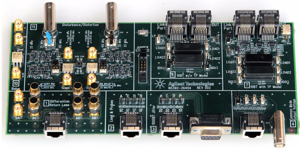
Figure 2 N5395B/N5395C Ethernet Electrical Compliance Test Board
