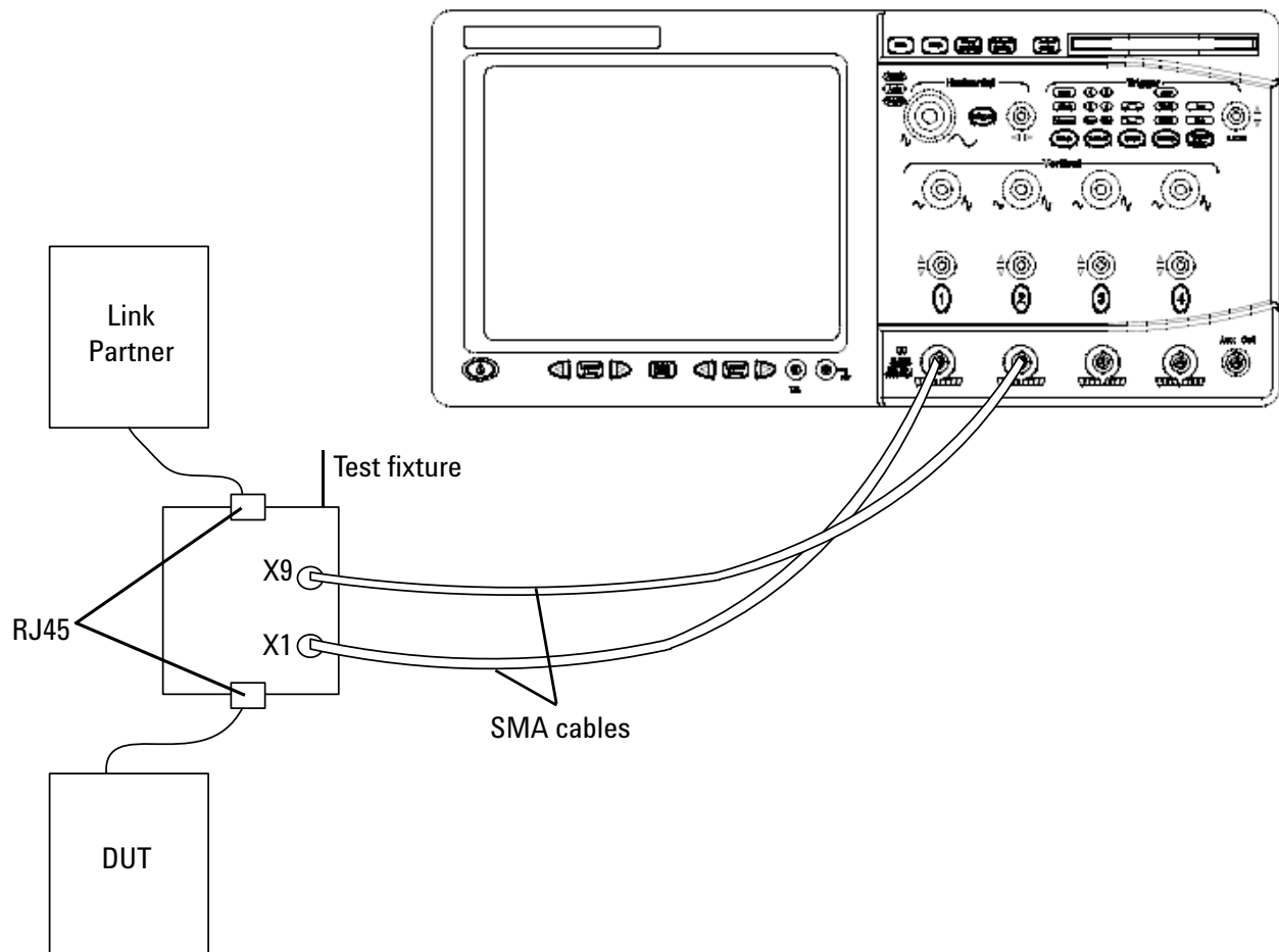
Figure 44 Probing for 1000 Base-T EEE Tests
