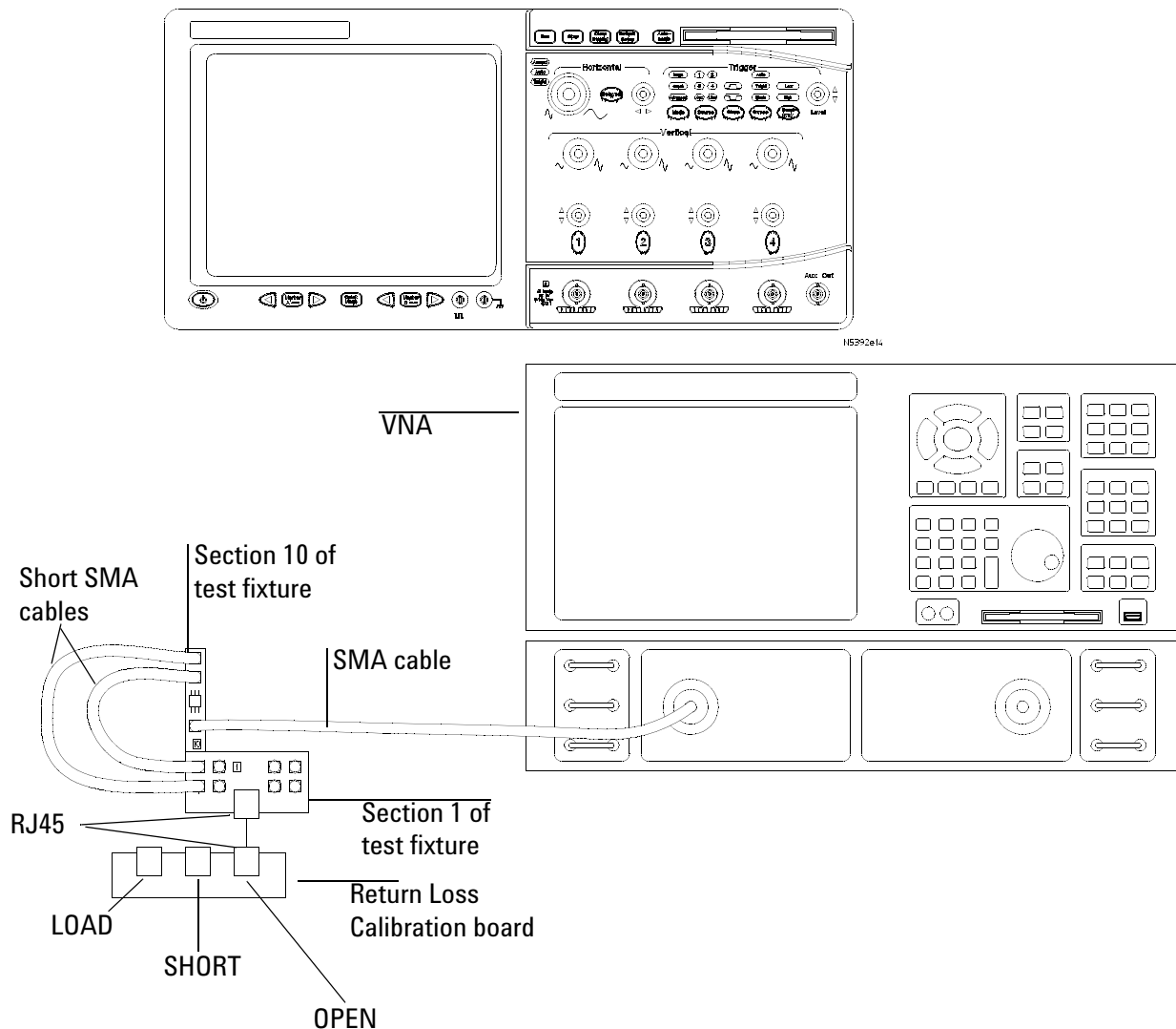
Figure 30 VNA Calibration
