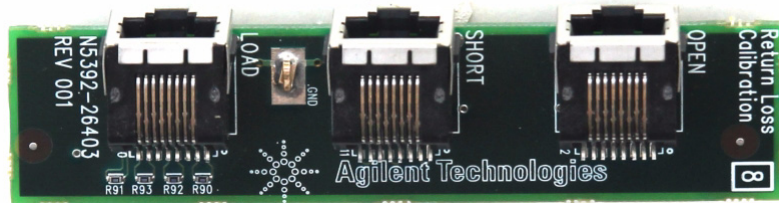
Figure 3 N5395A Ethernet Electrical Compliance Test Board - N5392-66402
