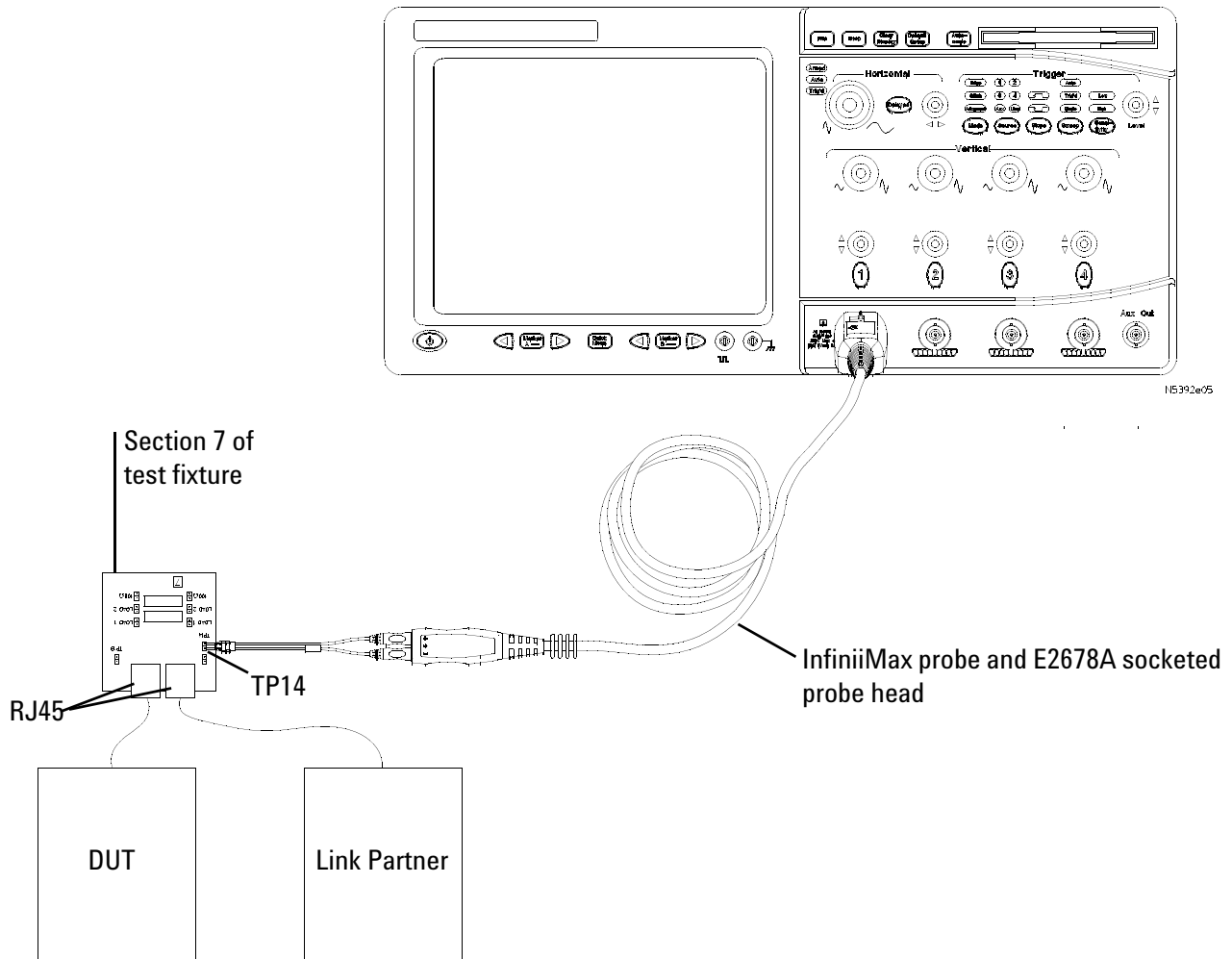
Figure 35 Probing for 10 Base-T Tests With the TPM and Link Partner
