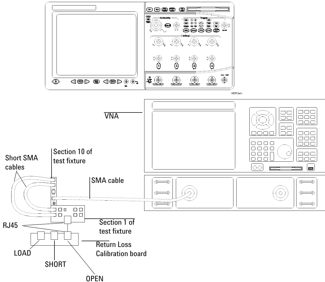
Figure 50 VNA Calibration
