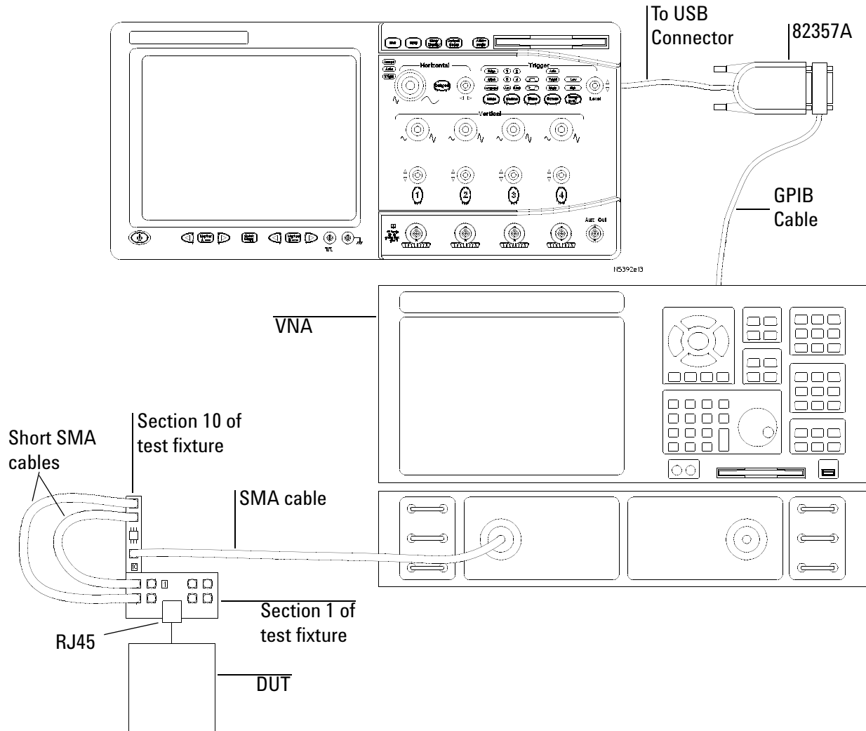
Figure 51 Probing for 10 Base-Tc Transmitter Return Loss
