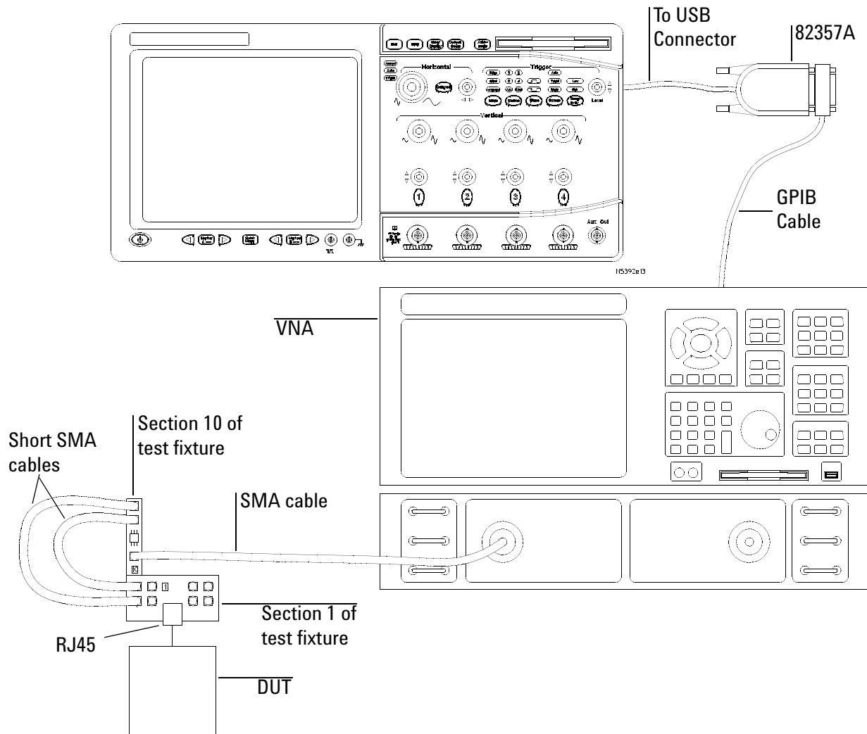
Figure 53 Probing for 10 Base-Te Receiver Return Loss
