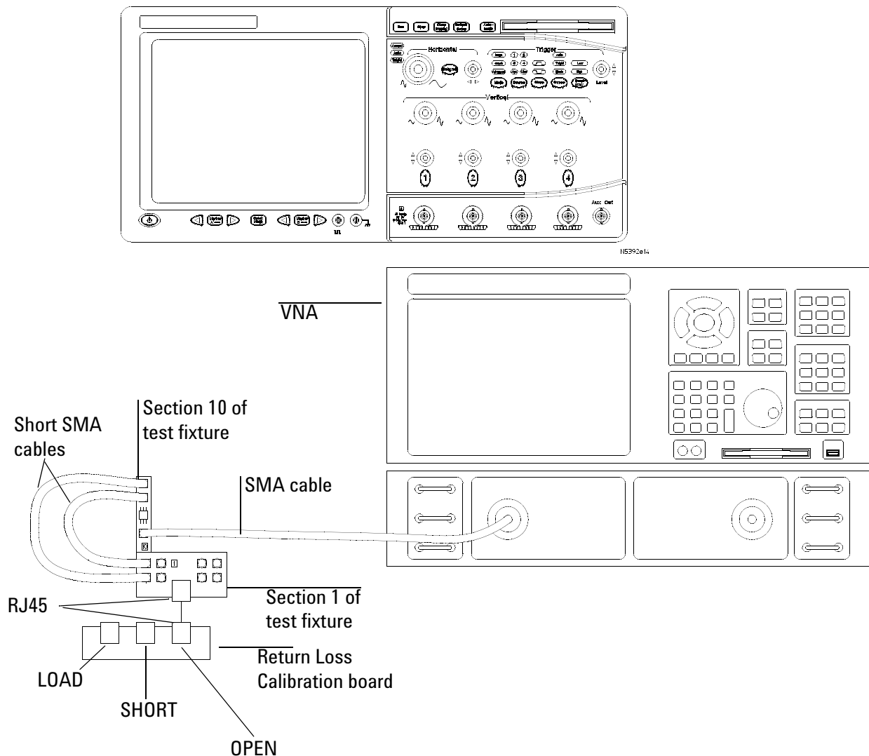
Figure 40 VNA Calibration
