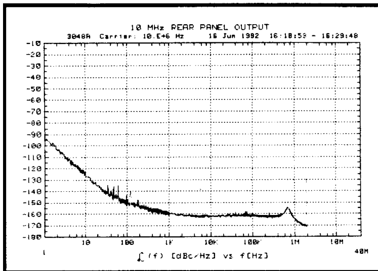
Figure 5 10 MHz output typical performance
