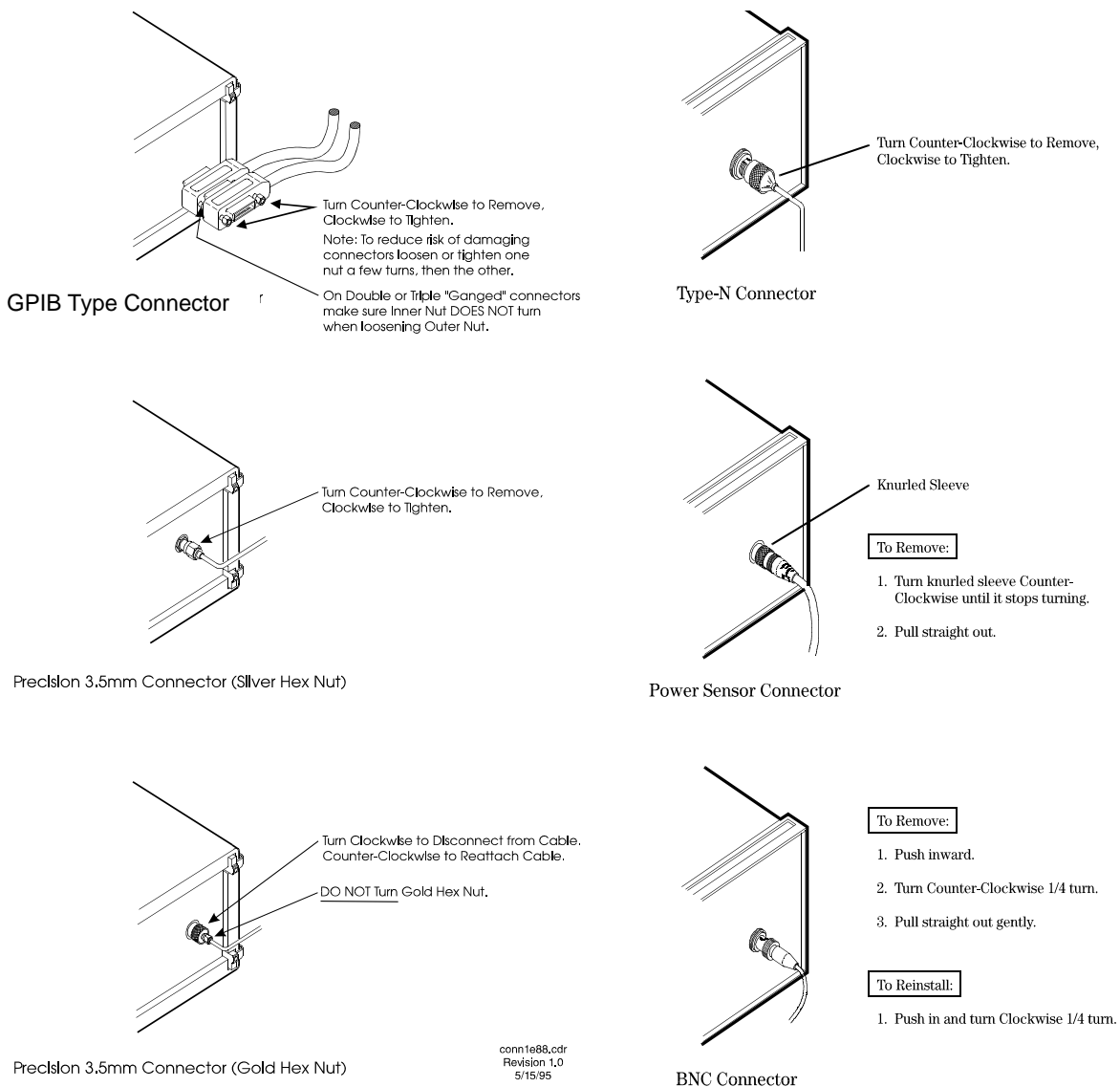
Figure 8 GPIB, 3.5 mm, Type-N, power sensor, and BNC connectors
