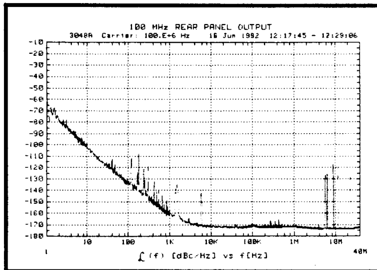
Figure 6 100 MHz output typical performance
