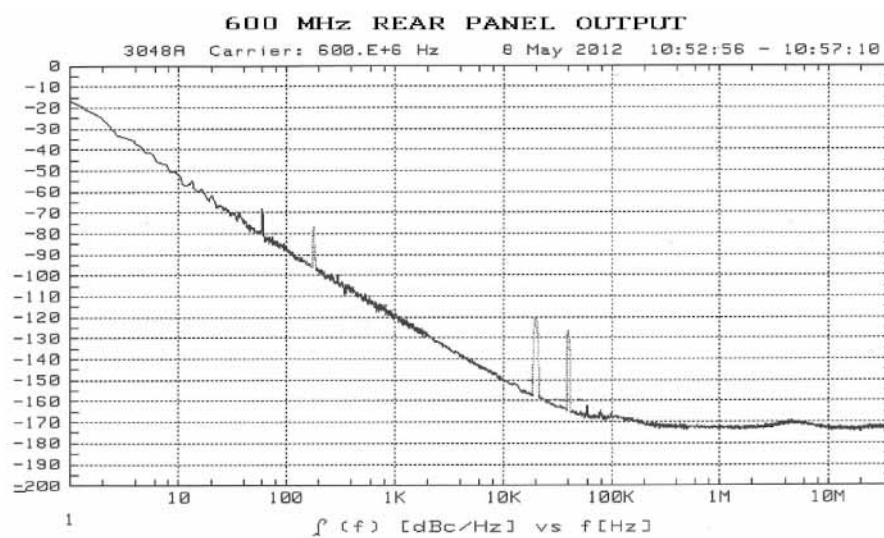
Figure 7 600 MHz output typical performance
