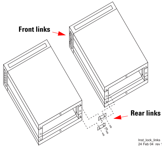
Figure 9 Instrument lock links, front and rear
