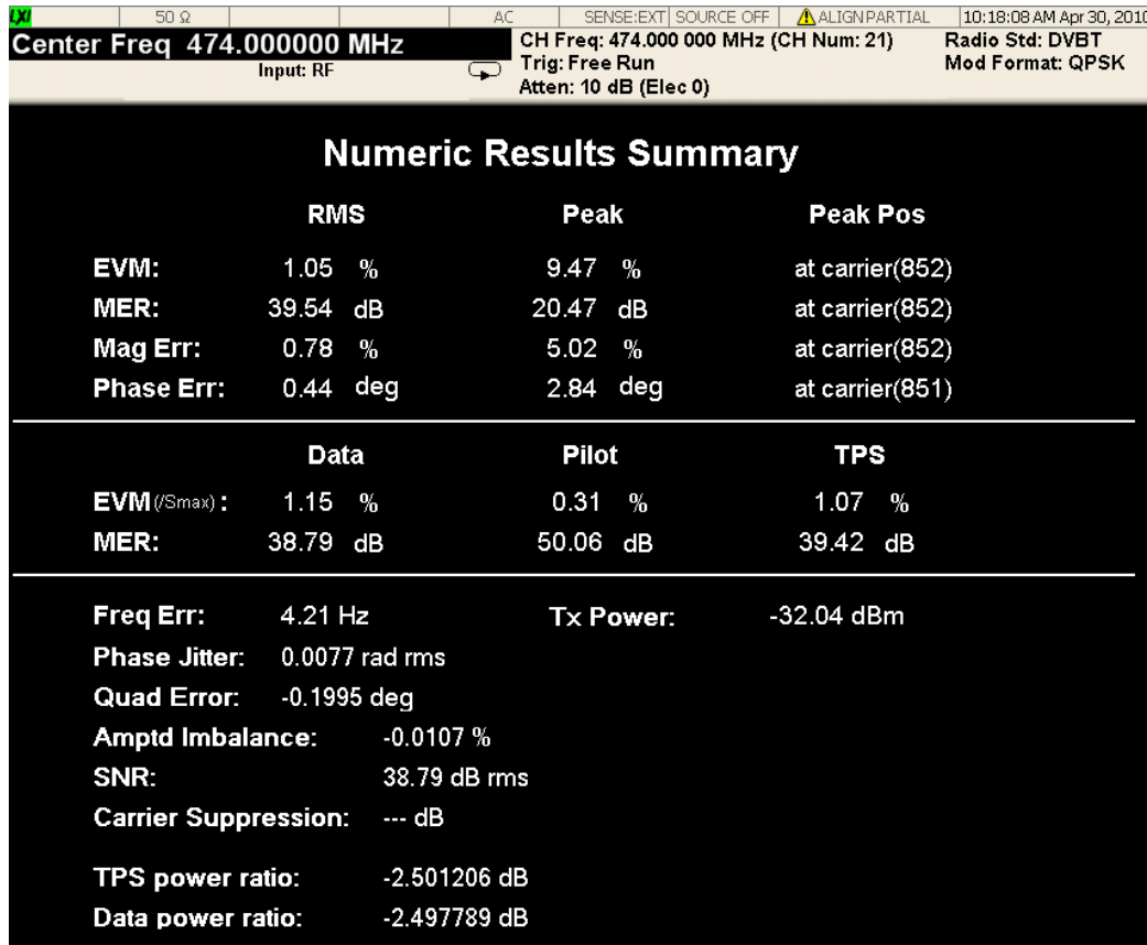
Figure 5 - 7 Result Metrics View of Modulation Accuracy Measurement
