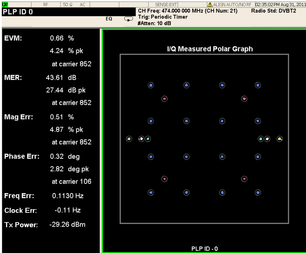
Rotated constellation
