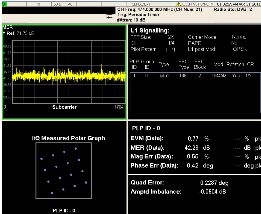
Figure 5 - 2 I/Q Error View of Modulation Accuracy Measurement
