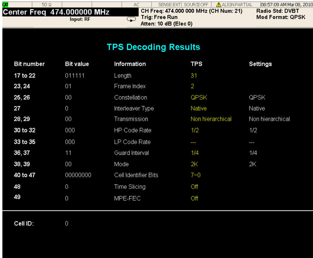
Figure 5 - 5 TPS Decoding View of Modulation Accuracy Measurement
