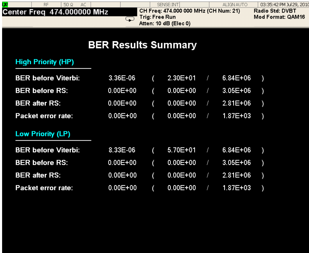
Figure 5 - 6 BER Results View of Modulation Accuracy Measurement
