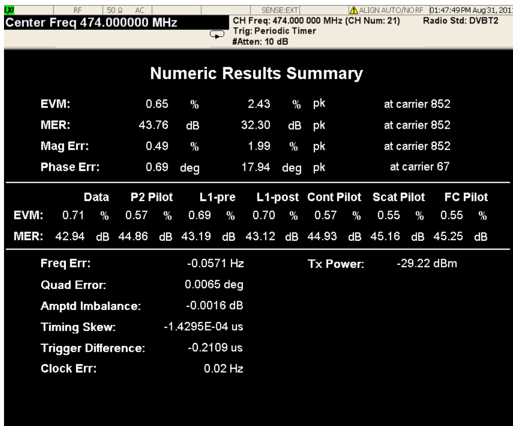
Figure 5 - 5 Result Metrics View of Modulation Accuracy Measurement
