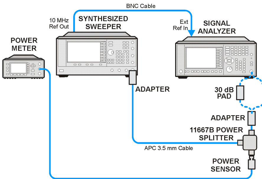
Figure 5-1. Amplitude Accuracy Test Setup
