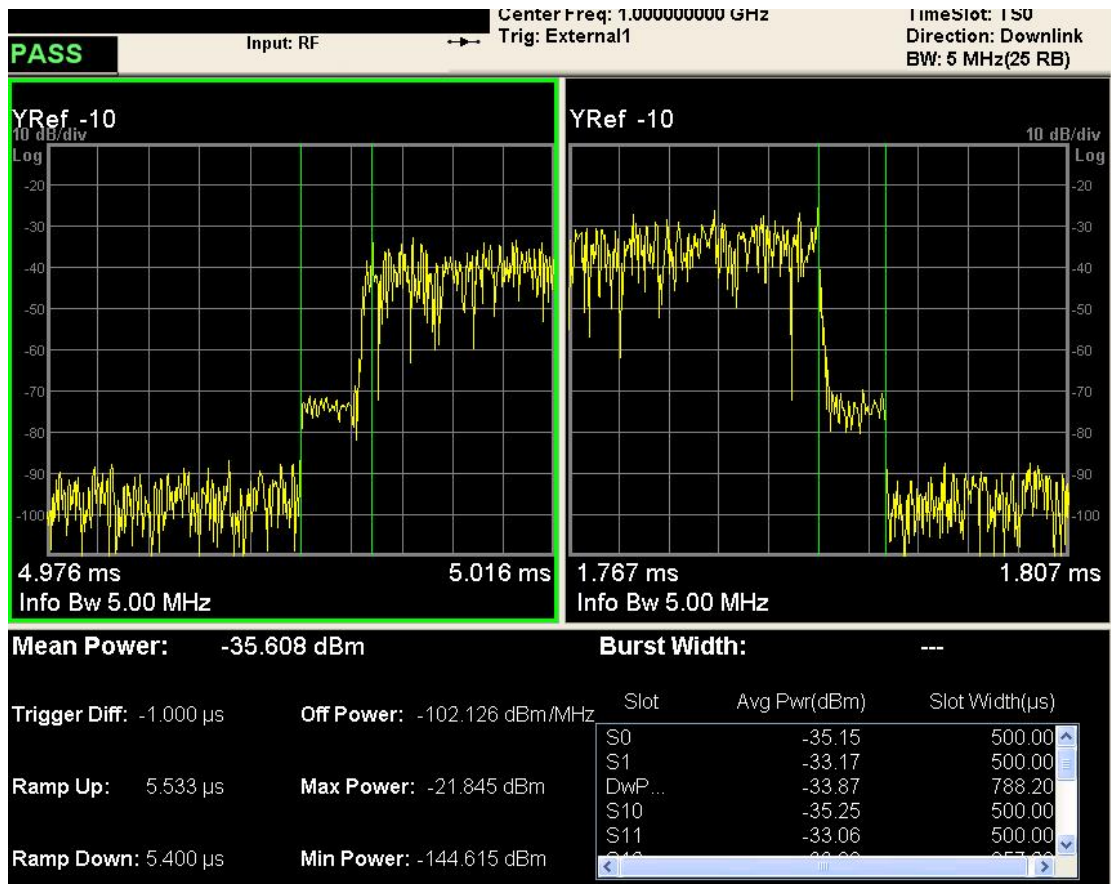
Figure 4-13 Rise & Fall View for LTE Power vs. Time Measurement
