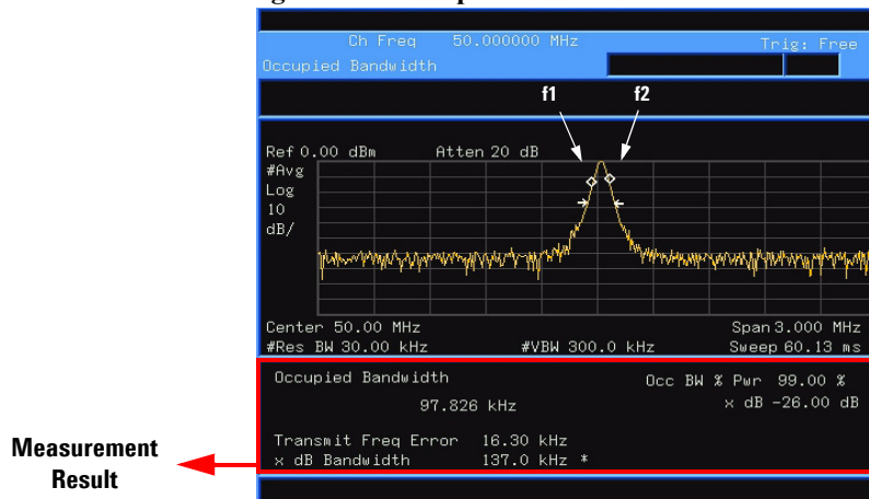
Figure 4-5 Occupied Bandwidth Measurement
