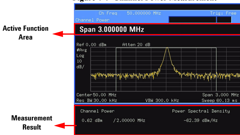
Figure 4-4 Channel Power Measurement
