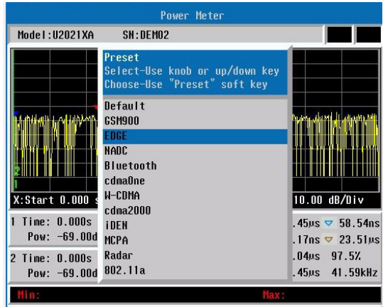
Figure 3-27 Customized Preset the U2020 Power Sensor
