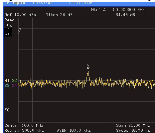
Figure 3-3 Delta Marker with Reference Signal Off-Screen
