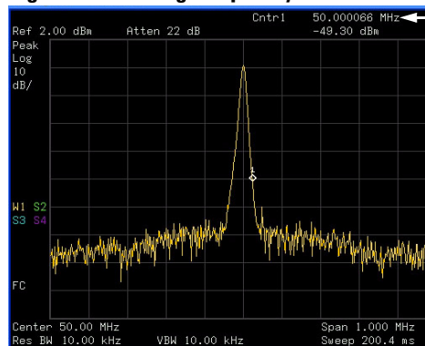
Figure 3-14 Using Frequency Counter
