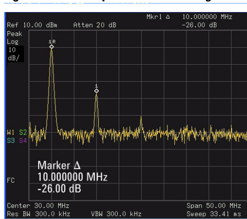
Figure 3-2 Delta pair marker with signals on the same screen
