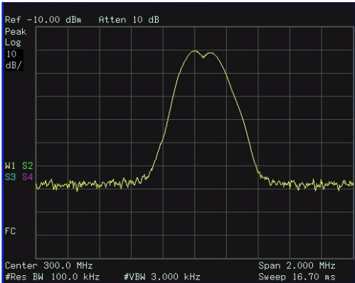
Figure 3-6 Resolving Signals of Equal Amplitude
