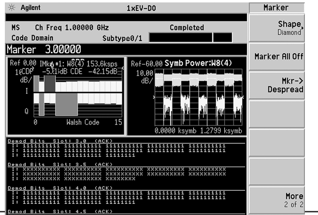
Figure 14. Demodulated bits view presents power-off half slots with X
