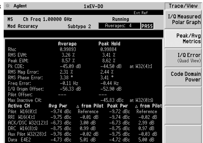
Figure 17. Mod Accuracy in Peak and Average result metrics view
