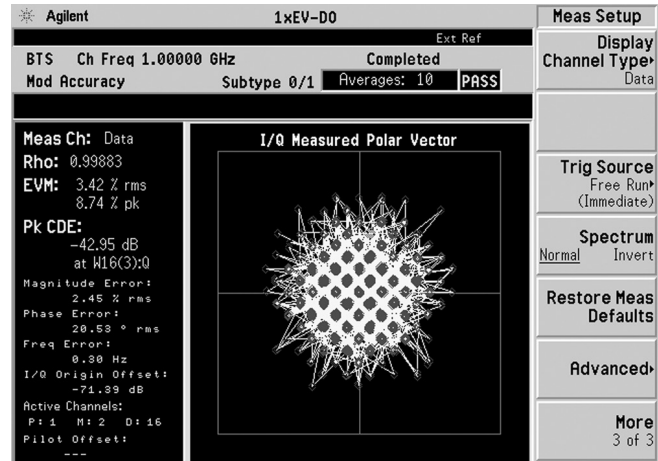
Figure 11. Modulation accuracy for data channel
