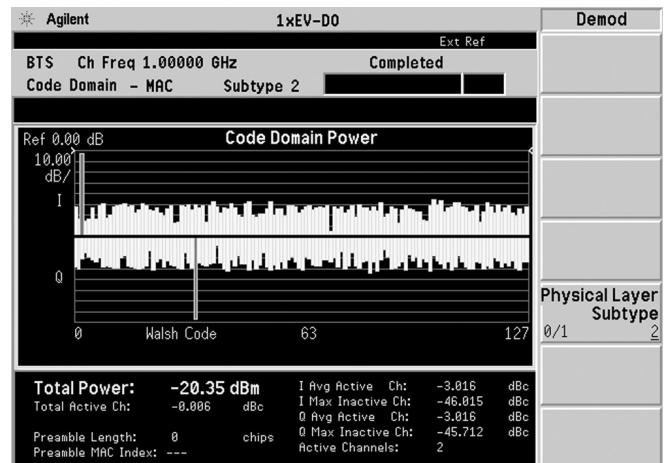
Figure 7. 1xEV-DO code domain for the MAC channel with subtype 2 (1xEV-DO rev. A)
