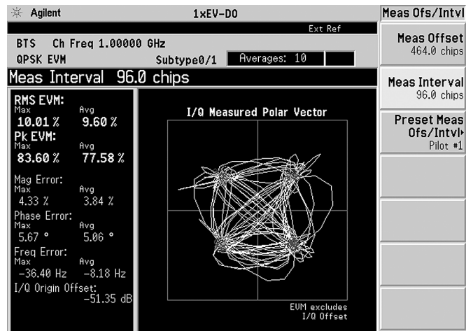
Figure 13. QPSK EVM for pilot
