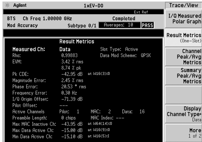
Figure 12. Numeric result summary of measured channel for one-slot
