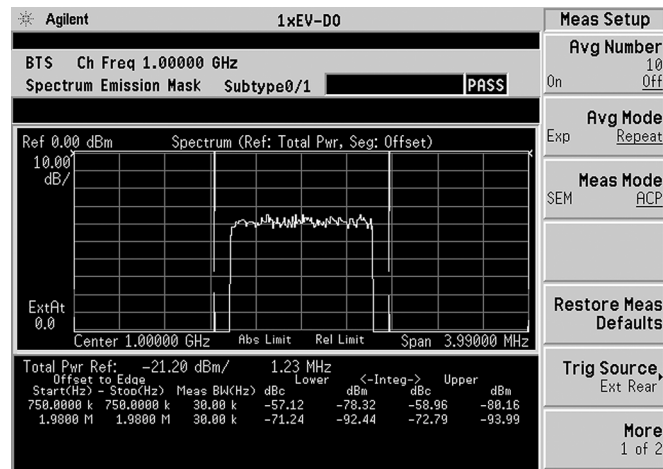
Figure 5. ACP measurement for idle slot
