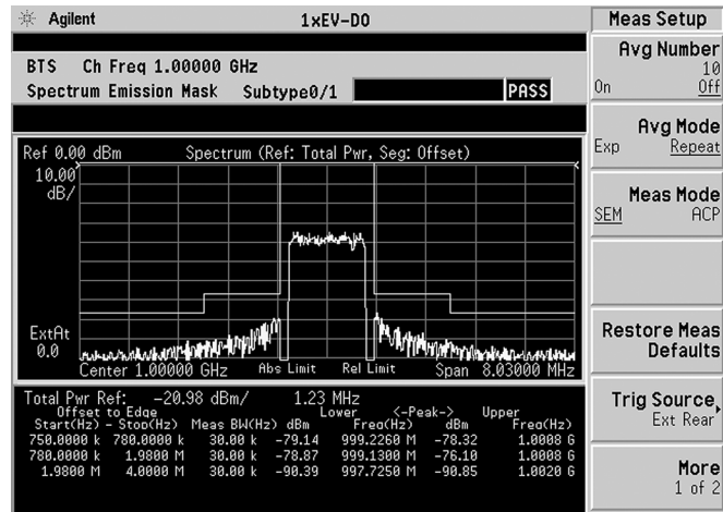
Figure 4. SEM (spectrum emission mask) measurement for idle slot
