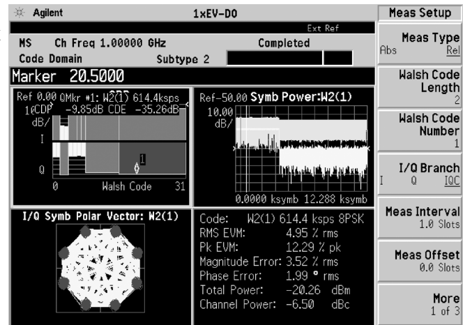
Figure 16. Code domain quad view with data in 8PSK constellation on IQ combined branch
