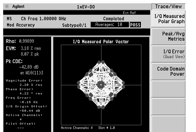
Figure 15. Modulation accuracy in I/Q polar graph view
