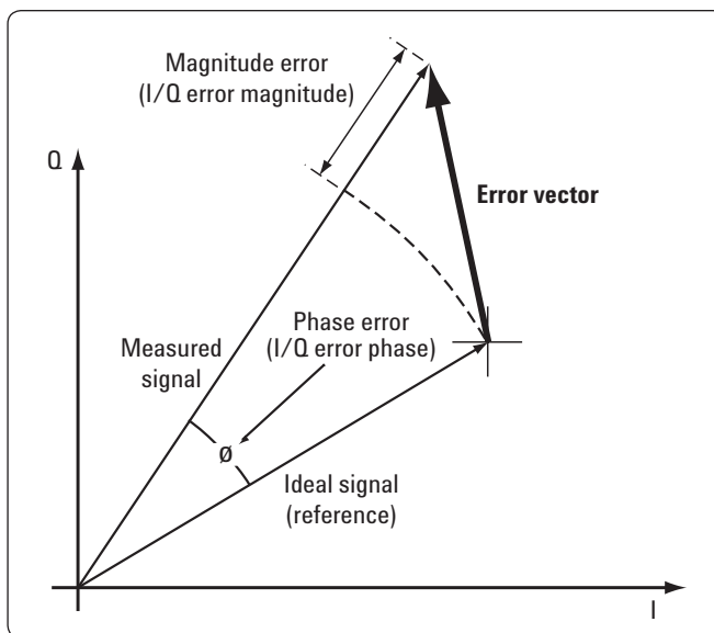
Figure 9. Error vector magnitude
