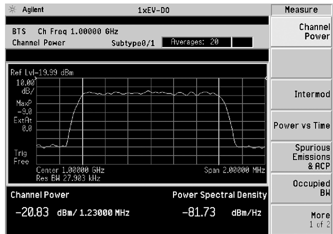
Figure 2. Channel power
