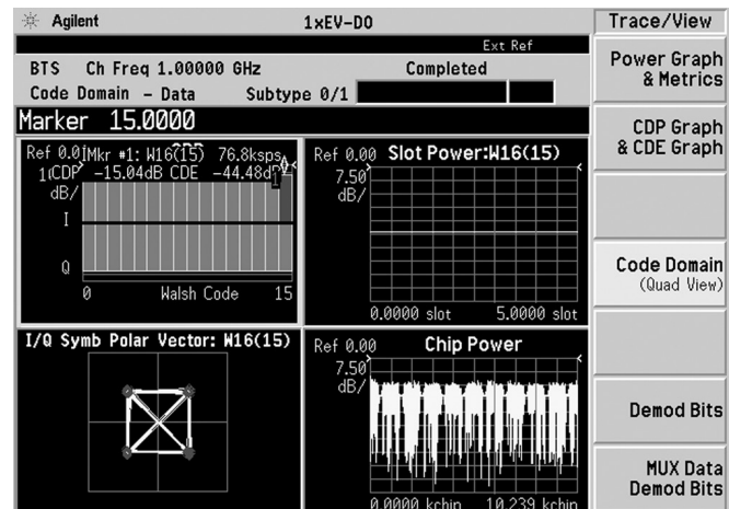
Figure 8. 1xEV-DO code domain for the DATA channel with subtype 1 (1xEV-DO rev. O)
