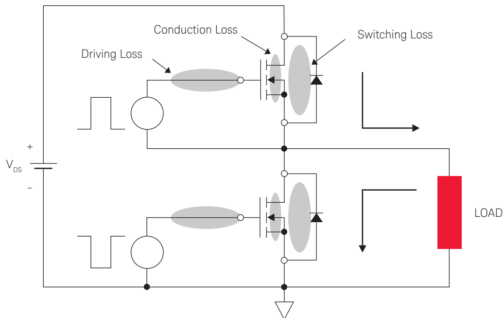
Figure 9.1. The components of power loss.
