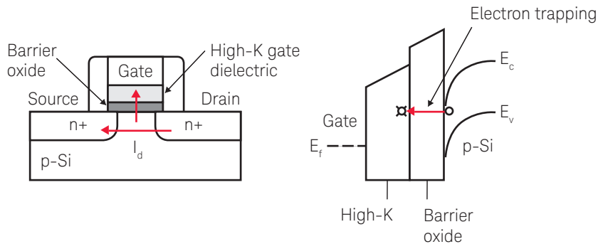
Figure 5.39. High-k gate dielectric MOSFETs are susceptible to electron trapping in the gate dielectric.
