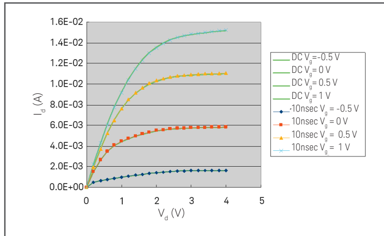
Figure 5.45. Comparisons of I_d - V_d measurements taken on a standard transistor using both the pulsed IV solution and SMUs shows excellent correlation.
