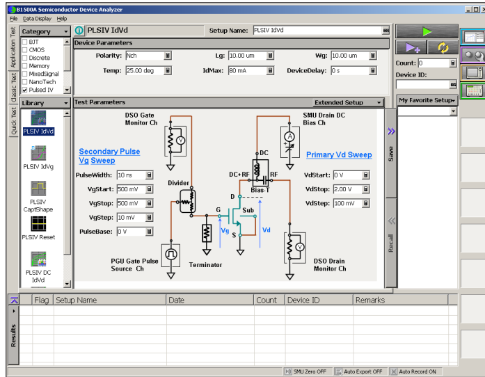
Figure 5.44. The B1542A 10 ns I_d - V_d application test.
