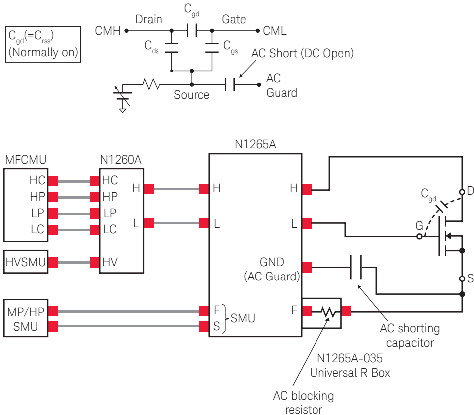
Figure 9.29. Measuring C_{gd} (=C_{rss}) on a normally on device using the N1260A Bias-T and the N1265A test fixture.
