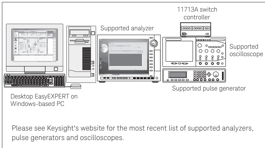
Figure 5.42. The B1542A 10 ns pulsed IV solution using an external PC running Desktop EasyEXPERT.
