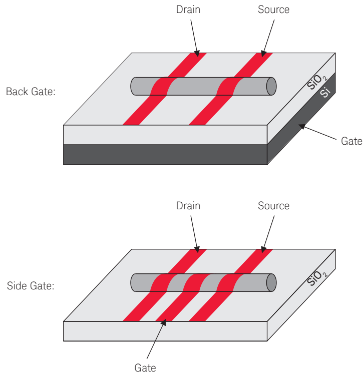
Figure 7.27. Illustration showing the two most common methods of creating a gate connection on a carbon nanotube transistor.
