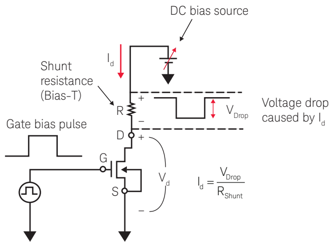
Figure 5.40. The basic circuit schematic outlining the operation of Keysight’s 10 ns pulsed IV measurement solution.
