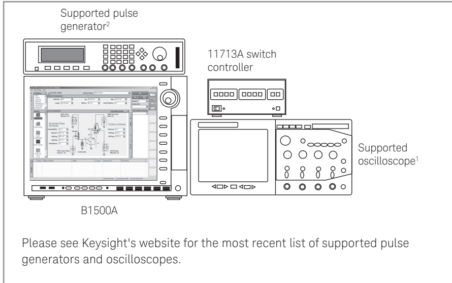
Figure 5.41. The B1542A 10 ns pulsed IV solution using the B1500A as the system controller.
