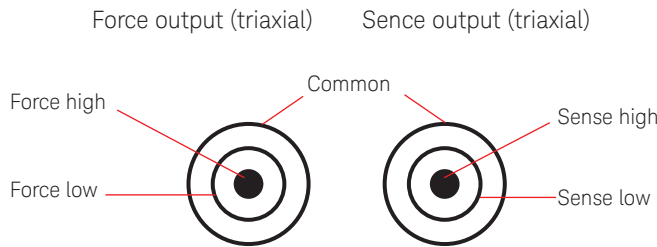
Figure 3.17 – The output configuration of the MCSMUs.
