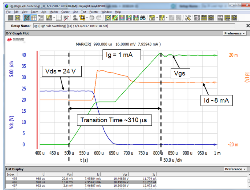
Figure 9.63. The high voltage switching waveforms for the MOSFET gate charge measurement with VdsOff = 24 V.
