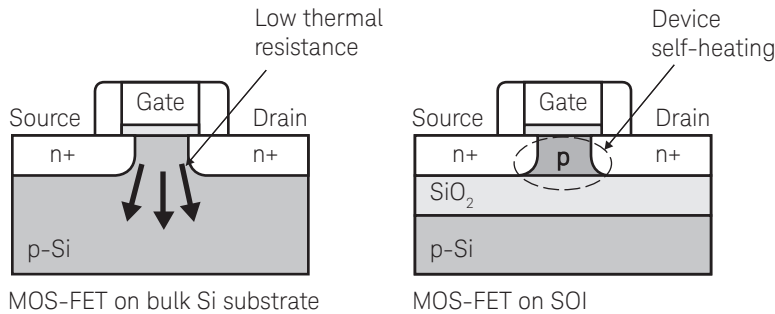
Figure 5.38. SOI based MOSFETs cannot easily dissipate the heat generated by continuous operation as can MOSFETs fabricated on bulk silicon.
