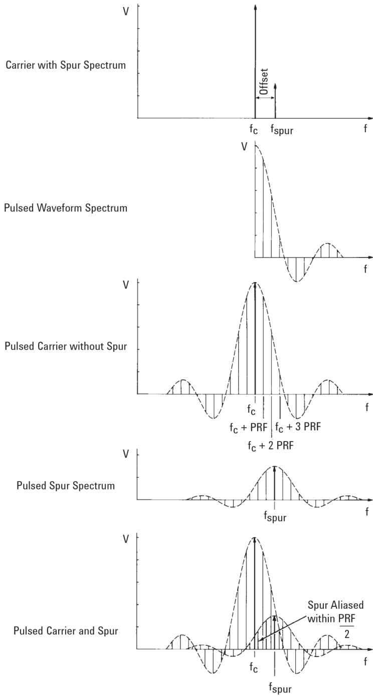
Figure 9. Convolution of a CW carrier with spur spectra and a pulsed waveform spectra
