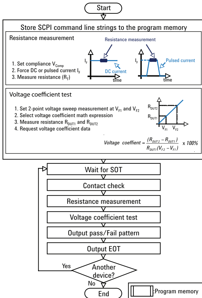
Figure 5. Resistor production test flow example using the B2900A Series of SMUs
