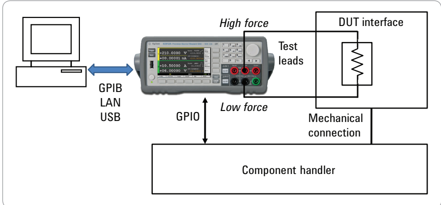
Figure 1. Example test system configuration using the B2900A Series of SMUs
