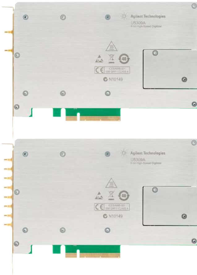
Figure 5. The Keysight 2 and 8 channels U5309A PCIe 8-bit digitizers with on-board processing offers a small size for easy integration.
