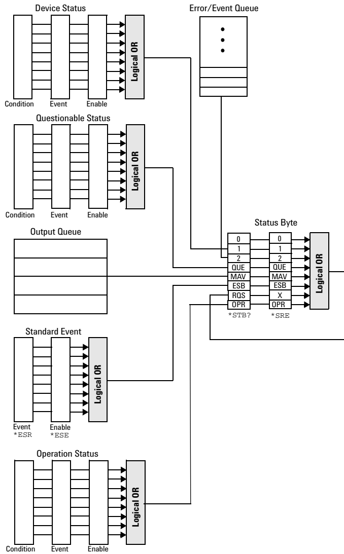
Figure 1-13 Status system
